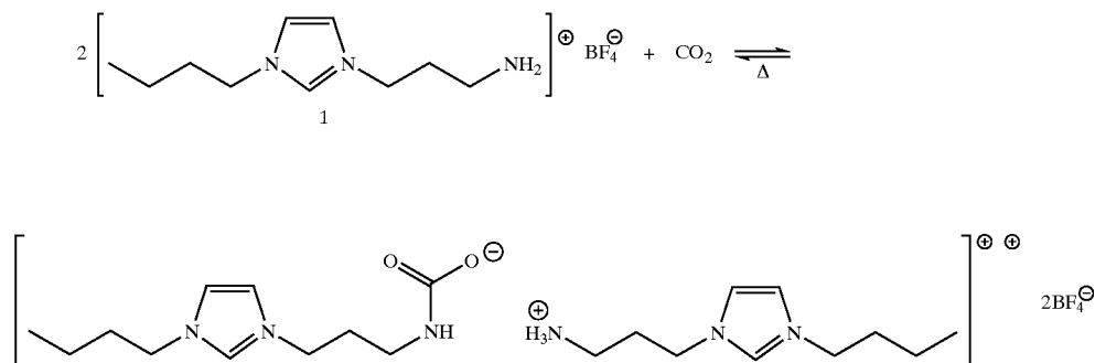
Scheme 2. Proposed reaction between TSIL 1 and CO 2 .
