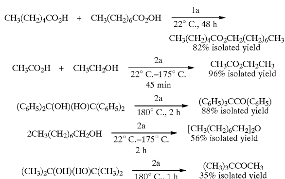
Scheme 1. Representative reactions using IL 1a and 2a.
