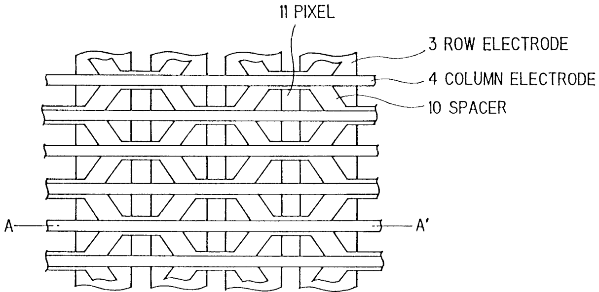
FIG.1 PRIOR ART
