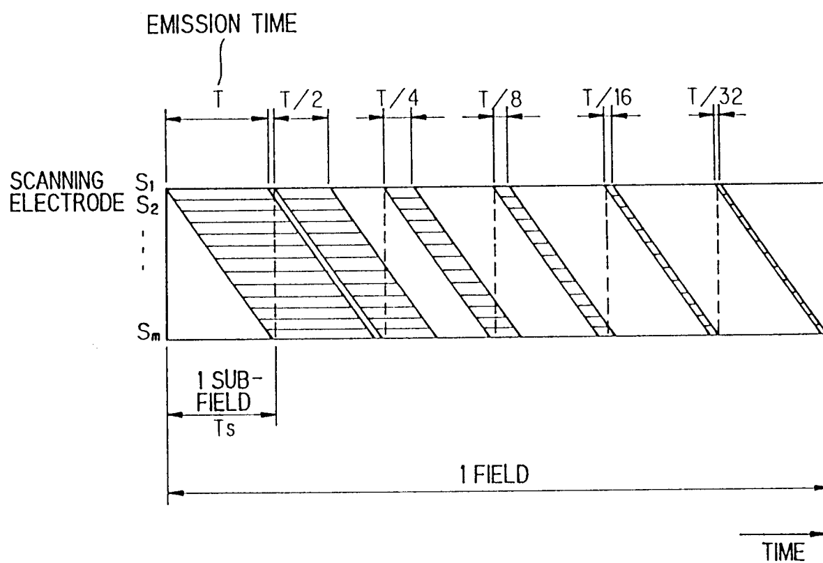
FIG.5 PRIOR ART
