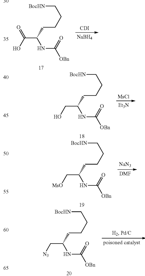
Scheme 3.
