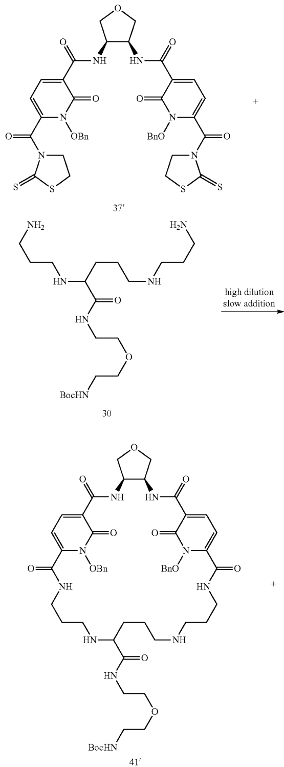
Scheme 15.
