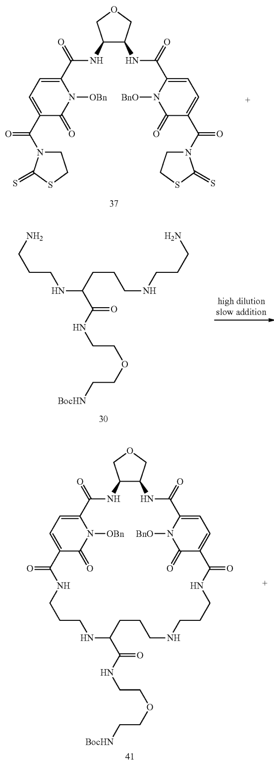
Scheme 7.
