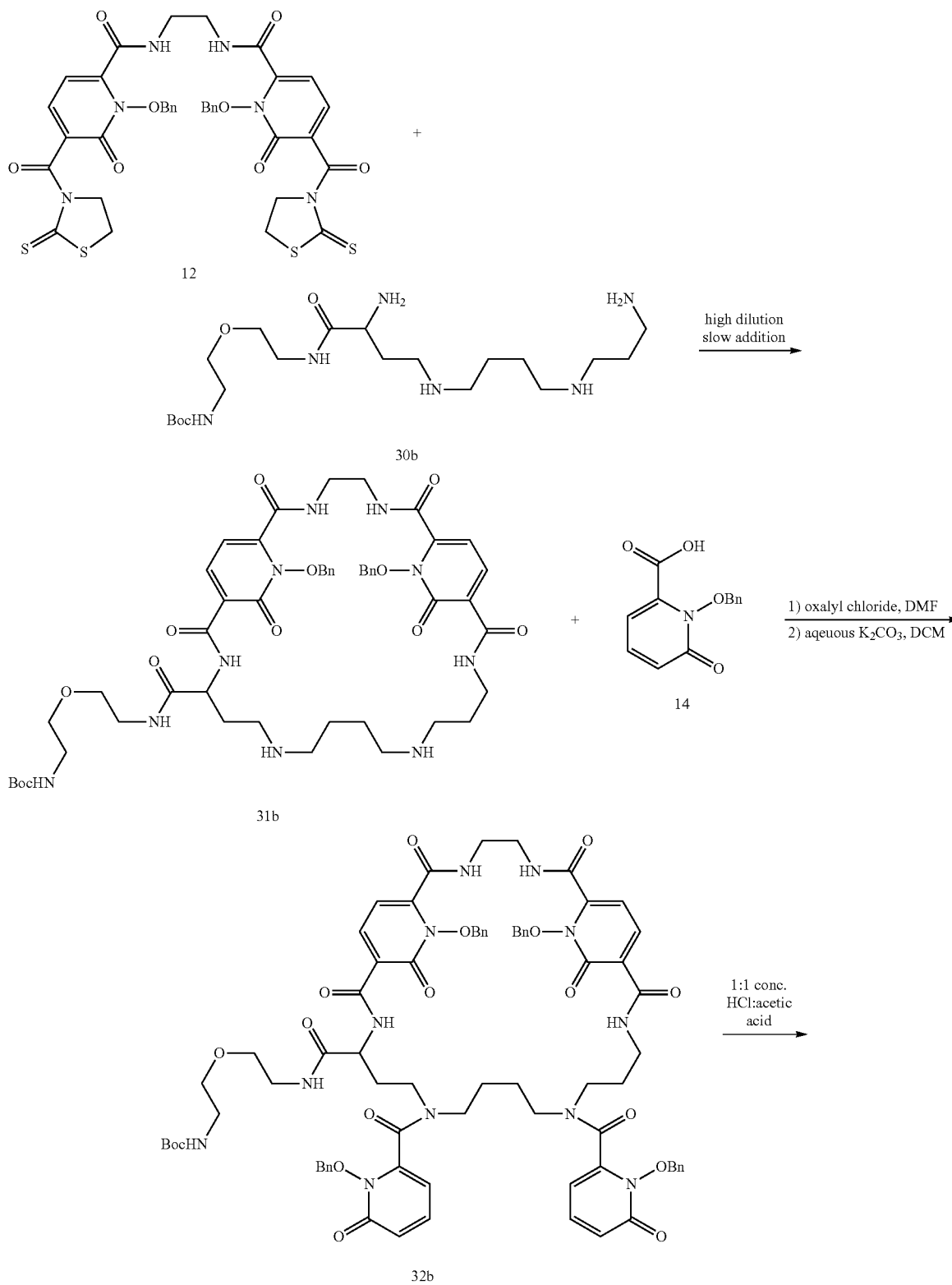
Scheme 8.
