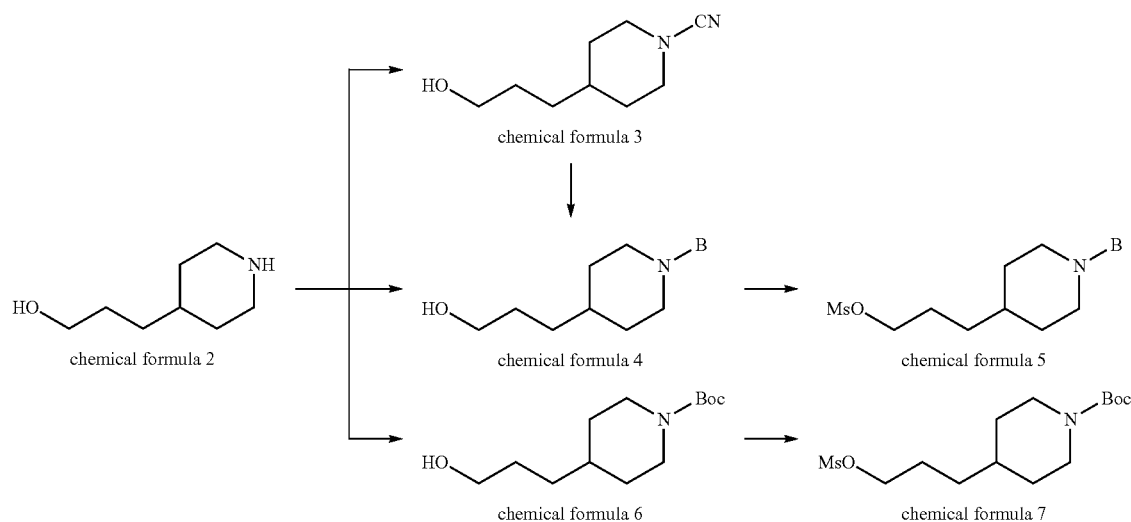
[Reaction Formula 2]
