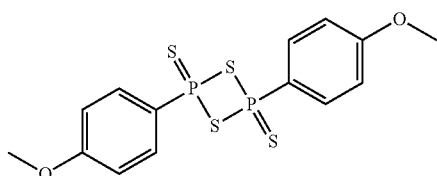
[Chemical Formula 21]
