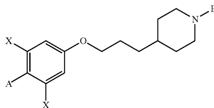
[Chemical Formula 2]
