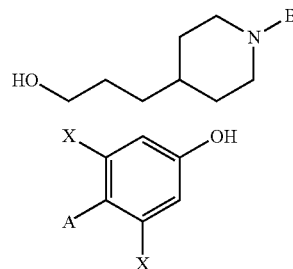
[Chemical Formula 12]
