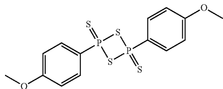
[Chemical Formula 21]
