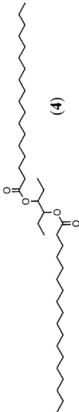
Octadecanoic acid 1-ethyl-2-octadecanoyloxy-butyl ester
