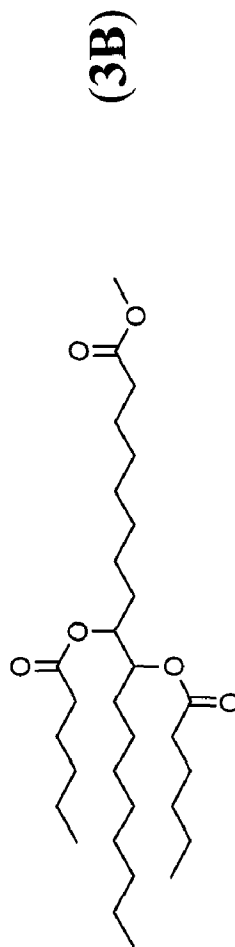
9,10-Bis-hexanoyloxy-octadecanoic acid methyl ester
