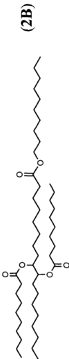
9,10-Bis-decanoyloxy-octadecanoic acid decyl ester
