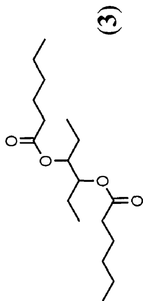
Hexanoic acid 1-ethyl-2-hexanoyloxy-butyl ester
