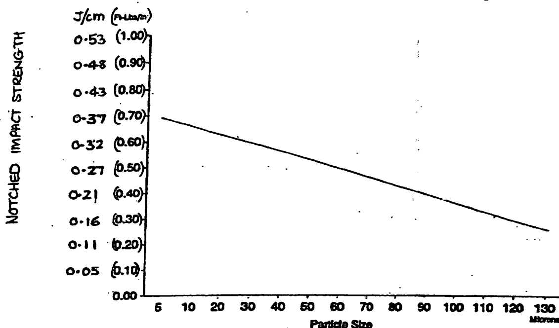
Particle Size v. IZOD Notched Impact Strength
