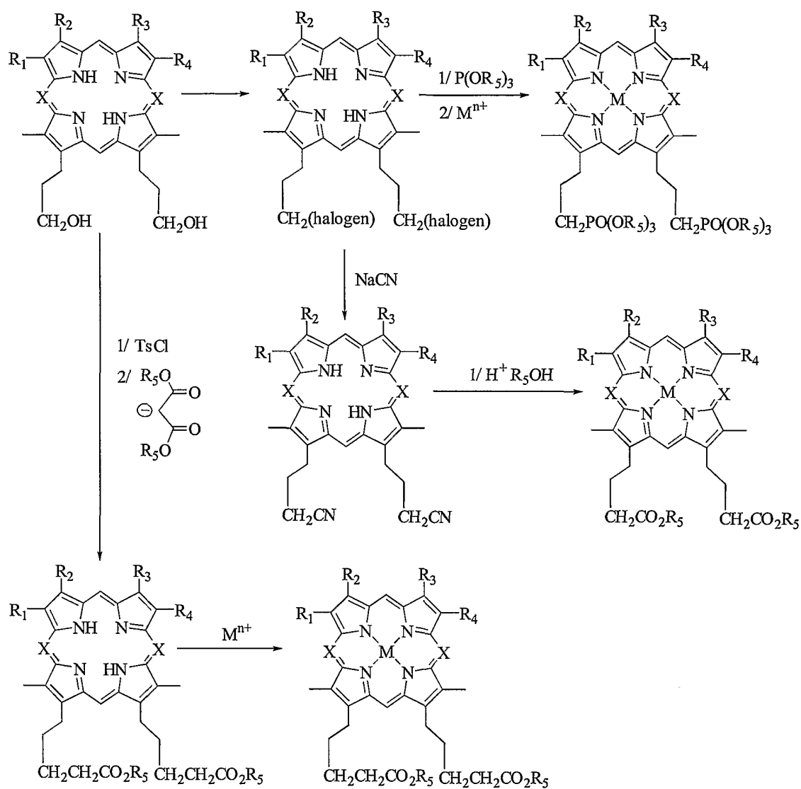
Scheme 6. Modification of Porphyrin (X=CR) and azaporphyrin (X=N) compounds
