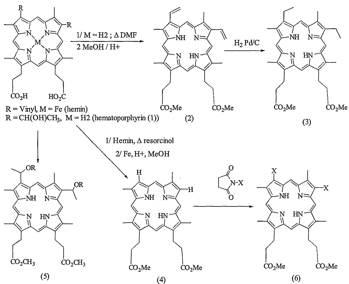
Scheme 1. Blood Derived Porphyrins
