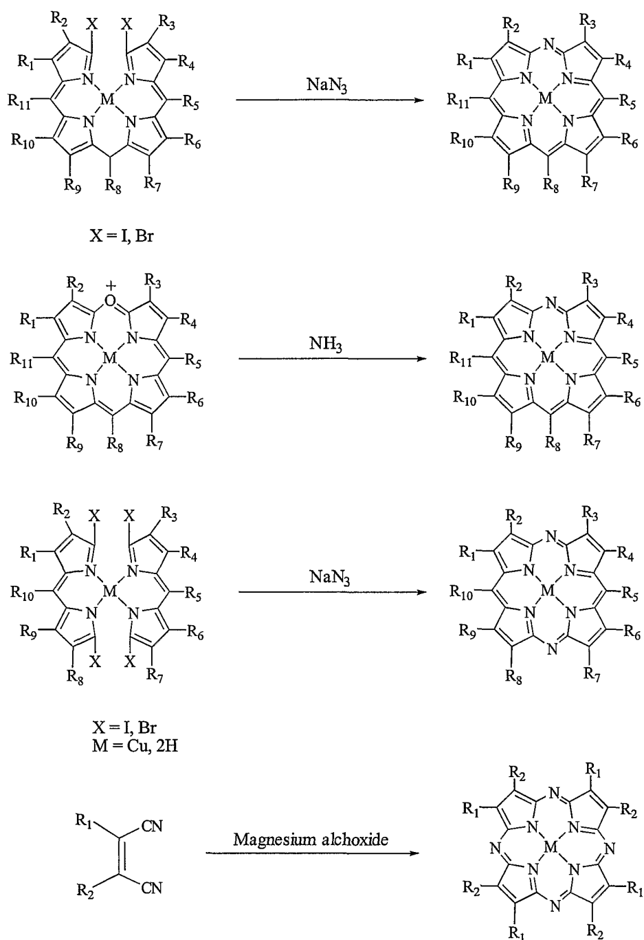
Scheme 3. Azaporphyrin Syntheses
