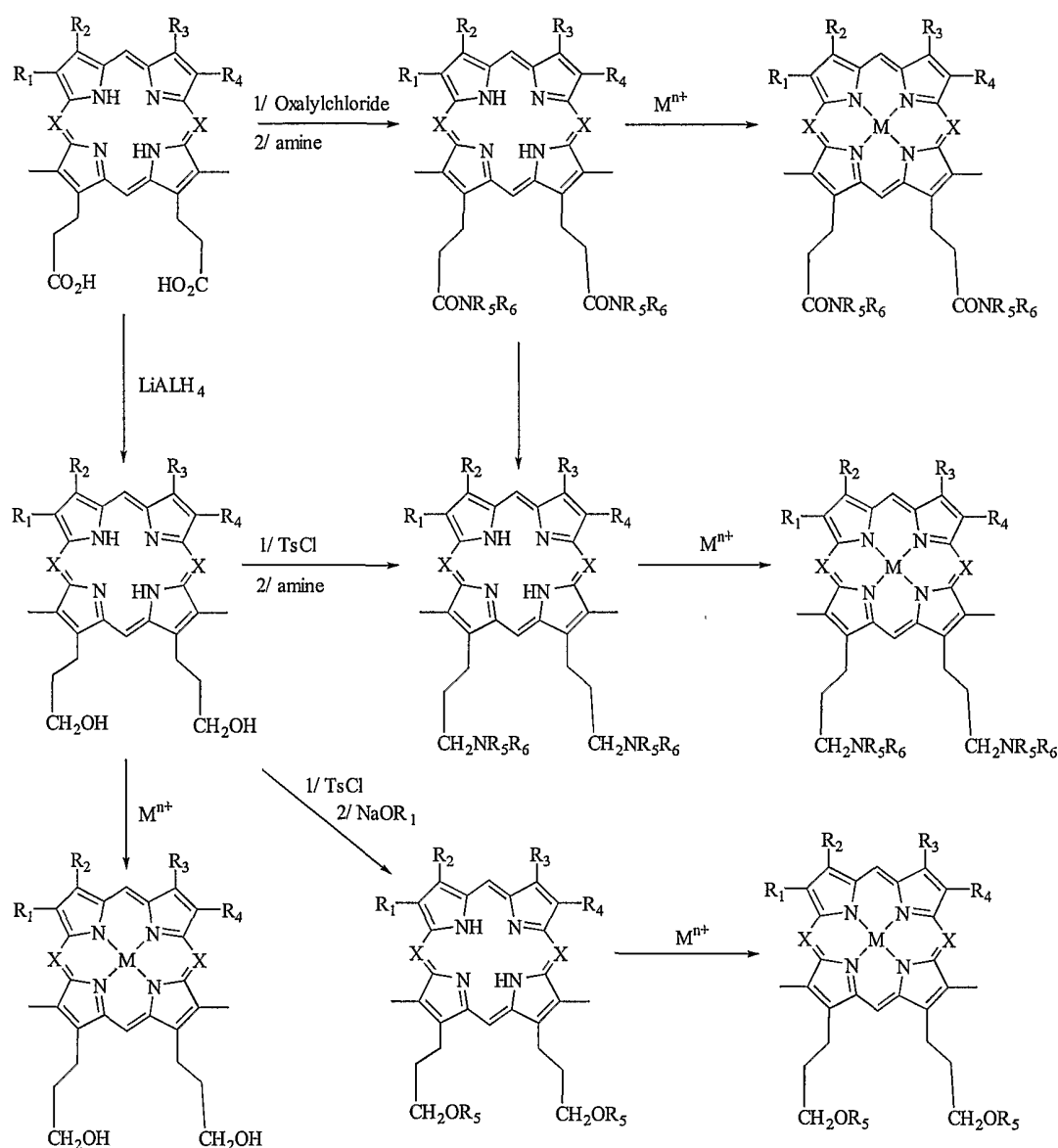
Scheme 7. Modification of Porphyrin ( \text{X}=\text{CR} ) and diazaporphyrin ( \text{X}=\text{N} ) compounds
