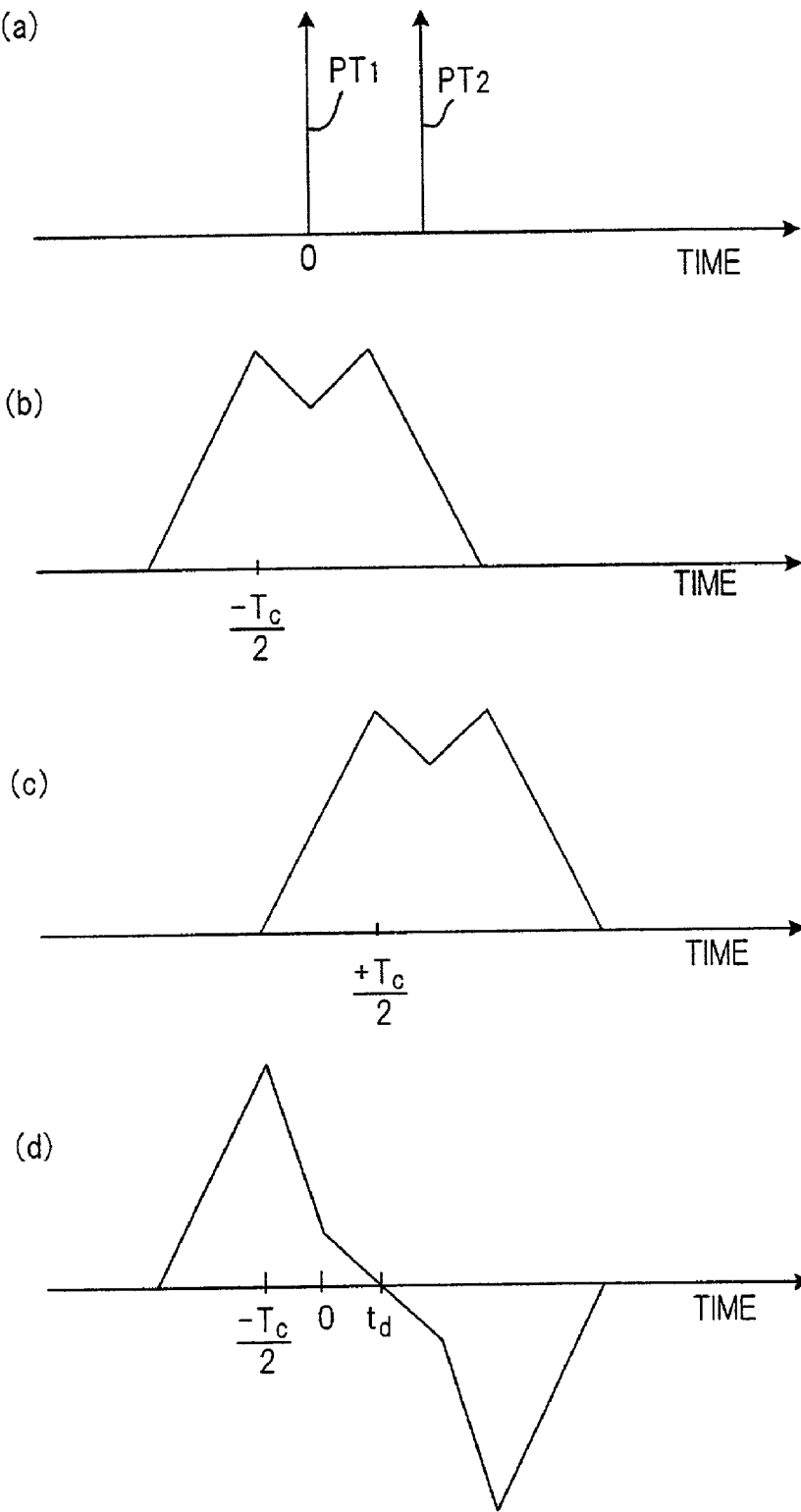
FIG. 19 PRIOR ART
