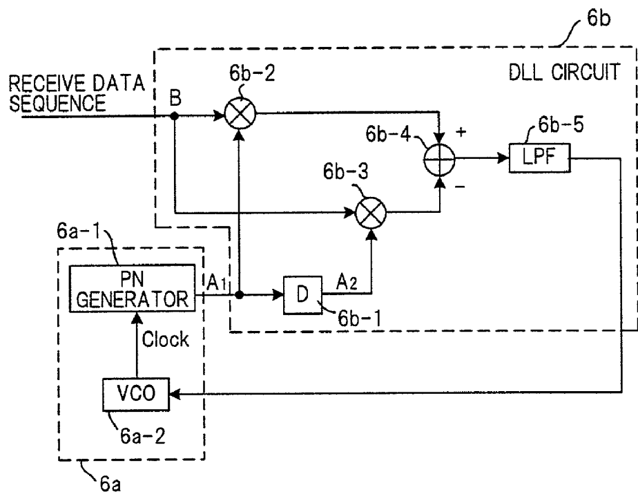
FIG. 13 PRIOR ART
