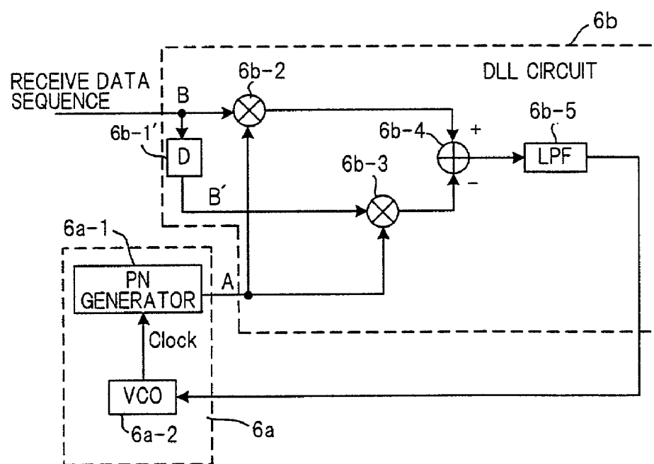
FIG. 14 PRIOR ART
