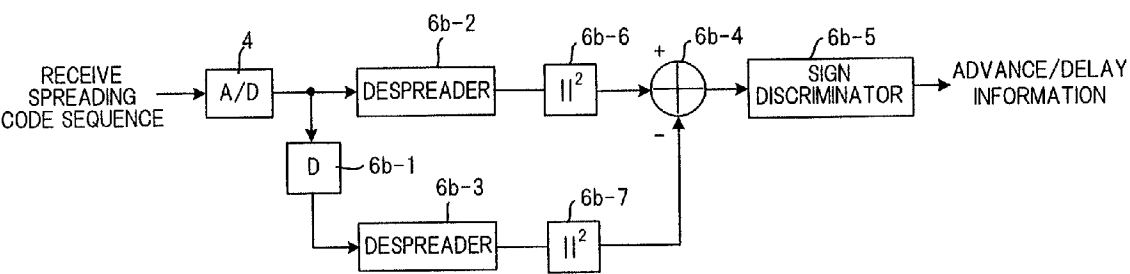
FIG. 17 PRIOR ART
