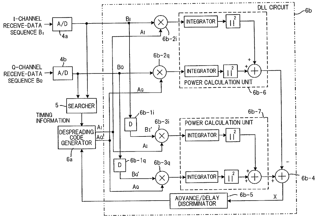
FIG. 16 PRIOR ART
