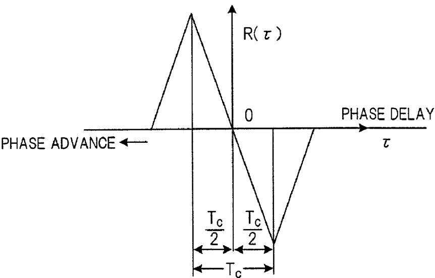
FIG. 15C PRIOR ART
