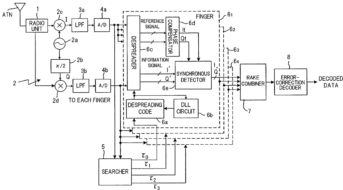
FIG. 12 PRIOR ART
