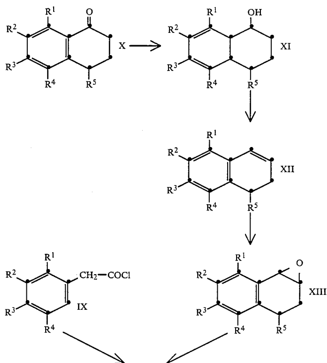
Reaction Scheme
