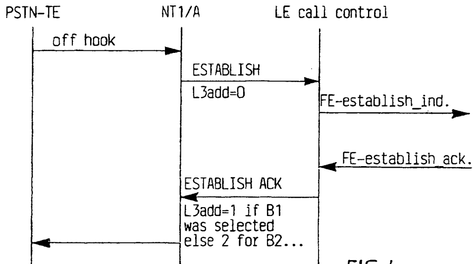
FIG. 4 ORIGINATING CALL INITIATE
