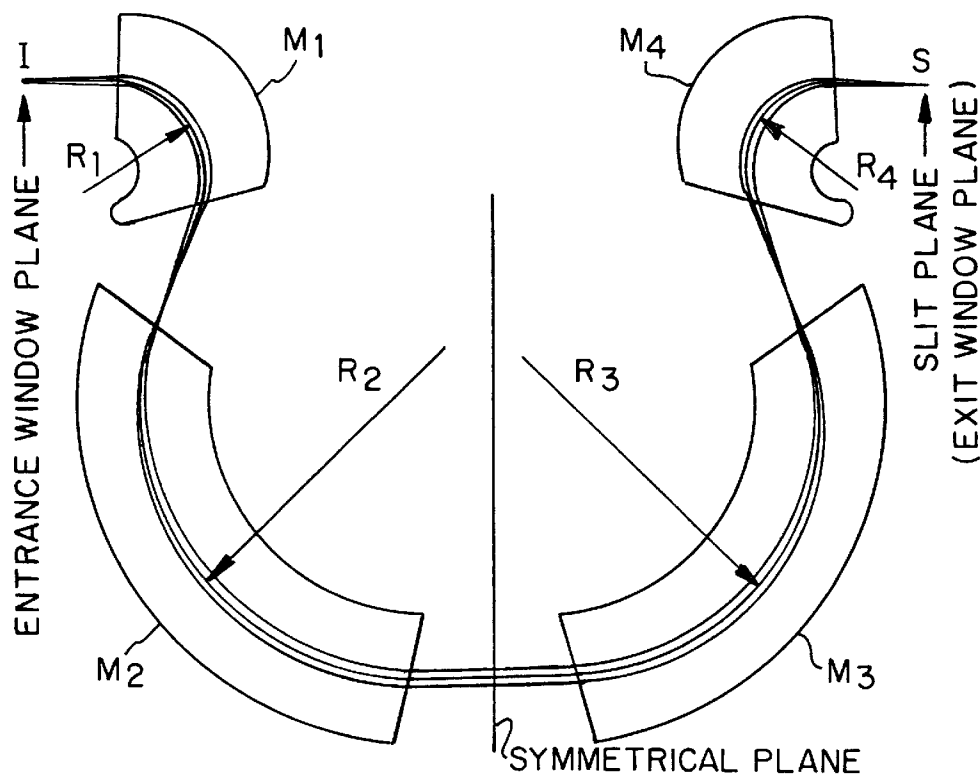
FIG. 3 PRIOR ART
