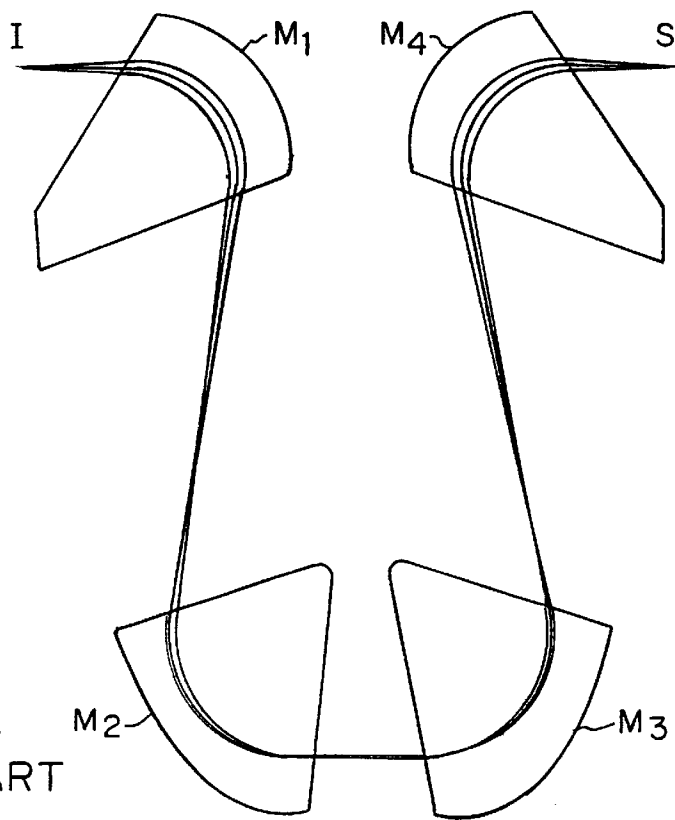
FIG. 3 PRIOR ART
