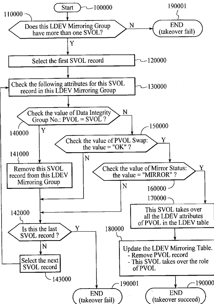
Process of PVOL takeover in LDEV Mirroring Group
