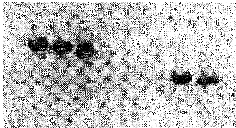
32 P-Immobilized Substrate
