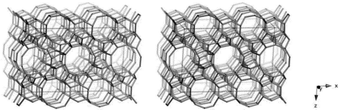
Topology of [010] face
