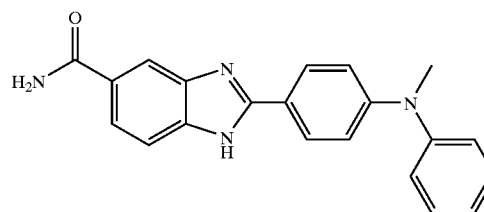
2-[4-(Methyl-phenyl-amino)-phenyl]-1H-benzimidazole-5-carboxylic acid amide
