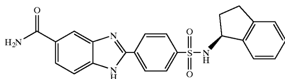
2-[4-((S)-Indan-1-ylsulfamoyl)-phenyl]-1H-benzoimidazole-5-carboxylic acid amide
