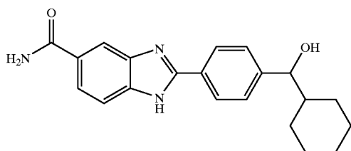
2-[4-(Cyclohexyl-hydroxy-methyl)-phenyl]-1H-benzoimidazole-5-carboxylic acid amide
