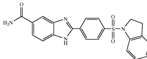
2-[4-(2,3-Dihydro-indole-1-sulfonyl)-phenyl]-1H-benzimidazole-5-carboxylic acid amide
