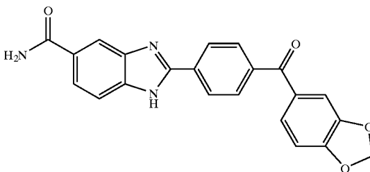
2-[4-(Benzo[1,3]dioxole-5-carbonyl)-phenyl]-1H-benzimidazole-5-carboxylic acid amide
