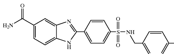
2-[4-(4-Methyl-benzylsulfamoyl)-phenyl]-1H-benzimidazole-5-carboxylic acid amide
