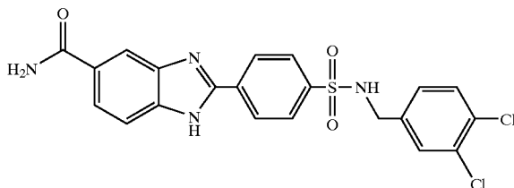
2-[4-(3,4-Dichloro-benzylsulfamoyl)-phenyl]-1H-benzimidazole-5-carboxylic acid amide
