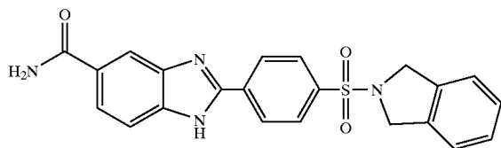
2-[4-(1,3-Dihydro-indole-2-sulfonyl)-phenyl]-1H-benzimidazole-5-carboxylic acid amide
