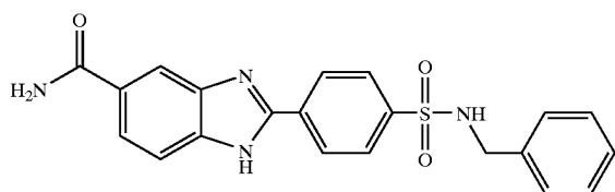
2-(4-Benzylsulfamoyl-phenyl)-1H-benzimidazole-5-carboxylic acid amide
