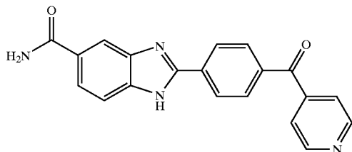
2-[4-(Pyridine-4-carbonyl)-phenyl]-1H-benzimidazole-5-carboxylic acid amide
