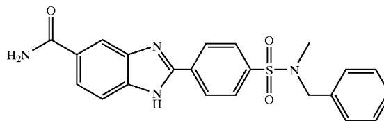
2-[4-(Benzyl-methyl-sulfamoyl)-phenyl]-1H-benzimidazole-5-carboxylic acid amide
