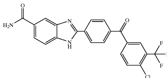
2-[4-(4-Chloro-3-trifluoromethyl-benzoyl)-phenyl]-1H-benzimidazole-5-carboxylic acid amide
