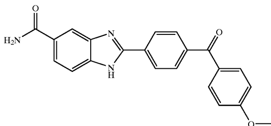
2-[4-(4-Methoxy-benzoyl)-phenyl]-1H-benzimidazole-5-carboxylic acid amide
