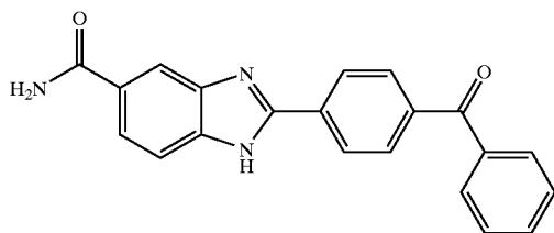
2-(4-Benzoyl-phenyl)-1H-benzimidazole-5-carboxylic acid amide
