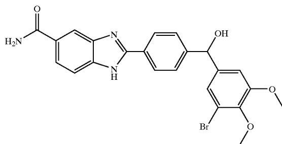
2-{4-[(3-Bromo-4,5-dimethoxy-phenyl)-hydroxy-methyl]-phenyl}-1H-benzimidazole-5-carboxylic acid amide
