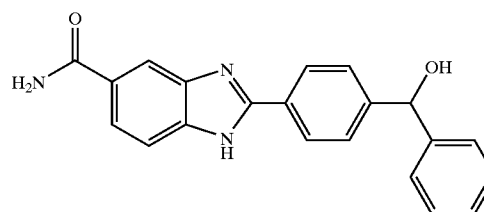
2-[4-(Hydroxy-phenyl-methyl)-phenyl]-1H-benzimidazole-5-carboxylic acid amide
