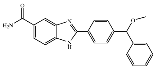
2-[4-(Methoxy-phenyl-methyl)-phenyl]-1H-benzoimidazole-5-carboxylic acid amide
