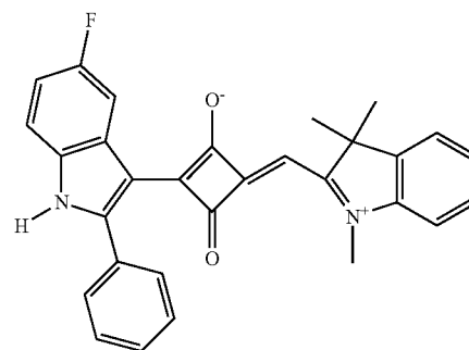
Compound No. 34
