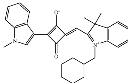
Compound No. 55
