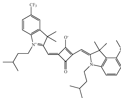
Compound No. 214
