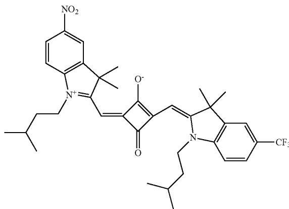
Compound No. 212
