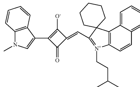
Compound No. 56
