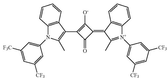
Compound No. 101
