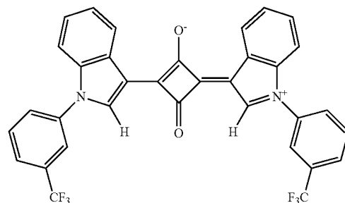
Compound No. 117
