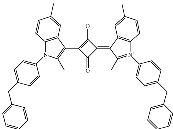
Compound No. 120
