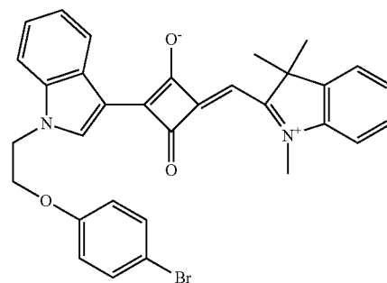
Compound No. 46
