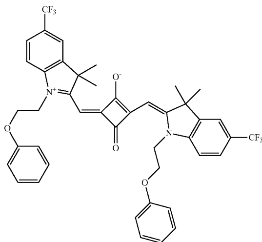
Compound No. 224
