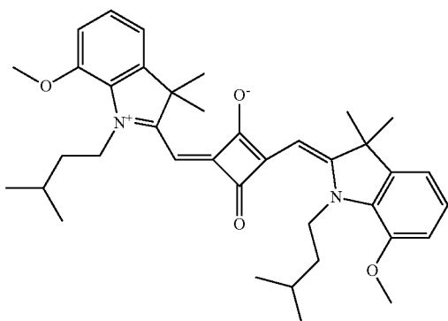
Compound No. 221
