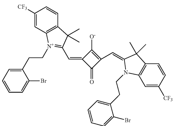
Compound No. 229
