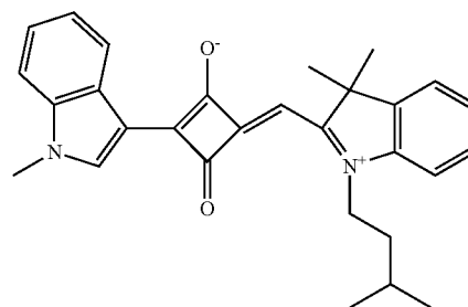
Compound No. 5
