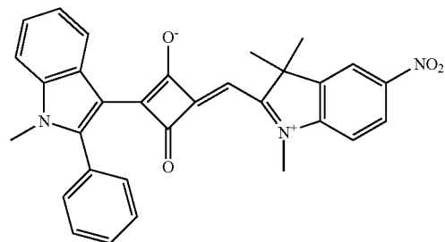
Compound No. 33
