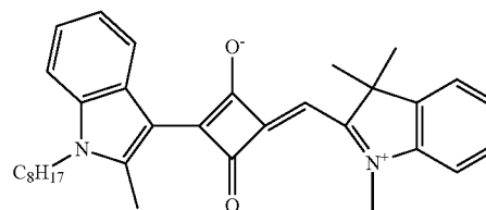
Compound No. 45
