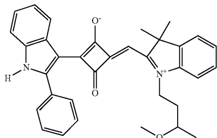
Compound No. 39
