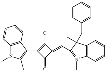
Compound No. 19
