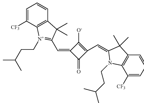
Compound No. 220
