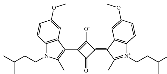
Compound No. 124
