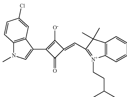
Compound No. 66
