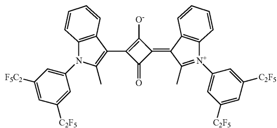
Compound No. 112
