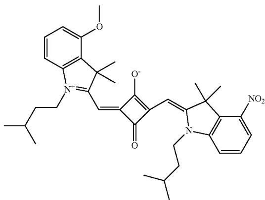
Compound No. 216
