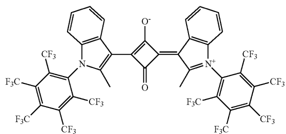
Compound No. 113
