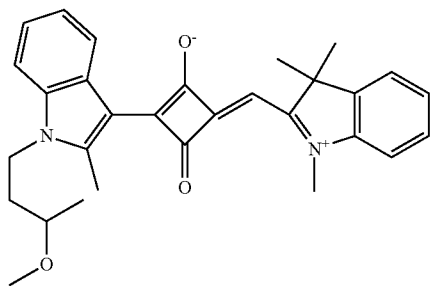
Compound No. 47
