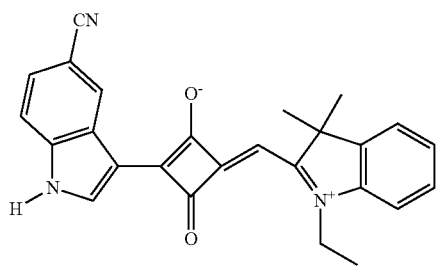
Compound No. 10
