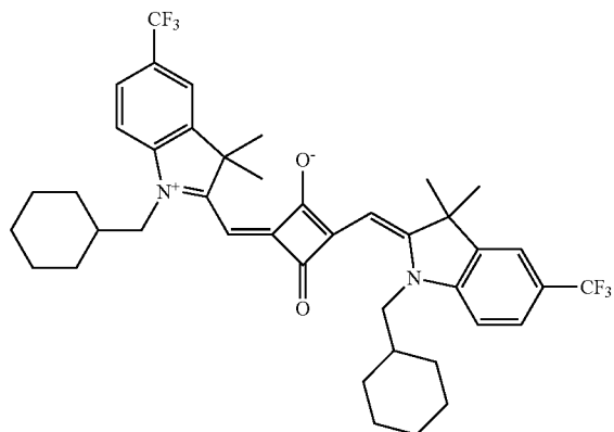
Compound No. 225
