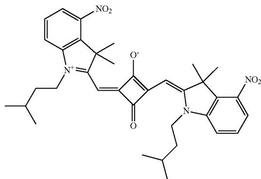
Compound No. 202
