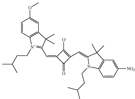
Compound No. 218
