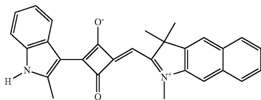
Compound No. 41
