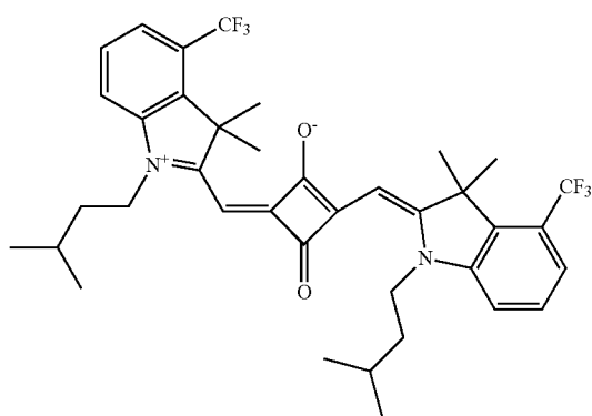
Compound No. 204
