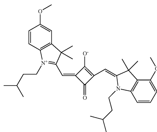
Compound No. 208
