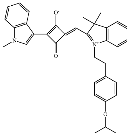
Compound No. 70
