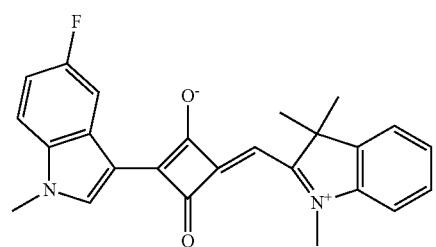
Compound No. 12
