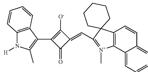
Compound No. 17
