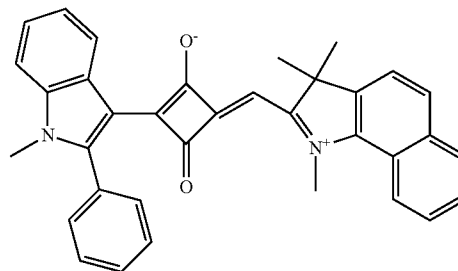
Compound No. 43
