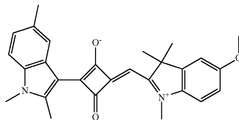
Compound No. 24
