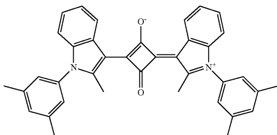
Compound No. 103
