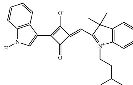
Compound No. 54
