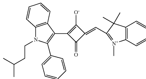
Compound No. 28
