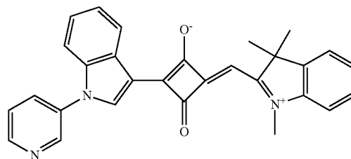
Compound No. 52
