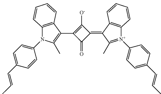
Compound No. 121
