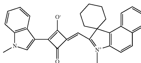
Compound No. 4
