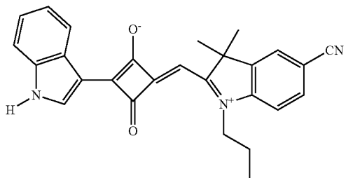
Compound No. 8
