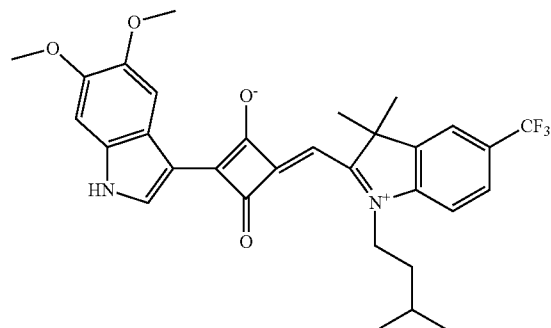
Compound No. 72
