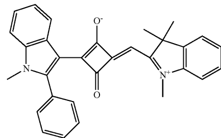
Compound No. 26
