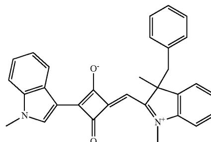
Compound No. 7
