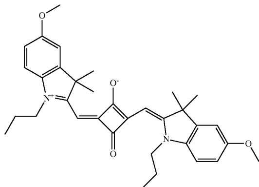
Compound No. 209
