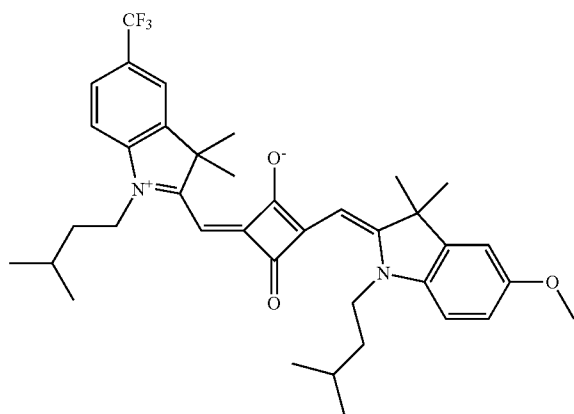
Compound No. 215
