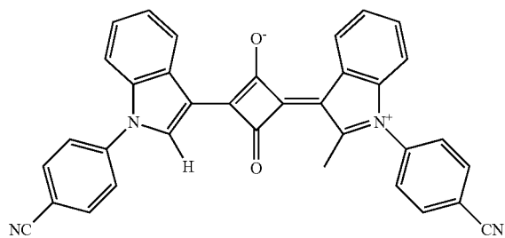
Compound No. 118
