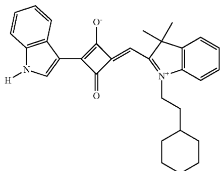
Compound No. 37
