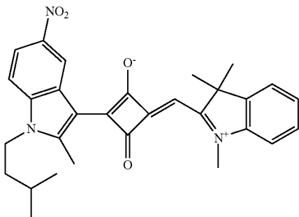
Compound No. 23
