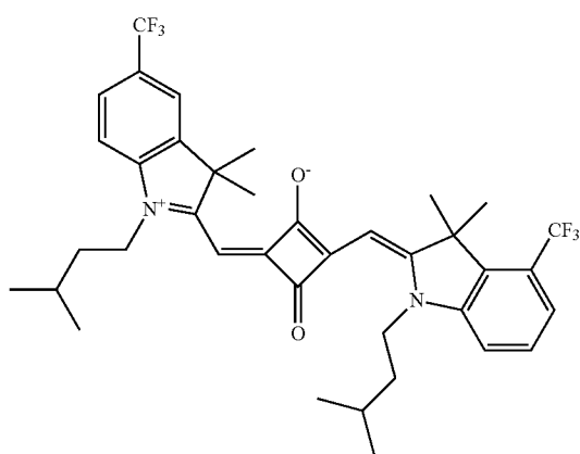
Compound No. 205
