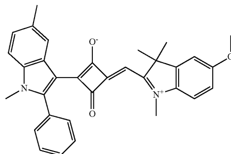
Compound No. 36
