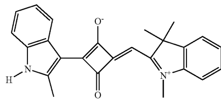
Compound No. 14
