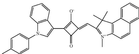
Compound No. 51
