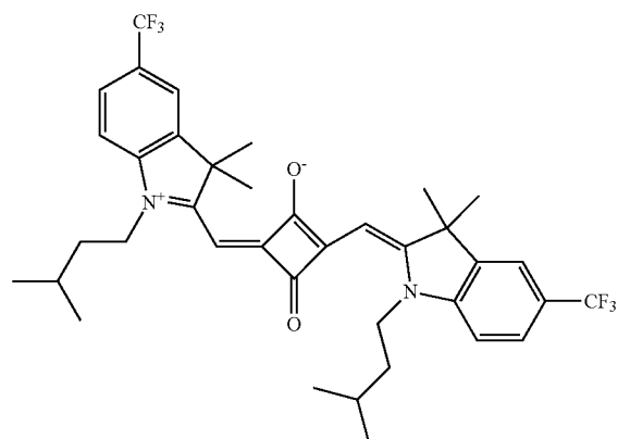
Compound No. 206
