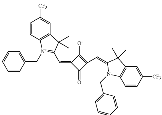
Compound No. 223
