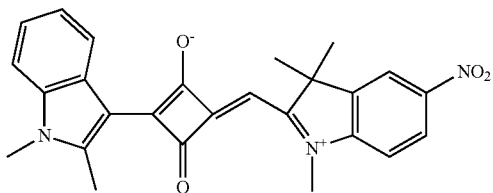
Compound No. 21
