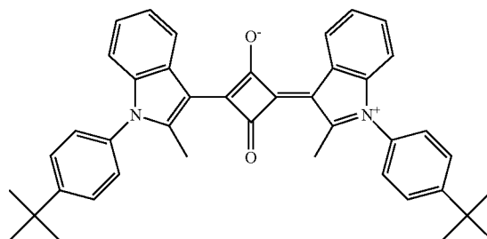
Compound No. 105
