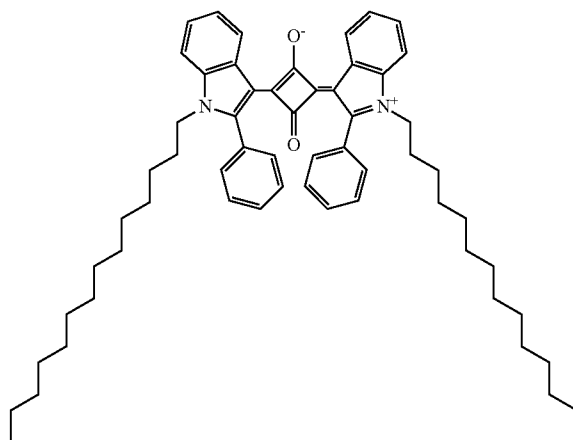
Compound No. 124
