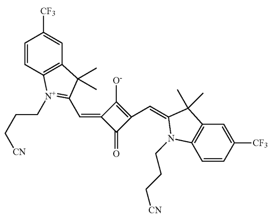
Compound No. 232
