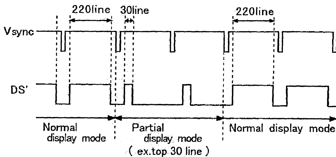
FIG.2B Waveform diagram of vertical scanning
