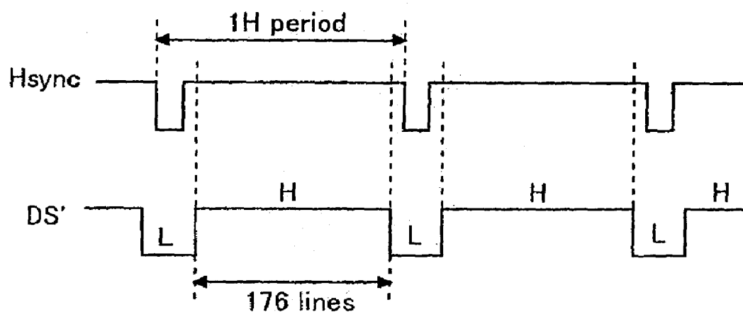
FIG.2A Waveform diagram of horizontal scanning
