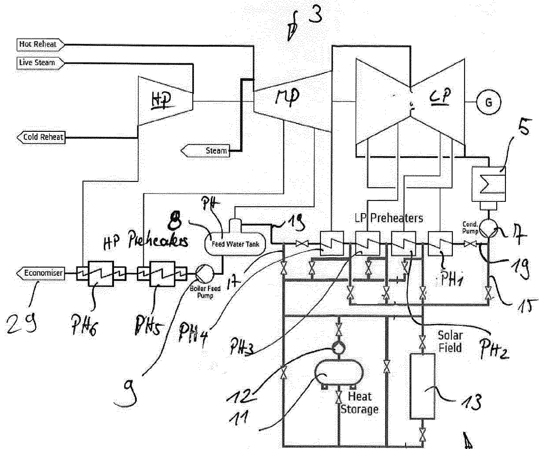
Figure 1: Low Pressure Direct Integration - Simplified Diagram
