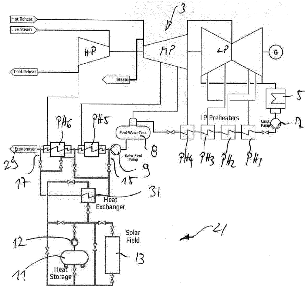
Figure 6: High Pressure indirect Integration with direct storage integration – Simplified Diagram
