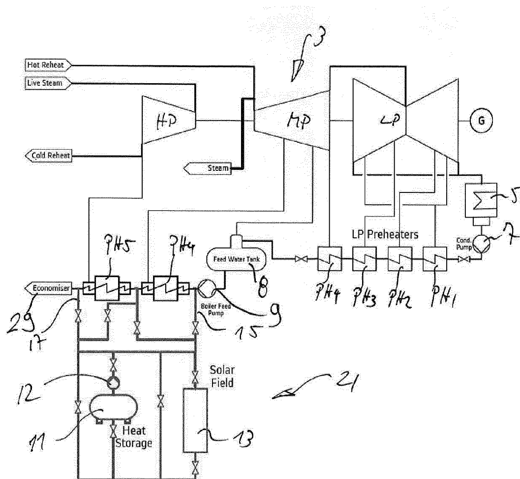
Figure 5: High Pressure direct Integration – Simplified Diagram
