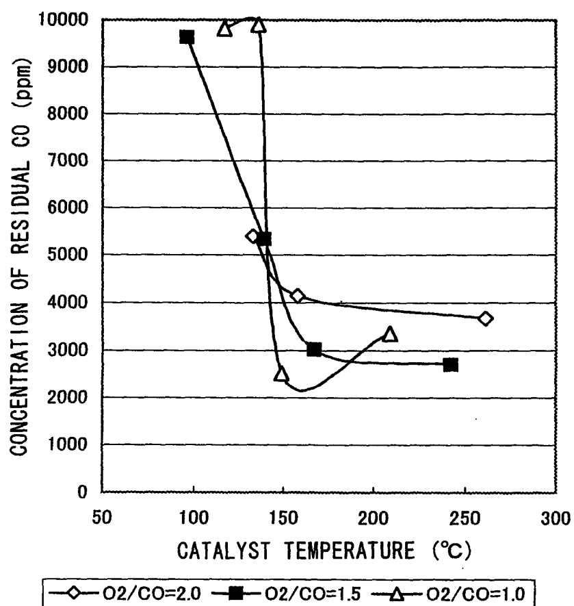
FIG. 2 COMPARATIVE EXAMPLE 1 (PURITY OF ALUMINA CARRIER: 99.9%)
