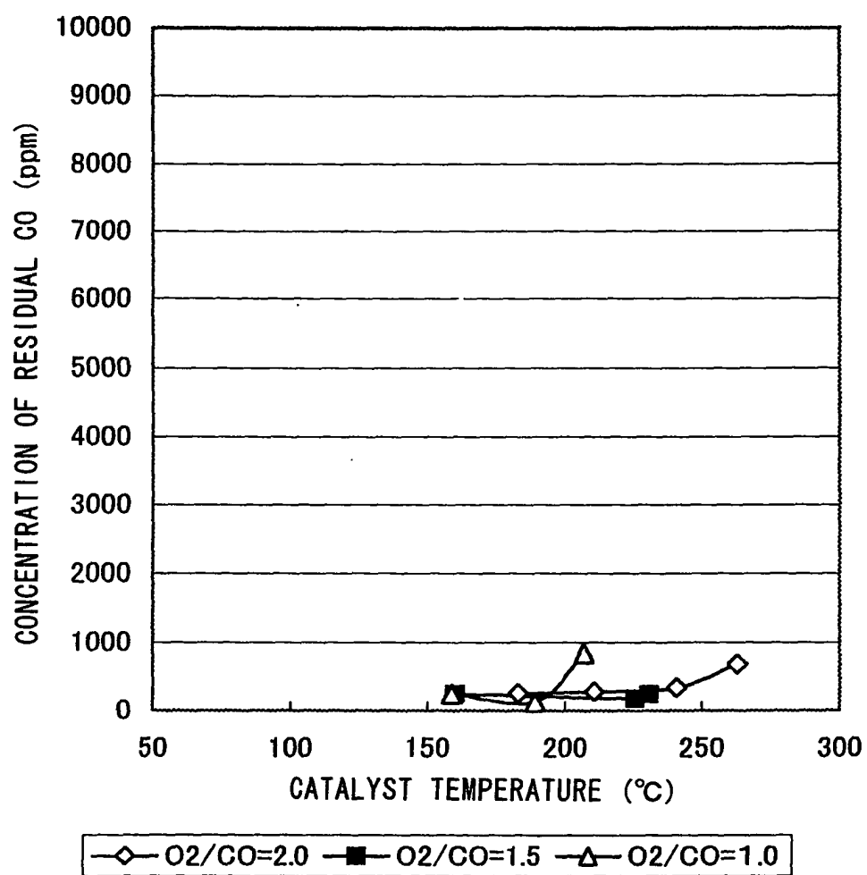
FIG. 1 EXAMPLE 2 (PURITY OF ALUMINA CARRIER: 99.995%)
