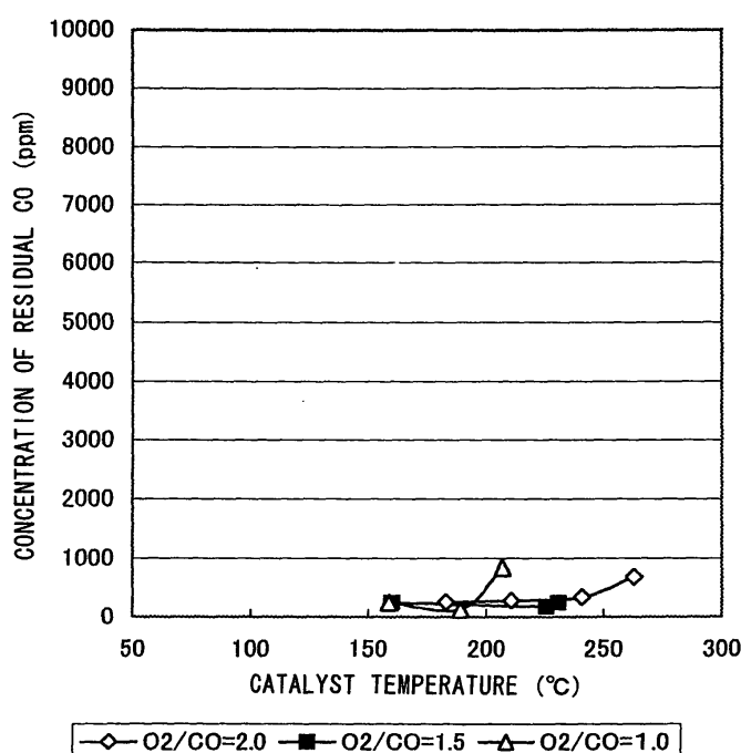
FIG. 1 EXAMPLE 2 (PURITY OF ALUMINA CARRIER: 99.995%)
