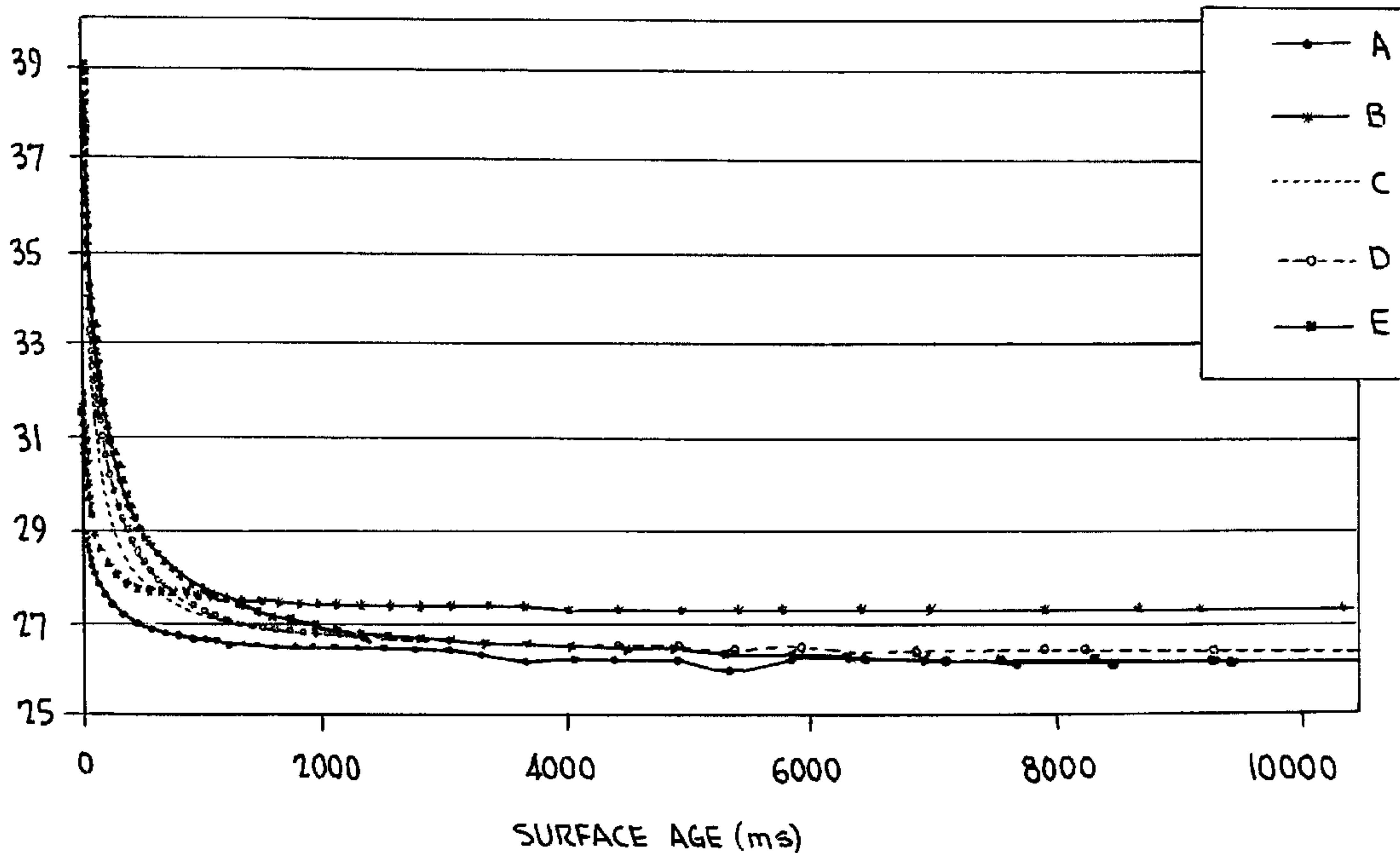
DYNAMIC SURFACE TENSION PLOT FOR CLOUDY VERSUS CLEAR EMULSIONS
