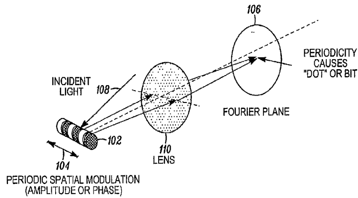
AN EXAMPLE OF A FOURIER PLANE READOUT OF A MULTILAYER METALLIC PARTICLE, WHICH OBIATES THE NEED FOR A HIGH RESOLUTION IMAGING SYSTEM
