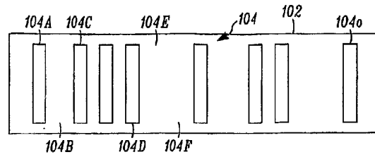
MICROBEAD INCLUDING CODE HAVING PERIODIC LAYERS OF MATERIAL WITH DIFFERENT REFLECTIVITY
