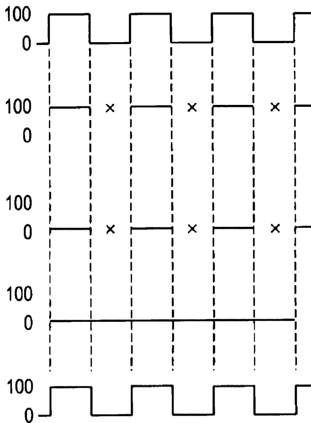
FIG. 5G R SIGNAL GENERATED BY ADDING BACK G SIGNAL
