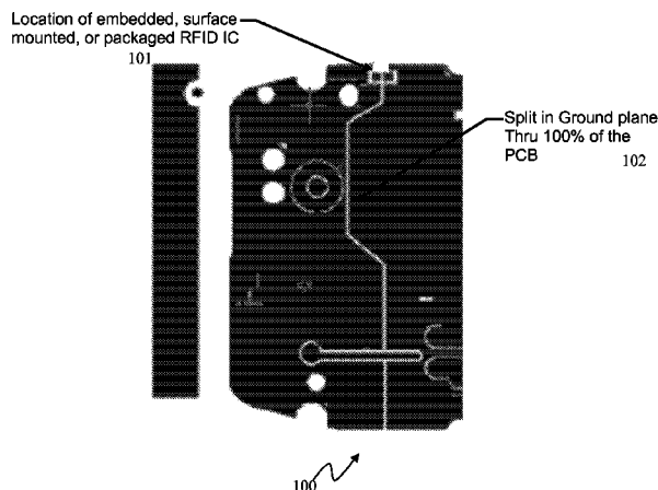
100% Split Ground Plane Antenna
