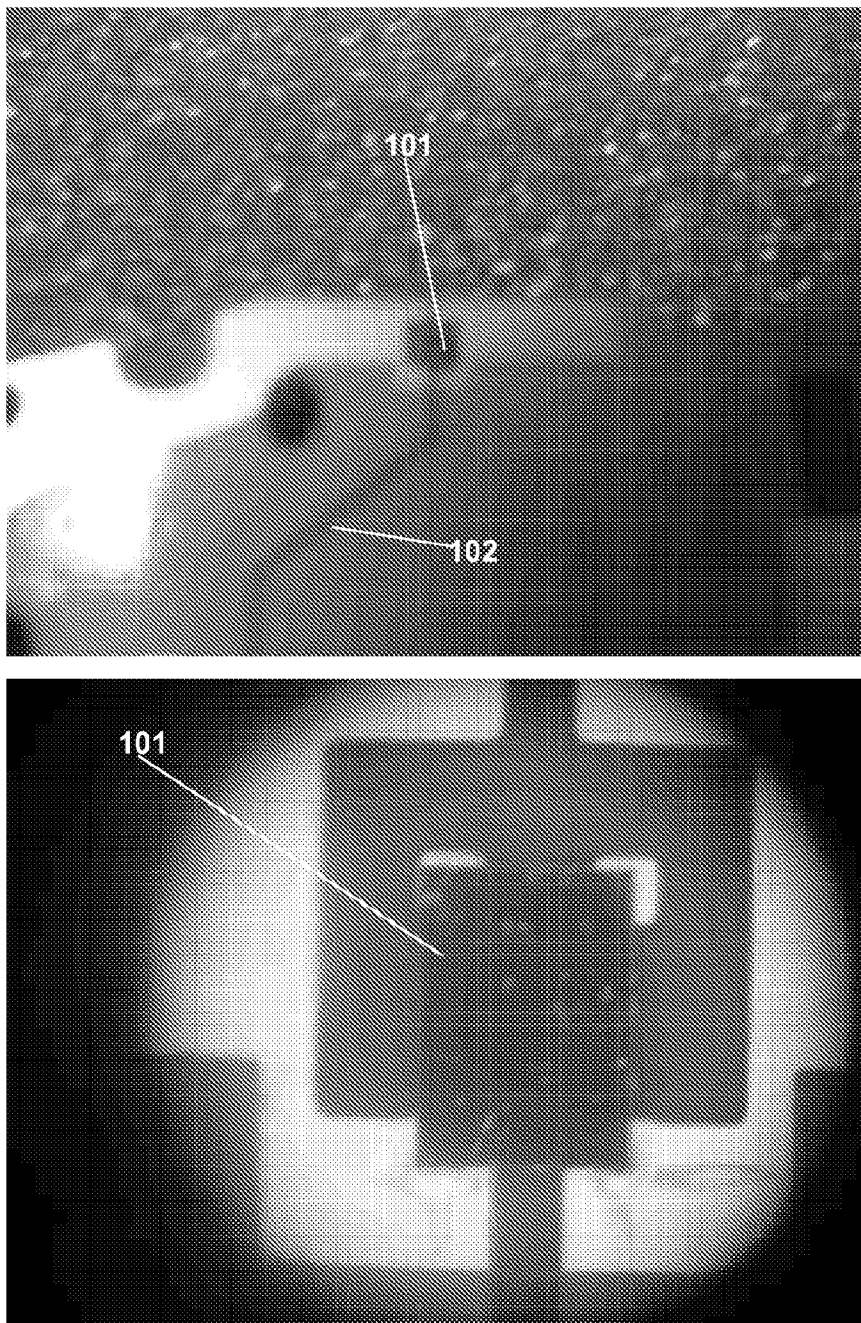
Example of Flip Chip Surface-Mounted RFID IC
