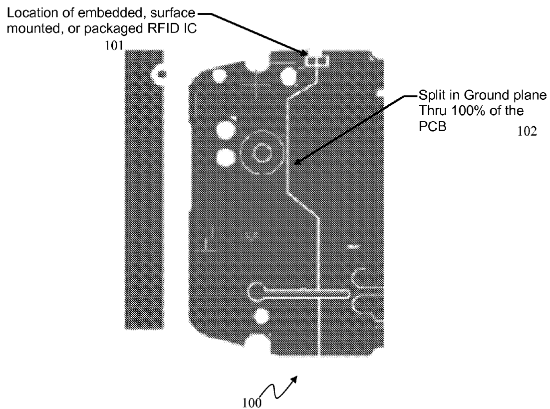
100% Split Ground Plane Antenna FIG. 1A
