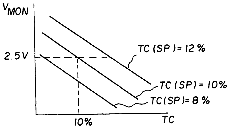
FIG. 7 (PRIOR ART)
