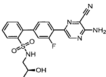
4'-(5-Amino-6-cyanopyrazin-2-yl)-3'-fluoro-N-[(2R)-2-hydroxypropyl]biphenyl-2-sulfonamide
