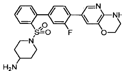
1-([4'-(3,4-Dihydro-2H-pyrido[3,2-b][1,4]oxazin-7-yl)-3'-fluorobiphenyl-2-yl]sulfonyl)piperidin-4-amine
