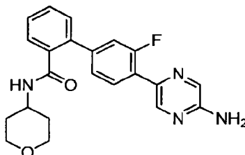
4'-{5-Aminopyrazin-2-yl}-3'-fluoro-N-(tetrahydro-2H-pyran-4-yl)biphenyl-2-carboxamide
