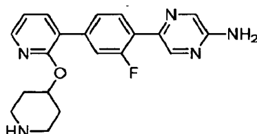
5-{2-Fluoro-4-[2-(piperidin-4-yloxy)pyridin-3-yl]phenyl}pyrazin-2-amine.
