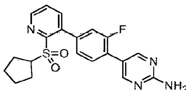
5-(4-(2-(Cyclopentylsulfonyl)pyridin-3-yl)-2-fluorophenyl)pyrimidine-2-amine hydrochloride
