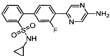
4'-(5-Aminopyrazin-2-yl)-N-cyclopropyl-3'-fluorobiphenyl-2-sulfonamide
