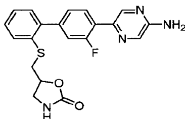
racemic 5- \{[4'\text{-(5-Aminopyrazin-2-yl)-3'-fluorobiphenyl-2-yl]sulfanyl}\} methyl)-1,3-oxazolidin-2-one
