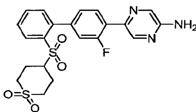
5-{2'-[(1,1-Dioxidotetrahydro-2H-thiopyran-4-yl)sulfonyl]-3-fluorobiphenyl-4-yl}pyrazin-2-amine
