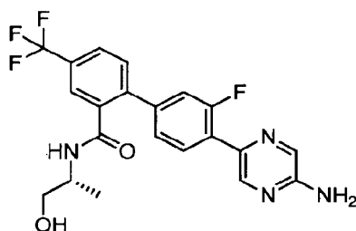
2-[4-(5-Aminopyrazin-2-yl)-3-fluoro-phenyl]-N-[(1 R )-2-hydroxy-1-methyl-ethyl]-5-(trifluoromethyl)benzamide
