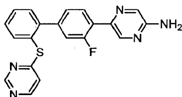
5-(3-Fluoro-2'-(pyrimidin-4-ylthio)-[1,1'-biphenyl]-4-yl)pyrazin-2-amine
