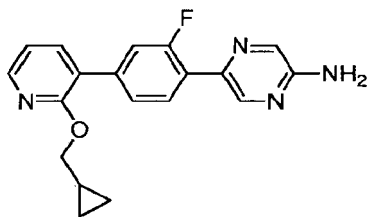
5-{4-[2-(Cyclopropylmethoxy)pyridin-3-yl]-2-fluorophenyl}pyrazin-2-amine
