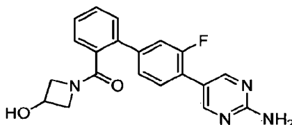
[2-[4-(2-Aminopyrimidin-5-yl)-3-fluoro-phenyl]phenyl]-[3-hydroxyazetidin-1-yl]methanone
