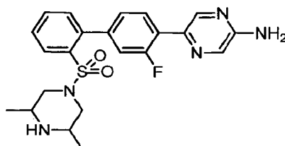
racemic-5-{2'-[(3,5-Dimethylpiperazin-1-yl)sulfonyl]-3-fluorobiphenyl-4-yl}pyrazin-2-amine
