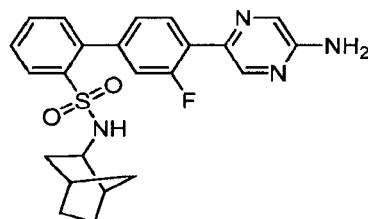
racemic (endo)-4'-(5-Aminopyrazin-2-yl)-N-bicyclo[2.2.1]hept-2-yl-3'-fluorobiphenyl-2-sulfonamide
