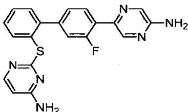
2-[[4'-(5-Aminopyrazin-2-yl)-3'-fluorobiphenyl-2-yl]sulfanyl]pyrimidin-4-amine hydrochloride
