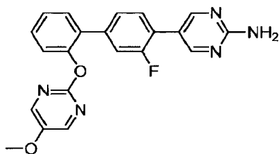
5-[3-Fluoro-2'-[(5-methoxypyrimidin-2-yl)oxy]biphenyl-4-yl]pyrimidin-2-amine
