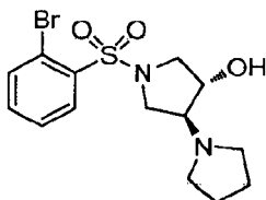
(Racemic)-1'-((2-Bromophenyl)sulfonyl)-[1,3'-bipyrrolidin]-4'-ol.
