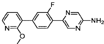
5-[2-Fluoro-4-(2-methoxypyridin-3-yl)phenyl]pyrazin-2-amine
