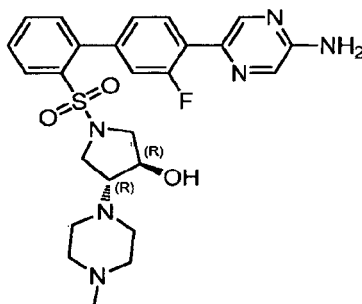
Racemic-1-([4'-(5-Aminopyrazin-2-yl)-3'-fluorobiphenyl-2-yl]sulfonyl)-4-(4-methylpiperazin-1-yl)-pyrrolidin-3-ol trifluoroacetic acid salt
