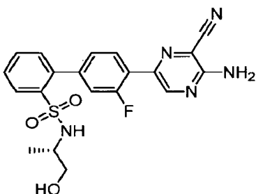
4'-(5-amino-6-cyanopyrazin-2-yl)-3'-fluoro-N-[(1R)-2-hydroxy-1-methylethyl]biphenyl-2-sulfonamide
