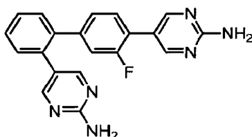
5,5'-(3'-Fluorobiphenyl-2,4'-diyl)dipyrimidin-2-amine.
