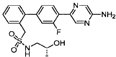
( R )-1-[4'-(5-Aminopyrazin-2-yl)-3'-fluorobiphenyl-2-yl]- N -[(2 R )-2-hydroxypropyl]-methanesulfonamide
