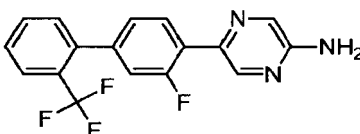
5-[3-Fluoro-2'-(trifluoromethyl)biphenyl-4-yl]pyrazin-2-amine
