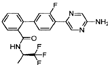
4'-(5-Aminopyrazin-2-yl)-3'-fluoro-N-[(1R)-2,2,2-trifluoro-1-methylethyl]biphenyl-2-carboxamide
