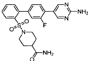
1-((4'-(2-Aminopyrimidin-5-yl)-3'-fluoro-[1,1'-biphenyl]-2-yl)sulfonyl)piperidine-4-carboxamide
