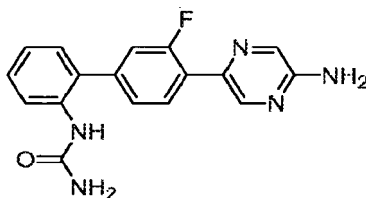
1-[4'-(5-Aminopyrazin-2-yl)-3'-fluorobiphenyl-2-yl]urea
