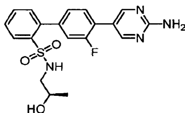
4'-(2-Aminopyrimidin-5-yl)-3'-fluoro-N-[(2R)-2-hydroxypropyl]biphenyl-2-sulfonamide-trifluoroacetic acid salt
