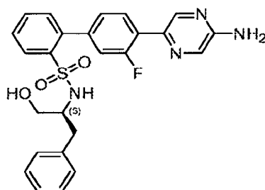
(S)-4'-(5-Aminopyrazin-2-yl)-3'-fluoro-N-(1-hydroxy-3-phenylpropan-2-yl)-[1,1'-biphenyl]-2-sulfonamide
