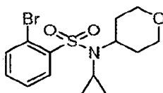
2-Bromo- N -cyclopropyl- N -(tetrahydro-2 H -pyran-4-yl)benzenesulfonamide
