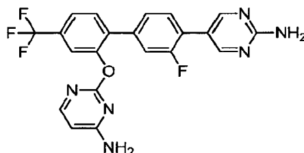
5-{2'-[(4-Aminopyrimidin-2-yl)oxy]-3-fluoro-4'-(trifluoromethyl)biphenyl-4-yl}pyrimidin-2-amine
