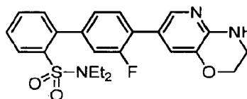
4'-((3,4-Dihydro-2H-pyrido[3,2-b][1,4]oxazin-7-yl)-N,N-diethyl-3'-fluorobiphenyl-2-sulfonamide
