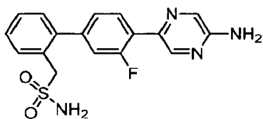
1-[4'-(5-Aminopyrazin-2-yl)-3'-fluorobiphenyl-2-yl]methanesulfonamide hydrochloride
