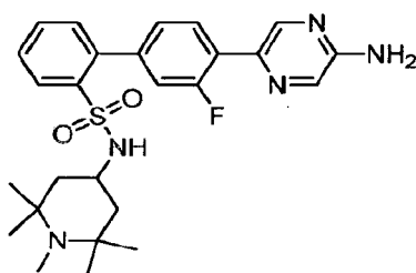
4'-(5-Aminopyrazin-2-yl)-3'-fluoro-N-(1,2,2,6,6-pentamethylpiperidin-4-yl)biphenyl-2-sulfonamide
