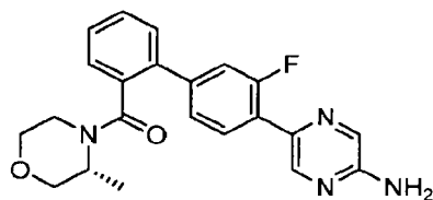
5-(3-Fluoro-2'--[(3R)-3-methylmorpholin-4-yl]carbonyl)biphenyl-4-yl)pyrazin-2-amine
