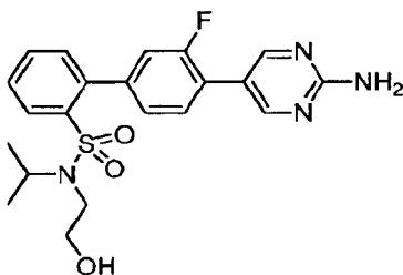
4'-(2-Aminopyrimidin-5-yl)-3'-fluoro-N-(2-hydroxyethyl)-N-(1-methylethyl)biphenyl-2-sulfonamide
