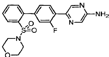
5-[3-Fluoro-2'-(morpholin-4-ylsulfonyl)biphenyl-4-yl]pyrazin-2-amine
