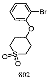
4-(2-Bromophenoxy)tetrahydro-2H-thiopyran 1,1-dioxide
