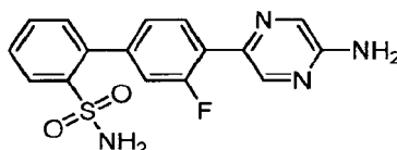
4'-(5-Aminopyrazin-2-yl)-3'-fluorobiphenyl-2-sulfonamide
