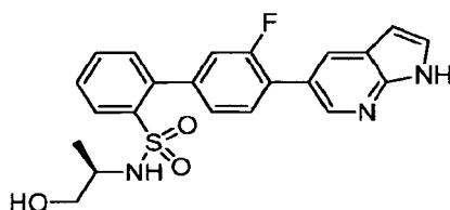
3'-Fluoro- N -[(1 R )-2-hydroxy-1-methylethyl]-4'-(1 H -pyrrolo[2,3- b ]pyridin-5-yl)biphenyl-2-sulfonamide
