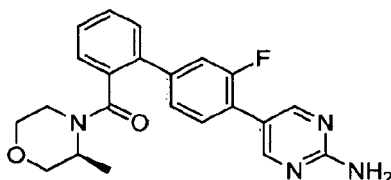
5-(3-Fluoro-2'--[(3S)-3-methylmorpholin-4-yl]carbonyl)biphenyl-4-yl)pyrimidin-2-amine
