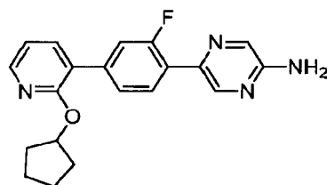
5-{4-[2-(Cyclopentyloxy)pyridin-3-yl]-2-fluorophenyl}pyrazin-2-amine
