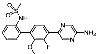
N -[4'-(5-Aminopyrazin-2-yl)-3'-fluoro-2'-methoxybiphenyl-2-yl]methanesulfonamide.
