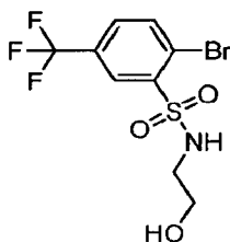
2-Bromo-N-(2-hydroxyethyl)-5-(trifluoromethyl)benzenesulfonamide.
