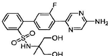
4'-(5-Aminopyrazin-2-yl)-3'-fluoro-N-[2-hydroxy-1-(hydroxymethyl)-1-methylethyl]biphenyl-2-sulfonamide
