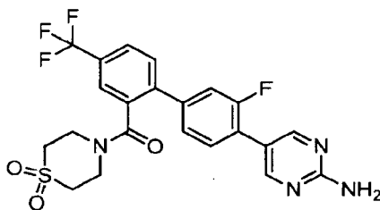
[2-[4-(2-Aminopyrimidin-5-yl)-3-fluoro-phenyl]-5-(trifluoromethyl)phenyl]-(1,1-dioxo-1,4-thiazinan-4-yl)methanone
