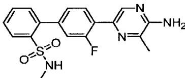
4'-(5-Amino-6-methylpyrazin-2-yl)-3'-fluoro- N -methylbiphenyl-2-sulfonamide
