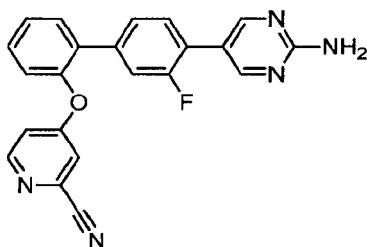
4-{[4'-(2-Aminopyrimidin-5-yl)-3'-fluorobiphenyl-2-yl]oxy}pyridine-2-carbonitrile
