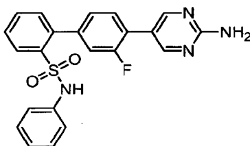
4'-(2-Aminopyrimidin-5-yl)-3'-fluoro- N -phenylbiphenyl-2-sulfonamide trifluoroacetic acid salt
