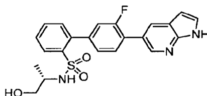
3-Fluoro- N -[(1 S )-2-hydroxy-1-methylethyl]-4'-((1 H -pyrrolo[2,3- b ]pyridin-5-yl)biphenyl-2-sulfonamide
