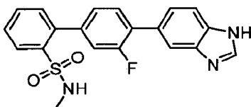
4'-(1 H -Benzimidazol-5-yl)-3'-fluoro- N -methylbiphenyl-2-sulfonamide
