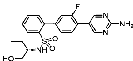
4'-(2-Aminopyrimidin-5-yl)-3'-fluoro- N -[(1 S )-1-(hydroxymethyl)propyl]biphenyl-2-sulfonamide
