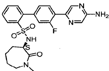
(S)-4'-(5-Aminopyrazin-2-yl)-3'-fluoro-N-[(3S)-1-methyl-2-oxoazepan-3-yl]biphenyl-2-sulfonamide
