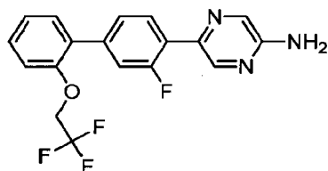
5-[3-Fluoro-2'-(2,2,2-trifluoroethoxy)biphenyl-4-yl]pyrazin-2-amine
