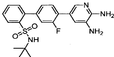
N -tert-Butyl-4'-(5,6-diaminopyridin-3-yl)-3'-fluorobiphenyl-2-sulfonamide
