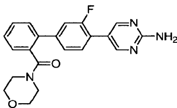
5-[3-Fluoro-2'-(morpholin-4-ylcarbonyl)biphenyl-4-yl]pyrimidin-2-amine
