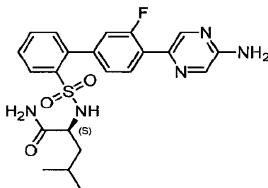
(S)-2-(4'-(5-Aminopyrazin-2-yl)-3'-fluoro-[1,1'-biphenyl]-2-ylsulfonamido)-4-methylpentanamide
