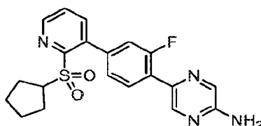
5-(4-(2-(Cyclopentylsulfonyl)pyridin-3-yl)-2-fluorophenyl)pyrazin-2-amine hydrochloride
