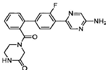
4-{{4'-(5-Aminopyrazin-2-yl)-3'-fluorobiphenyl-2-yl}carbonyl}piperazin-2-one
