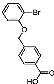
4-((2-Bromophenoxy)methyl)benzoic acid
