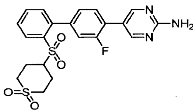
5-({2'-[1,1-Dioxidotetrahydro-2H-thiopyran-4-yl)sulfonyl]-3-fluorobiphenyl-4-yl}pyrimidin-2-amine hydrochloride
