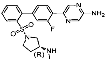
(R)-5-(3-Fluoro-2'-{[3-(methylamino)pyrrolidin-1-yl]sulfonyl}biphenyl-4-yl)pyrazin-2-amine
