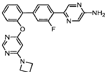
5-{2'-[(6-Azetidin-1-ylpyrimidin-4-yl)oxy]-3-fluorobiphenyl-4-yl}pyrazin-2-amine
