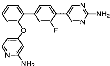
5-{2'-[(2-Aminopyridin-4-yl)oxy]-3-fluorobiphenyl-4-yl}pyrimidin-2-amine.
