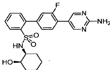
racemic cis 4'-(2-Aminopyrimidin-5-yl)-3'-fluoro-N-[(cis)-2-hydroxycyclohexyl]biphenyl-2-sulfonamide
