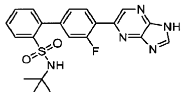
N - tert -Butyl-3'-fluoro-4'-(1 H -imidazo[4,5- b ]pyrazin-5-yl)biphenyl-2-sulfonamide
