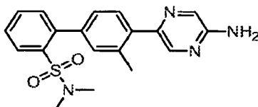
4'-(5-Aminopyrazin-2-yl)- N,N ,3'-trimethylbiphenyl-2-sulfonamide.
