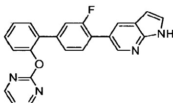
5-[3-Fluoro-2'-(pyrimidin-2-yloxy)biphenyl-4-yl]-1 H -pyrrolo[2,3- b ]pyridine
