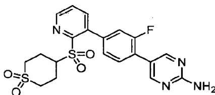
4-((3-(4-(2-aminopyrimidin-5-yl)-3-fluorophenyl)pyridine-2-yl)sulfonyl)tetrahydro-2H-thiopyran 1,1-dioxide
