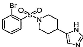
1-[(2-Bromophenyl)sulfonyl]-4-(1 H -imidazol-4-yl)piperidine
