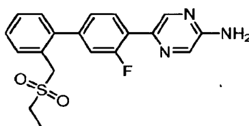
5-{2'-[(Ethylsulfonyl)methyl]-3-fluorobiphenyl-4-yl}pyrazin-2-amine hydrogen chloride salt
