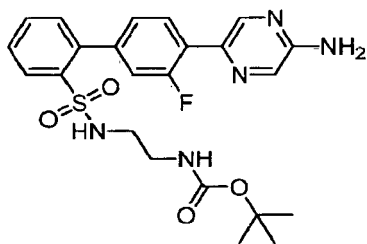
tert -Butyl [2-({4'-({5-aminopyrazin-2-yl})-3'-fluorobiphenyl-2-yl}sulfonyl)amino]ethyl]carbamate
