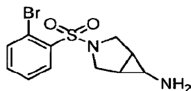
endo -3-[(2-Bromophenyl)sulfonyl]-3-azabicyclo[3.1.0]hexan-6-amine
