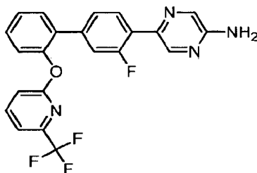
5-(3-Fluoro-2'--([6-(trifluoromethyl)pyridin-2-yl]oxy)biphenyl-4-yl)pyrazin-2-amine.
