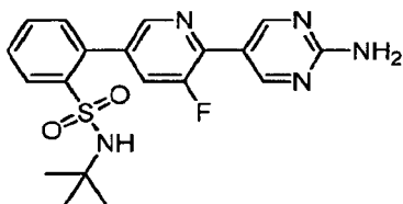
2-[6-(2-Aminopyrimidin-5-yl)-5-fluoropyridin-3-yl]-N-tert-butylbenzenesulfonamide.
