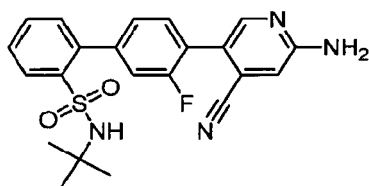
4'-(6-Amino-4-cyanopyridin-3-yl)- N - tert -butyl-3'-fluorobiphenyl-2-sulfonamide
