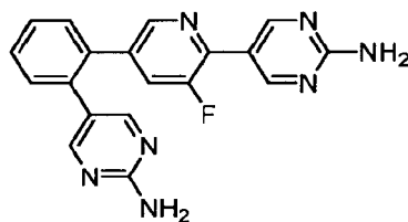
5-{2-[6-(2-Aminopyrimidin-5-yl)-5-fluoropyridin-3-yl]phenyl}pyrimidin-2-amine.
