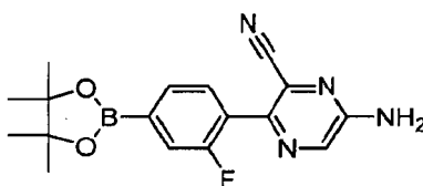
6-Amino-3-(2-fluoro-4-(4,4,5,5-tetramethyl-1,3,2-dioxaborolan-2-yl)phenyl)pyrazine-2-carbonitrile
