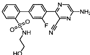
4'-(5-Amino-3-cyanopyrazin-2-yl)-3'-fluoro-N-(2-hydroxyethyl)biphenyl-2-sulfonamide
