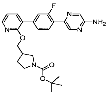
tert -Butyl 3-(((3-(4-(5-aminopyrazin-2-yl)-3-fluorophenyl)pyridin-2-yl)oxy)methyl)pyrrolidine-1-carboxylate
