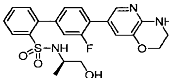
4'-((3,4-Dihydro-2H-pyrido[3,2-b][1,4]oxazin-7-yl)-3'-fluoro-N-((1R)-2-hydroxy-1-methylethyl)biphenyl-2-sulfonamide
