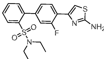
4'-(2-Amino-1,3-thiazol-4-yl)- N,N -diethyl-3'-fluorobiphenyl-2-sulfonamide
