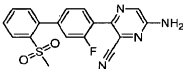
6-Amino-3-[3-fluoro-2'-(methylsulfonyl)biphenyl-4-yl]pyrazine-2-carbonitrile
