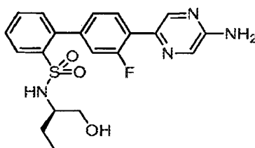
4'-(5-Aminopyrazin-2-yl)-3'-fluoro- N -[(1 R )-1-(hydroxymethyl)propyl]biphenyl-2-sulfonamide
