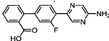
4'-(5-Aminopyrazin-2-yl)-3'-fluorobiphenyl-2-carboxylic acid
