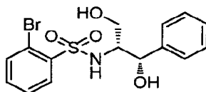
2-Bromo- N -[(1 S ,2 S )-2-hydroxy-1-(hydroxymethyl)-2-phenylethyl]benzenesulfonamide
