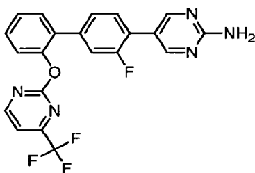
5-(3-Fluoro-2'--[[4-(trifluoromethyl)pyrimidin-2-yl]oxy]biphenyl-4-yl)pyrimidin-2-amine.
