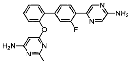
6-([4'-(5-Aminopyrazin-2-yl)-3'-fluorobiphenyl-2-yl]oxy)-2-methylpyrimidin-4-amine.
