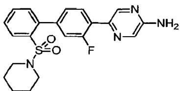
5-[3-Fluoro-2'-(piperidin-1-ylsulfonyl)biphenyl-4-yl]pyrazin-2-amine
