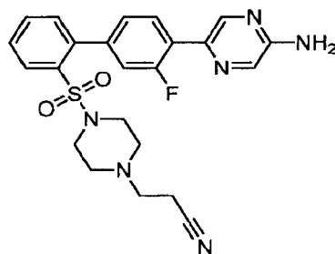
3-(4-({4'-(5-Aminopyrazin-2-yl)-3'-fluorobiphenyl-2-yl}sulfonyl)piperazin-1-yl)propanenitrile
