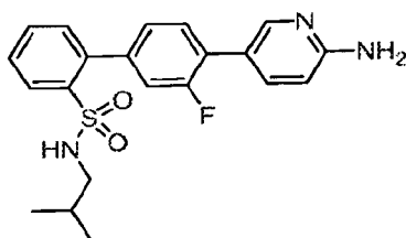
4'-(6-Aminopyridin-3-yl)-3'-fluoro-N-iso-butyl-[1,1'-biphenyl]-2-sulfonamide
