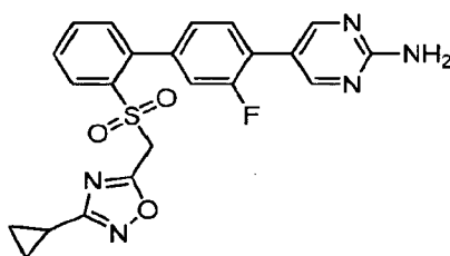
5-(2'-([3-(Cyclopropyl-1,2,4-oxadiazol-5-yl)methylsulfonyl]-3-fluorobiphenyl-4-yl)pyrimidin-2-amine
