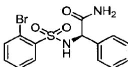
(2 R )-2-~[(2-Bromophenyl)sulfonyl]amino~-2-phenylethanamide
