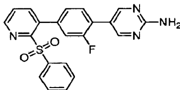
5-{2-Fluoro-4-[2-(phenylsulfonyl)pyridin-3-yl]phenyl}pyrimidin-2-amine.
