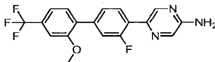
5-[3-Fluoro-2'-methoxy-4'-(trifluoromethyl)biphenyl-4-yl]pyrazin-2-amine
