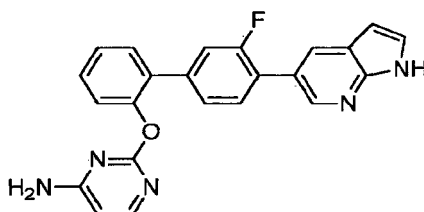
2-([3'-Fluoro-4'-(1 H -pyrrolo[2,3- b ]pyridin-5-yl)biphenyl-2-yl]oxy)pyrimidin-4-amine
