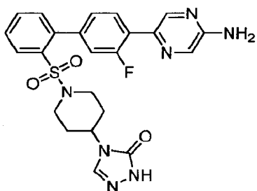
4-(1-([4'-(5-Aminopyrazin-2-yl)-3'-fluorobiphenyl-2-yl]sulfonyl)piperidin-4-yl)-2,4-dihydro-3H-1,2,4-triazol-3-one
