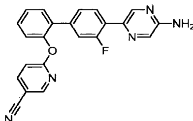
6-{{4'-(5-Aminopyrazin-2-yl)-3'-fluorobiphenyl-2-yl}oxy}pyridine-3-carbonitrile.
