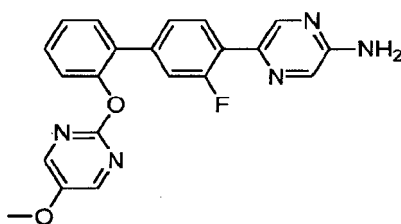
5-(3-Fluoro-2'-{[5-methoxypyrimidin-2-yl]oxy}biphenyl-4-yl)pyrazin-2-amine
