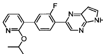
2-{2-Fluoro-4-[2-(1-methylethoxy)pyridin-3-yl]phenyl}-5H-pyrrolo[2,3-b]pyrazine
