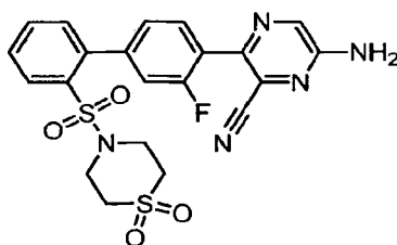
6-Amino-3-{2'-[1,1-dioxidothiomorpholin-4-yl)sulfonyl]-3-fluorobiphenyl-4-yl}pyrazine-2-carbonitrile
