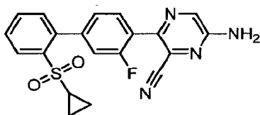
6-Amino-3-[2'-(cyclopropylsulfonyl)-3-fluorobiphenyl-4-yl]pyrazine-2-carbonitrile
