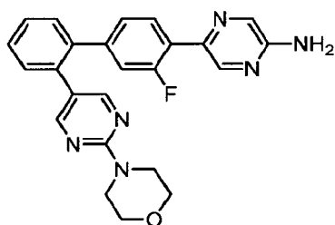
5-((3-Fluoro-2'-(2-morpholin-4-yl)pyrimidin-5-yl)biphenyl-4-yl)pyrazin-2-amine.
