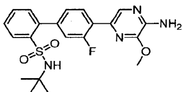
4'-(5-Amino-6-methoxypyrazin-2-yl)- N - tert -butyl-3'-fluorobiphenyl-2-sulfonamide
