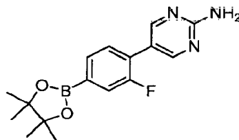
5-(2-Fluoro-4-(4,4,5,5-tetramethyl-1,3,2-dioxaborolan-2-yl)phenyl)pyrimidin-2-amine
