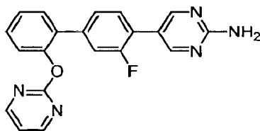
5-[3-Fluoro-2'-(pyrimidin-2-yloxy)biphenyl-4-yl]pyrimidin-2-amine
