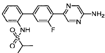
N -(4'-(5-Aminopyrazin-2-yl)-3'-fluoro-[1,1'-biphenyl]-2-yl)propane-2-sulfonamide
