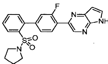
2-[3-Fluoro-2'-(pyrrolidin-1-ylsulfonyl)biphenyl-4-yl]-5 H -pyrrolo[2,3- b ]pyrazine
