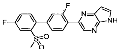
2-[3,4'-Difluoro-2'-(methylsulfonyl)biphenyl-4-yl]-5H-pyrrolo[2,3-b]pyrazine
