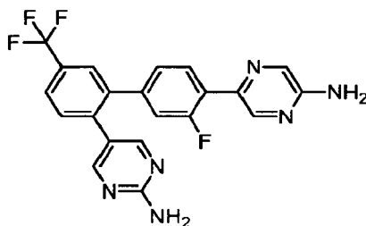
5-[4'-(5-Aminopyrazin-2-yl)-3'-fluoro-5-(trifluoromethyl)biphenyl-2-yl]pyrimidin-2-amine.
