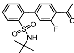
4'-Acetyl-N-tert-butyl-3'-fluorobiphenyl-2-sulfonamide
