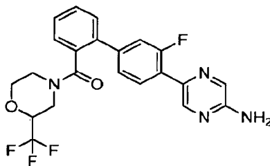
racemic 5-(3-Fluoro-2'-{[2-(trifluoromethyl)morpholin-4-yl]carbonyl}biphenyl-4-yl)pyrazin-2-amine
