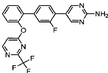
5-(3-Fluoro-2'-{[2-(trifluoromethyl)pyrimidin-4-yl]oxy}biphenyl-4-yl)pyrimidin-2-amine
