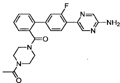
5-{2'-[(4-Acetylpiperazin-1-yl)carbonyl]-3-fluorobiphenyl-4-yl}pyrazin-2-amine
