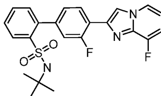
N -tert-Butyl-3'-fluoro-4'-(8-fluoroimidazo[1,2-a]pyridin-2-yl)biphenyl-2-sulfonamide
