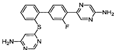
6-[[4'-(5-Aminopyrazin-2-yl)-3'-fluorobiphenyl-2-yl]sulfanyl]pyrimidin-4-amine hydrochloride
