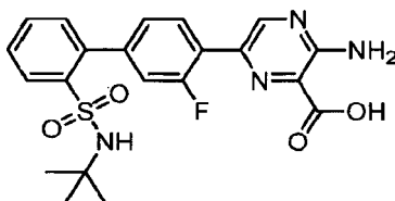
3-Amino-6-{2'-[(tert-butylsulfamoyl)-3-fluorobiphenyl-4-yl]pyrazine-2-carboxylic acid.
