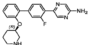
5-{3-Fluoro-2'-[(3R)-piperidin-3-yloxy]biphenyl-4-yl}pyrazin-2-amine.
