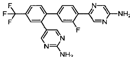
5-[4'-(5-Aminopyrazin-2-yl)-3'-fluoro-4-(trifluoromethyl)biphenyl-2-yl]pyrimidin-2-amine.
