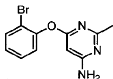
6-(2-Bromophenoxy)-2-methylpyrimidin-4-amine
