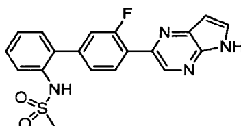
N -[3'-Fluoro-4'-(5H-pyrrolo[2,3-b]pyrazin-2-yl)biphenyl-2-yl]methanesulfonamide
