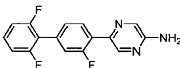
5-(2',3,6'-Trifluorobiphenyl-4-yl)pyrazin-2-amine
