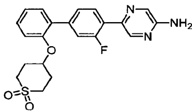
5-{2'-[({1,1-Dioxidotetrahydro-2H-thiopyran-4-yl}oxy)-3-fluorobiphenyl-4-yl]pyrazin-2-amine.
