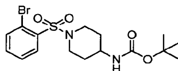
tert -Butyl (1-((2-bromophenyl)sulfonyl)piperidin-4-yl)carbamate.
