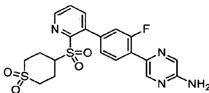
4-((3-(4-(2-Aminopyrazin-5-yl)-3-fluorophenyl)pyridine-2-yl)sulfonyl)tetrahydro-2H-thiopyran 1,1-dioxide
