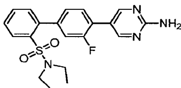
4'-(2-Aminopyrimidin-5-yl)- N,N -diethyl-3'-fluorobiphenyl-2-sulfonamide trifluoroacetic acid salt
