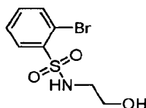
2-Bromo-N-(2-hydroxyethyl)benzenesulfonamide
