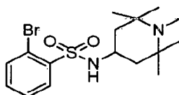
2-Bromo- N -(1,2,2,6,6-pentamethylpiperidin-4-yl)benzenesulfonamide
