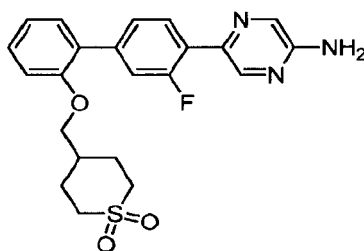
5-{2'-[1,1-Dioxidotetrahydro-2H-thiopyran-4-yl)methoxy]-3-fluorobiphenyl-4-yl}pyrazin-2-amine.
