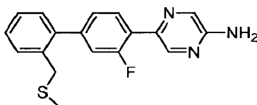
5-(3-Fluoro-2'-[(methylsulfanyl)methyl]biphenyl-4-yl)pyrazin-2-amine hydrochloride
