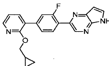
2-{4-[2-(Cyclopropylmethoxy)pyridin-3-yl]-2-fluorophenyl}-5H-pyrrolo[2,3-b]pyrazine
