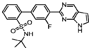
N -tert-Butyl-3'-fluoro-4'-(7H-pyrrolo[2,3-d]pyrimidin-2-yl)biphenyl-2-sulfonamide
