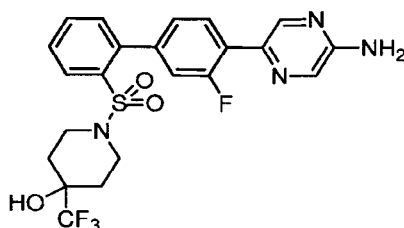
1-[[4'-(5-Aminopyrazin-2-yl)-3'-fluorobiphenyl-2-yl]sulfonyl]-4-(trifluoromethyl)piperidin-4-ol
