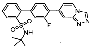
N - tert -Butyl-3'-fluoro-4'-[1,2,4]triazolo[4,3- a ]pyridin-7-ylbiphenyl-2-sulfonamide
