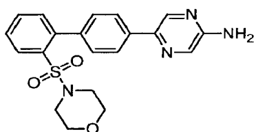
5-[2'-(Morpholin-4-ylsulfonyl)biphenyl-4-yl]pyrazin-2-amine
