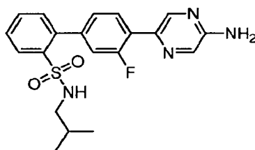
4'-(5-Aminopyrazin-2-yl)-3'-fluoro-N-(2-methylpropyl)biphenyl-2-sulfonamide
