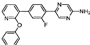
5-[2-Fluoro-4-(2-phenoxypyridin-3-yl)phenyl]pyrazin-2-amine.
