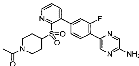
1-((3-(4-(2-Aminopyrazin-5-yl)-3-fluorophenyl)pyridine-2-yl)sulfonyl)piperidin-1-yl)ethanone hydrogen chloride salt
