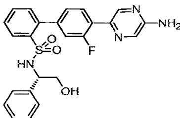
4'-(5-Aminopyrazin-2-yl)-3'-fluoro-N-[(1S)-2-hydroxy-1-phenylethyl]biphenyl-2-sulfonamide
