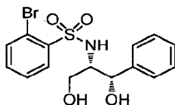
2-bromo-N-((1S,2S)-1,3-dihydroxy-1-phenylpropan-2-yl)benzenesulfonamide.
