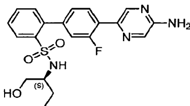
(S)-4'-(5-Aminopyrazin-2-yl)-3'-fluoro-N-(1-hydroxybutan-2-yl)-[1,1'-biphenyl]-2-sulfonamide
