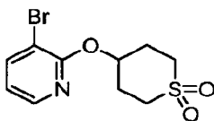
4-((3-Bromopyridin-2-yl)oxy)tetrahydro-2H-thiopyran 1,1-dioxide
