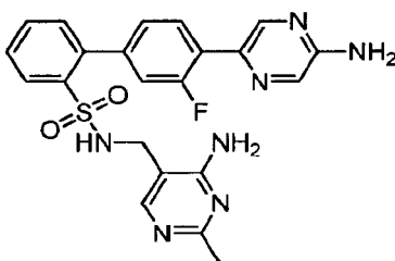
N-[(4-Amino-2-methylpyrimidin-5-yl)methyl]-4'-(5-aminopyrazin-2-yl)-3'-fluorobiphenyl-2-sulfonamide
