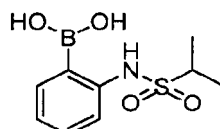
(2-(1-Methylethylsulfonamido)phenyl)boronic acid
