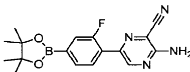
3-Amino-6-(2-fluoro-4-(4,4,5,5-tetramethyl-1,3,2-dioxaborolan-2-yl)phenyl)pyrazine-2-carbonitrile
