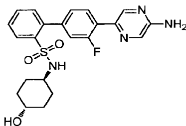
trans 4'-(5-Aminopyrazin-2-yl)-3'-fluoro- N -(4-hydroxycyclohexyl)biphenyl-2-sulfonamide
