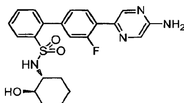
4'-(5-Aminopyrazin-2-yl)-3'-fluoro- N -[(1 R ,2 R )-2-hydroxycyclohexyl]biphenyl-2-sulfonamide
