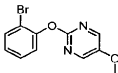
2-(2-Bromophenoxy)-5-methoxypyrimidine
