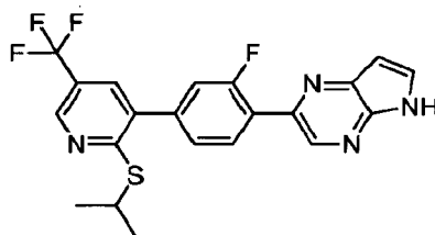
2-(2-Fluoro-4-{2-[(1-methylethyl)sulfanyl]-5-(trifluoromethyl)pyridin-3-yl}phenyl)-5H-pyrrolo[2,3-b]pyrazine
