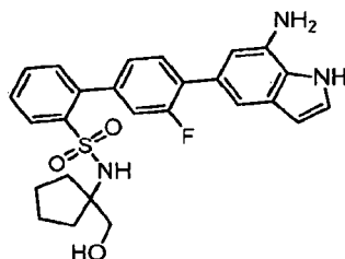
4'-(7-Amino-1 H -indol-5-yl)-3'-fluoro- N -[1-(hydroxymethyl)cyclopentyl]biphenyl-2-sulfonamide
