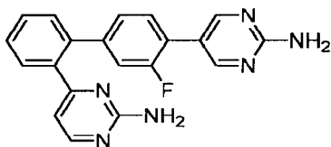
4-[4'-(2-Aminopyrimidin-5-yl)-3'-fluorobiphenyl-2-yl]pyrimidin-2-amine.
