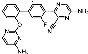
6-Amino-3-{2'-[(4-aminopyrimidin-2-yl)oxy]-3-fluorobiphenyl-4-yl}pyrazine-2-carbonitrile
