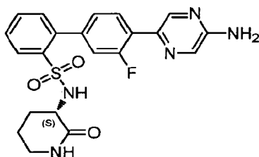
(S)-4'-(5-Aminopyrazin-2-yl)-3'-fluoro-N-(2-oxopiperidin-3-yl)-[1,1'-biphenyl]-2-sulfonamide
