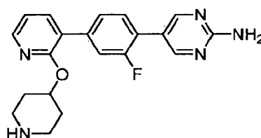
5-{2-Fluoro-4-[2-(piperidin-4-yloxy)pyridin-3-yl]phenyl}pyrimidin-2-amine.
