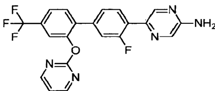
5-[3-Fluoro-2'-(pyrimidin-2-yloxy)-4'-(trifluoromethyl)biphenyl-4-yl]pyrazin-2-amine
