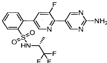
2-[6-(2-Aminopyrimidin-5-yl)-5-fluoropyridin-3-yl]- N -[(1 R )-2,2,2-trifluoro-1-methylethyl]benzenesulfonamide.
