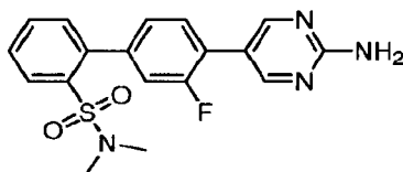
4'-(2-Aminopyrimidin-5-yl)-3'-fluoro- N,N -dimethylbiphenyl-2-sulfonamide trifluoroacetic acid salt
