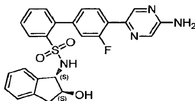
4'-(5-Aminopyrazin-2-yl)-3'-fluoro- N -((1 S ,2 S )-2-hydroxy-2,3-dihydro-1 H -inden-1-yl)-[1,1'-biphenyl]-2-sulfonamide
