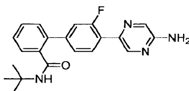
4'-(5-Aminopyrazin-2-yl)-N-tert-butyl-3'-fluorobiphenyl-2-carboxamide
