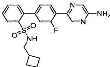
4'-(5-Aminopyrazin-2-yl)-N-(cyclobutylmethyl)-3'-fluorobiphenyl-2-sulfonamide
