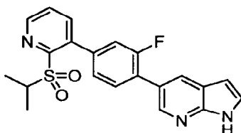
5-(2-Fluoro-4-(2-(isopropylsulfonyl)pyridine-3-yl)phenyl)-1H-pyrrolo[2,3-b]pyridine
