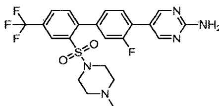
5-{3-Fluoro-2'-[(4-methylpiperazin-1-yl)sulfonyl]-4'-(trifluoromethyl)biphenyl-4-yl}pyrimidin-2-amine
