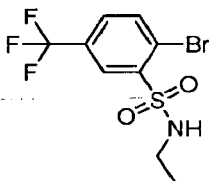
2-Bromo- N -ethyl-5-(trifluoromethyl)benzenesulfonamide.
