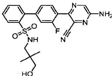
4'-(5-Amino-3-cyanopyrazin-2-yl)-3'-fluoro-N-(3-hydroxy-2,2-dimethylpropyl)biphenyl-2-sulfonamide
