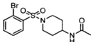
N-(1-((2-Bromophenyl)sulfonyl)piperidin-4-yl)acetamide.
