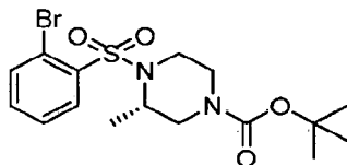
tert -Butyl (3 S )-4-[(2-bromophenyl)sulfonyl]-3-methylpiperazine-1-carboxylate
