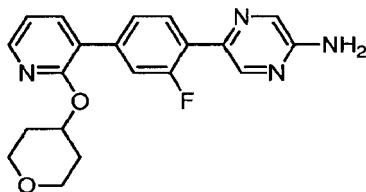
5-{2-Fluoro-4-[2-(tetrahydro-2H-pyran-4-yloxy)pyridin-3-yl]phenyl}pyrazin-2-amine.
