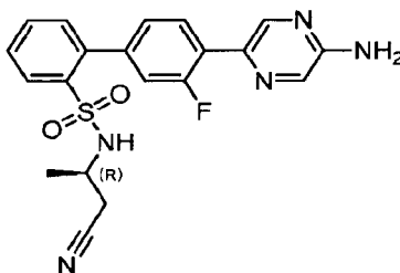
(R)-4'-(5-Aminopyrazin-2-yl)-N-(1-cyanopropan-2-yl)-3'-fluoro-[1,1'-biphenyl]-2-sulfonamide
