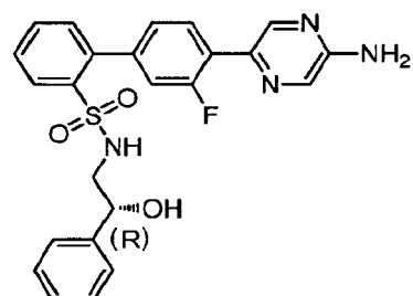
(R)-4'-(5-Aminopyrazin-2-yl)-3'-fluoro-N-(2-hydroxy-2-phenylethyl)-[1,1'-biphenyl]-2-sulfonamide
