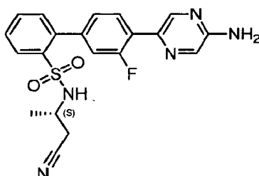
(S)-4'-(5-Aminopyrazin-2-yl)-N-(1-cyanopropan-2-yl)-3'-fluoro-[1,1'-biphenyl]-2-sulfonamide
