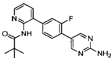
N -{3-[4-(2-Aminopyrimidin-5-yl)-3-fluorophenyl]pyridin-2-yl}-2,2-dimethylpropanamide
