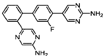
5-[2'-(5-Aminopyrazin-2-yl)-3-fluorobiphenyl-4-yl]pyrimidin-2-amine.
