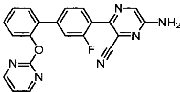
6-Amino-3-[3-fluoro-2'-(pyrimidin-2-yloxy)biphenyl-4-yl]pyrazine-2-carbonitrile
