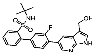
N - tert -Butyl-3'-fluoro-4'-(3-(hydroxymethyl)-1 H -pyrrolo[2,3- b ]pyridin-5-yl)biphenyl-2-sulfonamide
