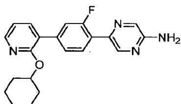
5-{4-[2-(Cyclohexyloxy)pyridin-3-yl]-2-fluorophenyl}pyrazin-2-amine
