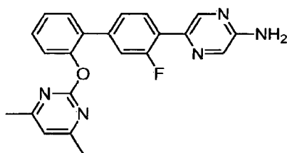
5-{2'-[(4,6-Dimethylpyrimidin-2-yl)oxy]-3-fluorobiphenyl-4-yl}pyrazin-2-amine.
