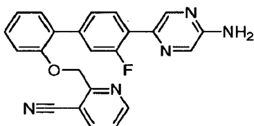
2-({[4'-(5-Aminopyrazin-2-yl)-3'-fluorobiphenyl-2-yl]oxy}methyl)pyridine-3-carbonitrile
