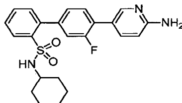
4'-(6-Aminopyridin-3-yl)-N-cyclohexyl-3'-fluoro-[1,1'-biphenyl]-2-sulfonamide
