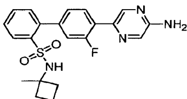
4'-(5-Aminopyrazin-2-yl)-3'-fluoro-N-(1-methylcyclobutyl)biphenyl-2-sulfonamide
