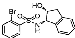
2-Bromo- N -[(1 S ,2 R )-2-hydroxy-2,3-dihydro-1 H -inden-1-yl]benzenesulfonamide
