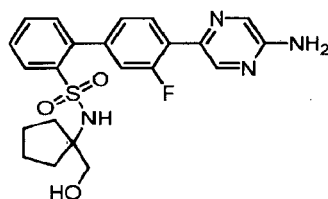
4'-(5-Aminopyrazin-2-yl)-3'-fluoro-N-[1-(hydroxymethyl)cyclopentyl]biphenyl-2-sulfonamide
