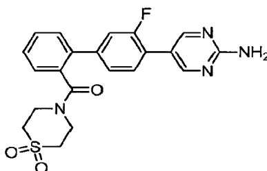
5-{2'-[(1,1-Dioxidothiomorpholin-4-yl)carbonyl]-3-fluorobiphenyl-4-yl}pyrimidin-2-amine
