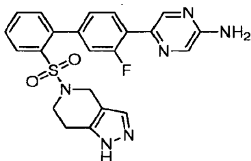
5-[3-Fluoro-2'-(1,4,6,7-tetrahydro-5H-pyrazolo[4,3-c]pyridin-5-ylsulfonyl)biphenyl-4-yl]pyrazin-2-amine
