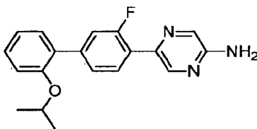
5-[3-Fluoro-2'-(1-methylethoxy)biphenyl-4-yl]pyrazin-2-amine
