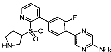
racemic 5-(2-Fluoro-4-(2-(pyrrolidin-3-yl)sulfonyl)pyridin-3-yl)phenyl)pyrazin-2-amine hydrochloride
