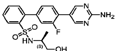
4'-(2-Aminopyrimidin-5-yl)-3'-fluoro- N -[(1 S )-2-hydroxy-1-methylethyl]biphenyl-2-sulfonamide trifluoroacetic acid salt
