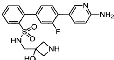
4'-((6-Aminopyridin-3-yl)-3'-fluoro-N-((3-hydroxyazetidin-3-yl)methyl)-[1,1'-biphenyl]-2-sulfonamide
