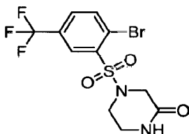
4-((2-Bromo-5-(trifluoromethyl)phenyl)sulfonyl)piperazin-2-one.
