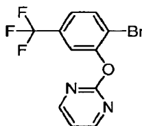
2-(2-Bromo-5-(trifluoromethyl)phenoxy)pyrimidine
