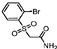
2-((2-Bromophenyl)sulfonyl)acetamide
