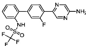
[4'-(5-Aminopyrazin-2-yl)-3'-fluorobiphenyl-2-yl]-1,1,1-trifluoromethanesulfonamide
