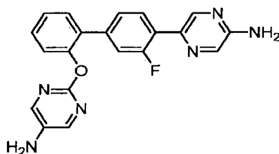
2-{{4'-(5-Aminopyrazin-2-yl)-3'-fluorobiphenyl-2-yl}oxy}pyrimidin-5-amine.
