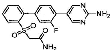
2-[[4'-(2-Aminopyrimidin-5-yl)-3'-fluorobiphenyl-2-yl]sulfonyl]acetamide.
