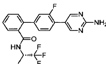
4'-(2-Aminopyrimidin-5-yl)-3'-fluoro- N -[(1 S )-2,2,2-trifluoro-1-methylethyl]biphenyl-2-carboxamide
