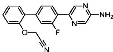
{[4'-(5-Aminopyrazin-2-yl)-3'-fluorobiphenyl-2-yl]oxy}acetonitrile.
