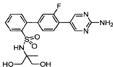
4'-(2-Aminopyrimidin-5-yl)-3'-fluoro- N -[2-hydroxy-1-(hydroxymethyl)-1-methylethyl]biphenyl-2-sulfonamide
