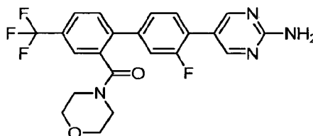
5-[3-Fluoro-2'-(morpholin-4-ylcarbonyl)-4'-(trifluoromethyl)biphenyl-4-yl]pyrimidin-2-amine
