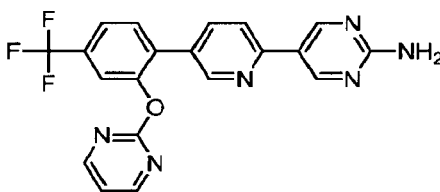
5-{5-[2-(Pyrimidin-2-yloxy)-4-(trifluoromethyl)phenyl]pyridin-2-yl}pyrimidin-2-amine
