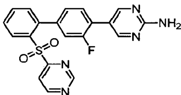
5-[3-fluoro-2'-(pyrimidin-4-ylsulfonyl)biphenyl-4-yl]pyrimidin-2-amine
