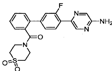
5-{2'-[(1;1-Dioxidothiomorpholin-4-yl)carbonyl]-3'-fluorobiphenyl-4-yl}pyrazin-2-amine
