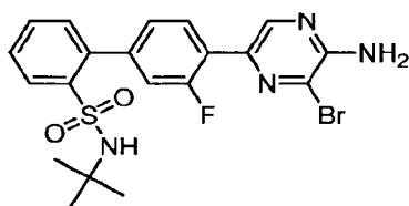
4'-(5-Amino-6-bromopyrazin-2-yl)- N - tert -butyl-3'-fluorobiphenyl-2-sulfonamide
