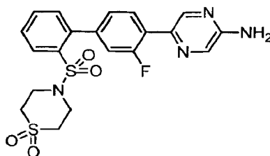
5-{2'-[(1,1-Dioxidothiomorpholin-4-yl)sulfonyl]-3-fluorobiphenyl-4-yl}pyrazin-2-amine
