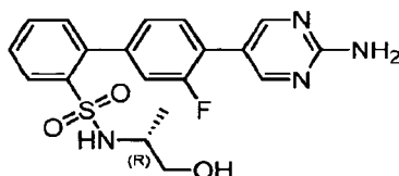
4'-(2-Aminopyrimidin-5-yl)-3'-fluoro-N-[(1R)-2-hydroxy-1-methylethyl]biphenyl-2-sulfonamide
