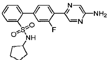
4'-(5-Aminopyrazin-2-yl)- N -cyclopentyl-3'-fluorobiphenyl-2-sulfonamide
