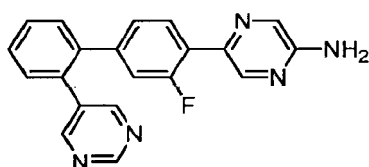
5-((3-Fluoro-2'-pyrimidin-5-yl)biphenyl-4-yl)pyrazin-2-amine.
