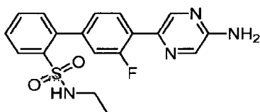
4'-(5-Aminopyrazin-2-yl)-N-ethyl-3'-fluorobiphenyl-2-sulfonamide
