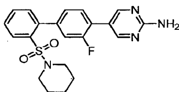
5-[3-Fluoro-2'-(piperidin-1-ylsulfonyl)biphenyl-4-yl]pyrimidin-2-amine trifluoroacetic acid salt
