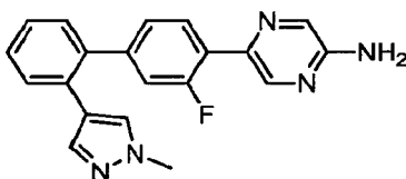
5-[3-Fluoro-2'-(1-methyl-1H-pyrazol-4-yl)biphenyl-4-yl]pyrazin-2-amine.
