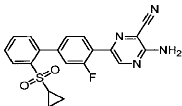
3-Amino-6-[2'-(cyclopropylsulfonyl)-3-fluorobiphenyl-4-yl]pyrazine-2-carbonitrile
