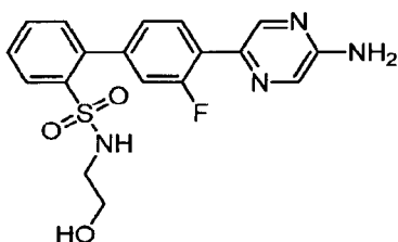
4'-(5-Aminopyrazin-2-yl)-3'-fluoro-N-(2-hydroxyethyl)biphenyl-2-sulfonamide
