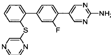
5-[3-Fluoro-2'-(pyrazin-2-ylsulfanyl)biphenyl-4-yl]pyrimidin-2-amine hydrochloride
