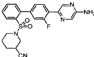
racemic 1-[[4'-(5-Aminopyrazin-2-yl)-3'-fluorobiphenyl-2-yl]sulfonyl]piperidine-3-carbonitrile
