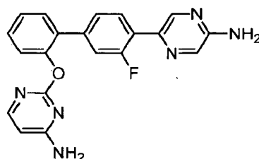
2-{{4'-(5-Aminopyrazin-2-yl)-3'-fluorobiphenyl-2-yl}oxy}pyrimidin-4-amine
