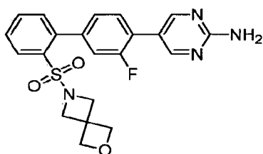
5-(2'-(2-Oxa-6-azaspiro[3.3]heptan-6-ylsulfonyl)-3-fluoro-[1,1'-biphenyl]-4-yl)pyrimidin-2-amine
