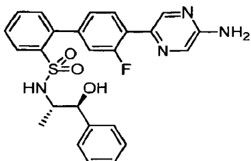
4'-(5-Aminopyrazin-2-yl)-3'-fluoro- N -[(1 S ,2 R )-2-hydroxy-1-methyl-2-phenylethyl]biphenyl-2-sulfonamide
