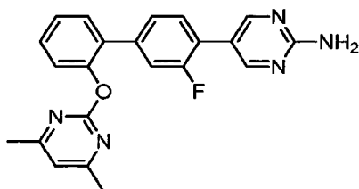
5-{2'-[(4,6-Dimethylpyrimidin-2-yl)oxy]-3-fluorobiphenyl-4-yl}pyrimidin-2-amine.
