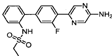
N -[4'-(5-Aminopyrazin-2-yl)-3'-fluorobiphenyl-2-yl]ethanesulfonamide
