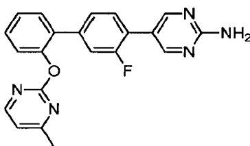
5-{3-Fluoro-2'-[(4-methylpyrimidin-2-yl)oxy]biphenyl-4-yl}pyrimidin-2-amine
