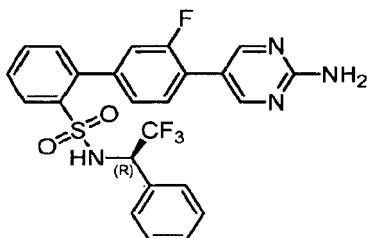
4'-(2-Aminopyrimidin-5-yl)-3'-fluoro-N-[(1 R )-2,2,2-trifluoro-1-phenylethyl]biphenyl-2-sulfonamide trifluoroacetic acid salt
