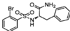
N -α-[(2-Bromophenyl)sulfonyl]-L-phenylalaninamide
