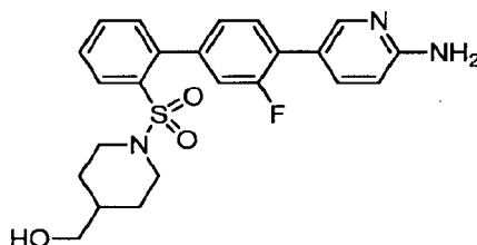
(1-((4'-(6-Aminopyridin-3-yl)-3'-fluoro-[1,1'-biphenyl]-2-yl)sulfonyl)piperidin-4-yl)methanol
