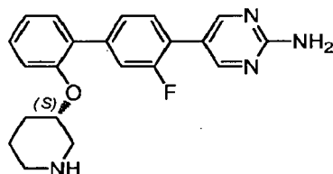
5-{3-Fluoro-2'-[(3 S )-piperidin-3-yloxy]biphenyl-4-yl}pyrimidin-2-amine.
