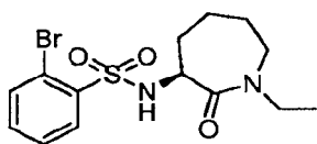
2-Bromo-N-[(3S)-1-ethyl-2-oxazepan-3-yl]benzenesulfonamide
