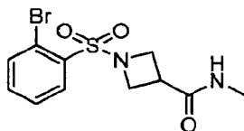
1-((2-Bromophenyl)sulfonyl)-N-methylazetidine-3-carboxamide
