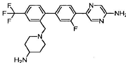
5-{2'-[(4-Aminopiperidin-1-yl)methyl]-3-fluoro-4'-(trifluoromethyl)biphenyl-4-yl}pyrazin-2-amine.
