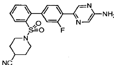
1-[[4'-(5-Aminopyrazin-2-yl)-3'-fluorobiphenyl-2-yl]sulfonyl]piperidine-4-carbonitrile
