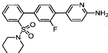
5-(3-Fluoro-2'-(piperidin-1-ylsulfonyl)-[1,1'-biphenyl]-4-yl)pyridin-2-amine
