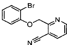
2-((2-Bromophenoxy)methyl)nicotinonitrile
