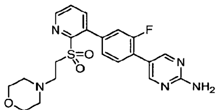
5-(2-Fluoro-4-(2-((2-morpholinoethyl)sulfonyl)pyridine-3-yl)phenyl)pyrimidin-2-amine formic acid salt.
