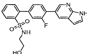
3'-Fluoro-N-(2-hydroxyethyl)-4'-(1H-pyrrolo[2,3-b]pyridin-5-yl)biphenyl-2-sulfonamide
