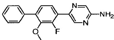
5-(3-Fluoro-2-methoxybiphenyl-4-yl)pyrazin-2-amine.
