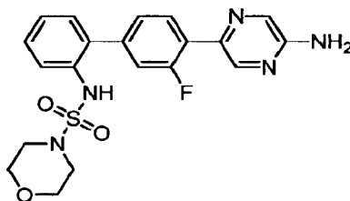
N -[4'-(5-Aminopyrazin-2-yl)-3'-fluorobiphenyl-2-yl]morpholine-4-sulfonamide
