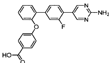
4-([4'-(2-Aminopyrimidin-5-yl)-3'-fluorobiphenyl-2-yl]oxy)benzoic acid.
