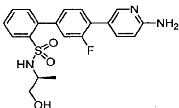
(S)-4'-(6-Aminopyridin-3-yl)-3'-fluoro-N-(1-hydroxypropan-2-yl)-[1,1'-biphenyl]-2-sulfonamide
