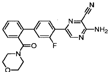
3-Amino-6-[3-fluoro-2'-(morpholin-4-ylcarbonyl)biphenyl-4-yl]pyrazine-2-carbonitrile
