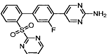
5-(3-Fluoro-2'-(pyrimidin-2-ylsulfonyl)biphenyl-4-yl)pyrimidin-2-amine
