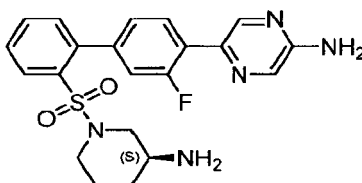
(S)-5-{2'-[(3-Aminopiperidin-1-yl)sulfonyl]-3-fluorobiphenyl-4-yl}pyrazin-2-amine
