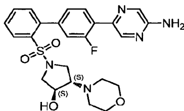
Racemic-1-([4'-(5-Aminopyrazin-2-yl)-3'-fluorobiphenyl-2-yl]sulfonyl)-4-morpholin-4-ylpyrrolidin-3-ol trifluoroacetic acid salt
