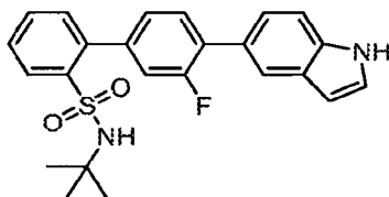
N -tert-Butyl-3'-fluoro-4'-(1 H -indol-5-yl)biphenyl-2-sulfonamide
