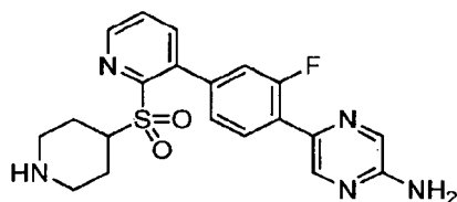
5-{2-Fluoro-4-[2-(piperidin-4-ylsulfonyl)pyridin-3-yl]phenyl}pyrazin-2-amine hydrochloride
