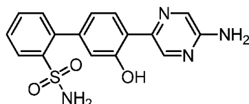
4'-(5-Aminopyrazin-2-yl)-3'-hydroxybiphenyl-2-sulfonamide.
