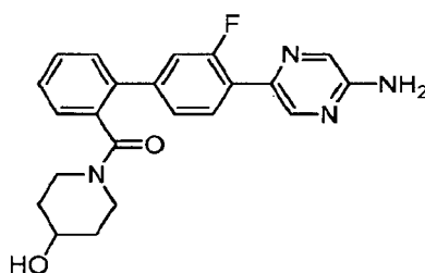
1-[(4'-(5-Aminopyrazin-2-yl)-3'-fluorobiphenyl-2-yl)carbonyl]piperidin-4-ol
