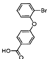
4-(2-Bromophenoxy)benzoic acid
