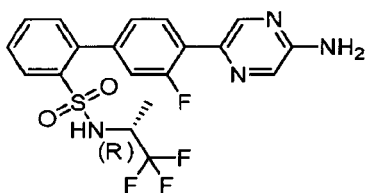
(R)-4'-(5-Aminopyrazin-2-yl)-3'-fluoro-N-(2,2,2-trifluoro-1-methylethyl)biphenyl-2-sulfonamide
