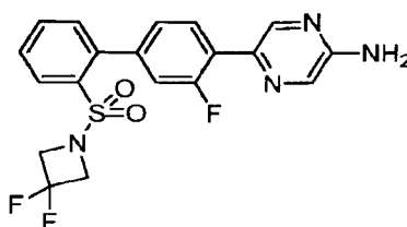
5-{2'-[(3,3-Difluoroazetidin-1-yl)sulfonyl]-3-fluorobiphenyl-4-yl}pyrazin-2-amine
