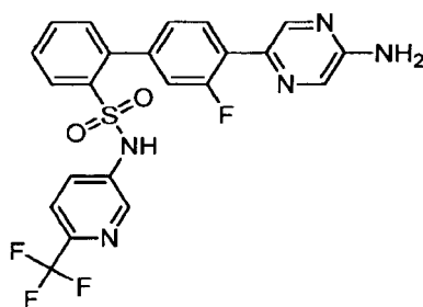
4'-(5-Aminopyrazin-2-yl)-3'-fluoro-N-[6-(trifluoromethyl)pyridin-3-yl]biphenyl-2-sulfonamide
