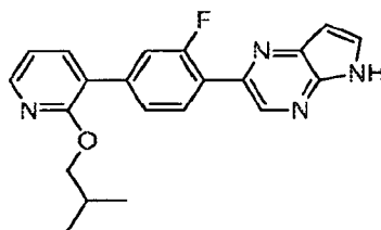
2-{2-Fluoro-4-[2-(2-methylpropoxy)pyridin-3-yl]phenyl}-5H-pyrrolo[2,3-b]pyrazine
