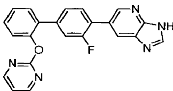
6-{3-Fluoro-2'-(pyrimidin-2-yloxy)biphenyl-4-yl}-3H-imidazo[4,5-b]pyridine
