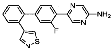
5-(3-Fluoro-2'-isothiazol-4-ylbiphenyl-4-yl)pyrazin-2-amine.
