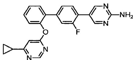
5-{2'-[(6-Cyclopropylpyrimidin-4-yl)oxy]-3-fluorobiphenyl-4-yl}pyrimidin-2-amine.
