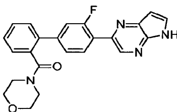
2-[3-Fluoro-2'-(morpholin-4-ylcarbonyl)biphenyl-4-yl]-5H-pyrrolo[2,3-b]pyrazine
