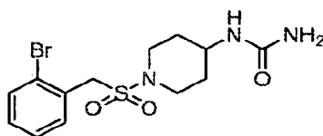
1-(1-((2-Bromobenzyl)sulfonyl)piperidin-4-yl)urea
