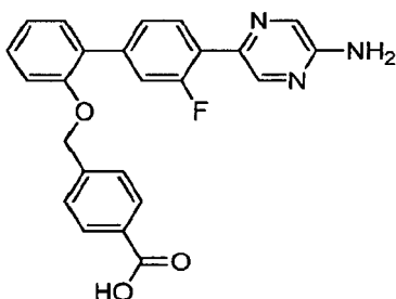
4-({[4'-(5-Aminopyrazin-2-yl)-3'-fluorobiphenyl-2-yl]oxy}methyl)benzoic acid.
