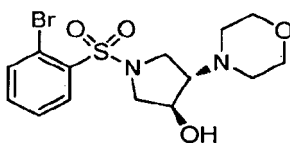
Racemic 1-((2-Bromophenyl)sulfonyl)-4-morpholinopyrrolidin-3-ol.
