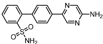
4'-(5-Aminopyrazin-2-yl)biphenyl-2-sulfonamide.
