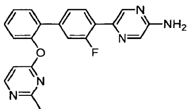
5-{3-Fluoro-2'-[(2-methylpyrimidin-4-yl)oxy]biphenyl-4-yl}pyrazin-2-amine
