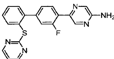
5-[3-Fluoro-2'-(pyrimidin-2-ylsulfanyl)biphenyl-4-yl]pyrazin-2-amine hydrochloride
