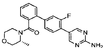
5-(3-Fluoro-2'--[(3R)-3-methylmorpholin-4-yl]carbonyl)biphenyl-4-yl)pyrimidin-2-amine
