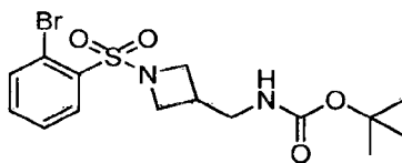
tert -Butyl ((1-((2-bromophenyl)sulfonyl)azetidin-3-yl)methyl)carbamate
