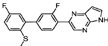
2-[3,5'-Difluoro-2'-(methylsulfanyl)biphenyl-4-yl]-5H-pyrrolo[2,3-b]pyrazine
