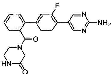
4-{{4'-(2-Aminopyrimidin-5-yl)-3'-fluorobiphenyl-2-yl}carbonyl}piperazin-2-one
