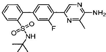
4'-(5-Amino-6-methylpyrazin-2-yl)- N - tert -butyl-3'-fluorobiphenyl-2-sulfonamide
