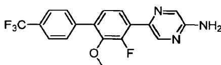
5-(3-fluoro-2-methoxy-4'-(trifluoromethyl)-[1,1'-biphenyl]-4-yl)pyrazin-2-amine.
