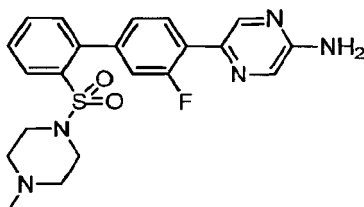
5-{3-Fluoro-2'-[4-methylpiperazin-1-yl]sulfonyl}biphenyl-4-yl}pyrazin-2-amine
