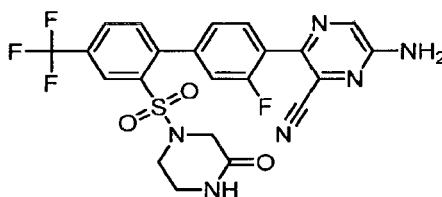
6-Amino-3-{3-fluoro-2'-[(3-oxopiperazin-1-yl)sulfonyl]-4'-(trifluoromethyl)biphenyl-4-yl}pyrazine-2-carbonitrile
