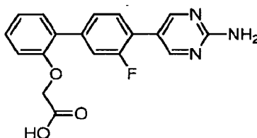
{[4'-(2-Aminopyrimidin-5-yl)-3'-fluorobiphenyl-2-yl]oxy}acetic acid.
