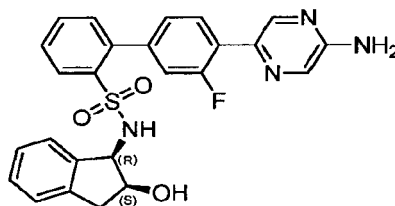
4'-(5-Aminopyrazin-2-yl)-3'-fluoro- N -((1 R ,2 S )-2-hydroxy-2,3-dihydro-1 H -inden-1-yl)-[1,1'-biphenyl]-2-sulfonamide
