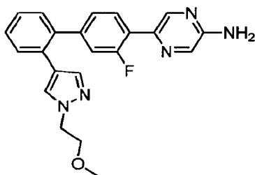
5-[3-Fluoro-2'-[1-(2-methoxyethyl)-1H-pyrazol-4-yl]biphenyl-4-yl]pyrazin-2-amine.
