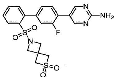
6-((4'-(2-Aminopyrimidin-5-yl)-3'-fluoro-[1,1'-biphenyl]-2-yl)sulfonyl)-2-thia-6-azaspiro[3.3]heptane 2,2-dioxide
