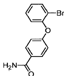
4-(2-Bromophenoxy)benzamide
