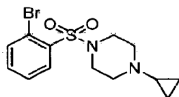
1-((2-Bromophenyl)sulfonyl)-4-cyclopropylpiperazine.
