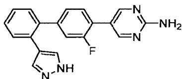
5-[3-Fluoro-2'-(1H-pyrazol-4-yl)biphenyl-4-yl]pyrimidin-2-amine.
