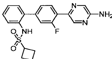
N -(4'-(5-Aminopyrazin-2-yl)-3'-fluoro-[1,1'-biphenyl]-2-yl)cyclobutanesulfonamide
