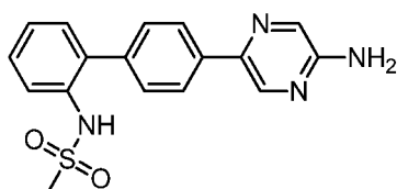
N -[4'-(5-Aminopyrazin-2-yl)biphenyl-2-yl]methanesulfonamide.
