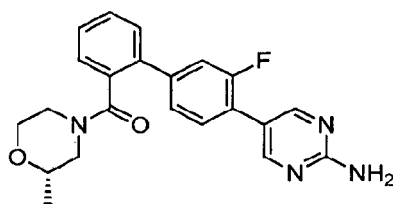
5-(3-Fluoro-2'--[(2S)-2-methylmorpholin-4-yl]carbonyl)biphenyl-4-yl)pyrimidin-2-amine
