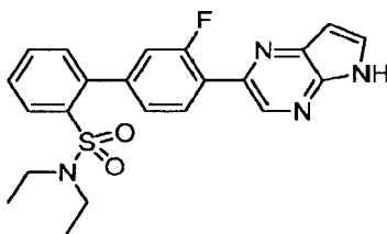
N,N -Diethyl-3'-fluoro-4'-(5 H -pyrrolo[2,3- b ]pyrazin-2-yl)biphenyl-2-sulfonamide
