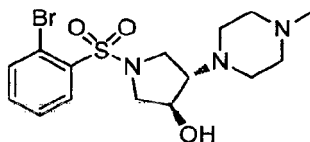
Racemic-1-((2-Bromophenyl)sulfonyl)-4-(4-methylpiperazin-1-yl)pyrrolidin-3-ol.
