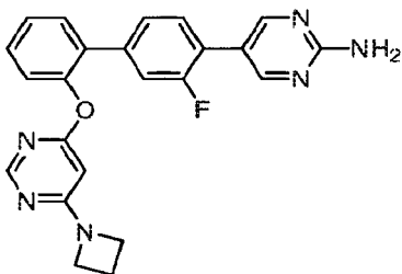
5-{2'-[(6-Azetidin-1-ylpyrimidin-4-yl)oxy]-3-fluorobiphenyl-4-yl}pyrimidin-2-amine
