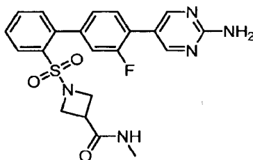
1-([4'-(2-Aminopyrimidin-5-yl)-3'-fluorobiphenyl-2-yl]sulfonyl)-N-methylazetidine-3-carboxamide
