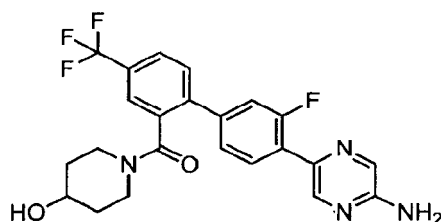
[2-[4-(5-Aminopyrazin-2-yl)-3-fluoro-phenyl]-5-(trifluoromethyl)phenyl]-(4-hydroxy-1-piperidyl)methanone
