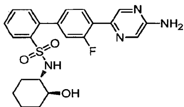
Racemic-( trans )-4'-(5-Aminopyrazin-2-yl)-3'-fluoro- N -(2-hydroxycyclohexyl)biphenyl-2-sulfonamide
