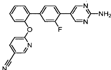
6-{{4'-(2-Aminopyrimidin-5-yl)-3'-fluorobiphenyl-2-yl}oxy}pyridine-3-carbonitrile.
