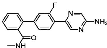
4'-(5-Aminopyrazin-2-yl)-3'-fluoro-N-methylbiphenyl-2-carboxamide
