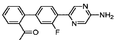
1-[4'-(5-Aminopyrazin-2-yl)-3'-fluorobiphenyl-2-yl]ethanone
