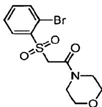
2-((2-Bromophenyl)sulfonyl)-1-morpholinoethanone
