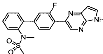
N -[3'-Fluoro-4'-(5 H -pyrrolo[2,3- b ]pyrazin-2-yl)biphenyl-2-yl]- N -methylmethanesulfonamide
