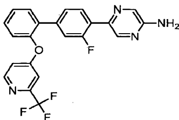
5-(3-Fluoro-2'-[2-(trifluoromethyl)pyridin-4-yl]oxy)biphenyl-4-yl}pyrazin-2-amine.
