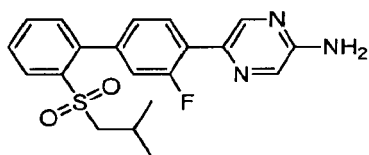
5-{3-Fluoro-2'-[(2-methylpropyl)sulfonyl]biphenyl-4-yl}pyrazin-2-amine
