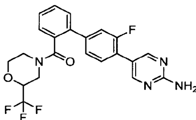
racemic 5-(3-Fluoro-2'-[2-(trifluoromethyl)morpholin-4-yl]carbonyl)biphenyl-4-yl)pyrimidin-2-amine
