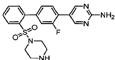
5-[3-Fluoro-2'-(piperazin-1-ylsulfonyl)biphenyl-4-yl]pyrimidin-2-amine trifluoroacetic acid salt
