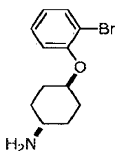
trans 4-(2-Bromophenoxy)cyclohexanamine
