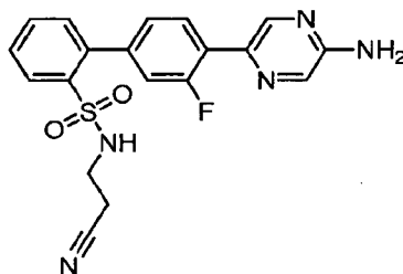
4'-(5-Aminopyrazin-2-yl)-N-(2-cyanoethyl)-3'-fluorobiphenyl-2-sulfonamide
