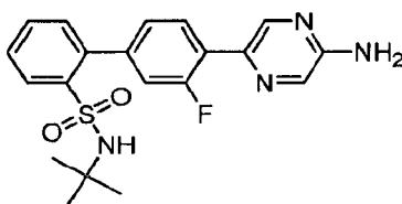
4'-(5-Aminopyrazin-2-yl)- N -tert-butyl-3'-fluorobiphenyl-2-sulfonamide
