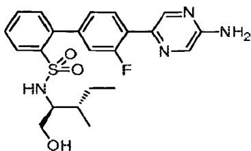
4'-(5-Aminopyrazin-2-yl)-3'-fluoro- N -[(1 S ,2 S )-1-(hydroxymethyl)-2-methylbutyl]biphenyl-2-sulfonamide
