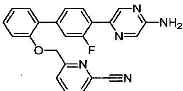
6-({[4'-(5-Aminopyrazin-2-yl)-3'-fluorobiphenyl-2-yl]oxy}methyl)pyridine-2-carbonitrile
