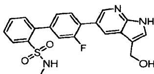
3'-Fluoro-4'-[3-(hydroxymethyl)-1 H -pyrrolo[2,3- b ]pyridin-5-yl]- N -methylbiphenyl-2-sulfonamide
