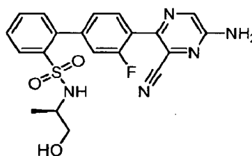
4'-(5-Amino-3-cyanopyrazin-2-yl)-3'-fluoro- N -[(1 R )-2-hydroxy-1-methylethyl]biphenyl-2-sulfonamide
