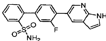
3'-Fluoro-4'-(1H-pyrrolo[2,3-b]pyridin-5-yl)biphenyl-2-sulfonamide
