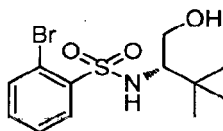
2-Bromo- N -[(1 S )-1-(hydroxymethyl)-2,2-dimethylpropyl]benzenesulfonamide
