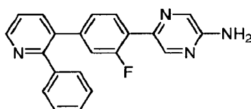
5-[2-Fluoro-4-(2-phenylpyridin-3-yl)phenyl]pyrazin-2-amine,
