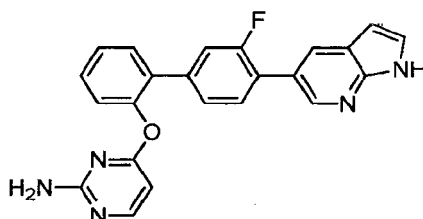
4-[[3'-Fluoro-4'-(1H-pyrrolo[2,3-b]pyridin-5-yl)biphenyl-2-yl]oxy]pyrimidin-2-amine
