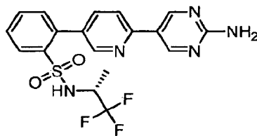
2-[6-(2-Aminopyrimidin-5-yl)pyridin-3-yl]- N -[(1 R )-2,2,2-trifluoro-1-methylethyl]benzenesulfonamide trifluoroacetic acid salt.
