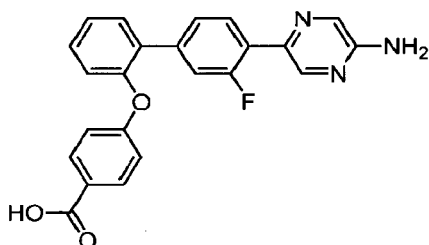
4-([4'-(5-Aminopyrazin-2-yl)-3'-fluorobiphenyl-2-yl]oxy)benzoic acid
