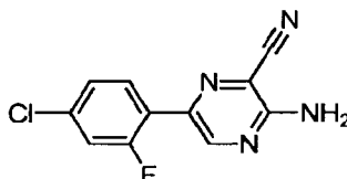
3-Amino-6-(4-chloro-2-fluorophenyl)pyrazine-2-carbonitrile
