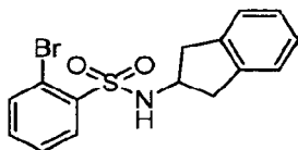
2-Bromo- N -(2,3-dihydro-1 H -inden-2-yl)benzenesulfonamide
