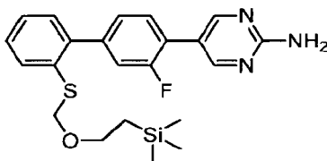
5-[3-Fluoro-2'-{[2-(trimethylsilyl)ethoxy]methyl}sulfanyl]biphenyl-4-yl]pyrimidin-2-amine
