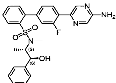
4'-({5-aminopyrazin-2-yl}-3'-fluoro- N -((1 S ,2 S )-1-hydroxy-1-phenylpropan-2-yl)- N -methyl-[1,1'-biphenyl]-2-sulfonamide
