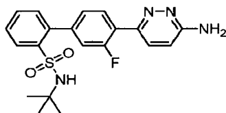
4'-(6-Aminopyridazin-3-yl)-N-tert-butyl-3'-fluorobiphenyl-2-sulfonamide
