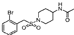
N-(1-((2-Bromobenzyl)sulfonyl)piperidin-4-yl)acetamide
