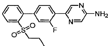
5-[3-Fluoro-2'-(propylsulfonyl)biphenyl-4-yl]pyrazin-2-amine
