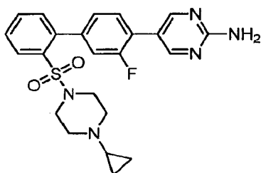
5-({2'-[(4-Cyclopropylpiperazin-1-yl)sulfonyl]-3-fluorobiphenyl-4-yl})pyrimidin-2-amine trifluoroacetic acid salt
