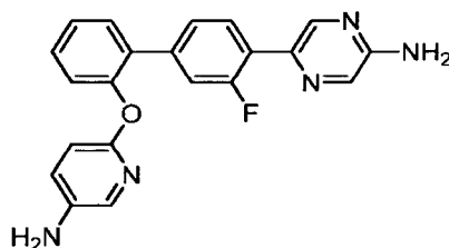
5-{2'-[(5-Aminopyridin-2-yl)oxy]-3-fluorobiphenyl-4-yl}pyrazin-2-amine.
