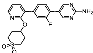
5-(4-{2-[(1,1-Dioxido-2H-thiopyran-4-yl)oxy]pyridin-3-yl}-2-fluorophenyl)pyrimidin-2-amine.
