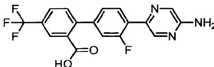
4'-(5-Aminopyrazin-2-yl)-3'-fluoro-4-(trifluoromethyl)biphenyl-2-carboxylic acid.
