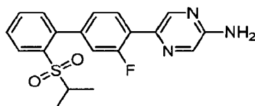
5-{3-Fluoro-2'-[(1-methylethyl)sulfonyl]biphenyl-4-yl}pyrazin-2-amine
