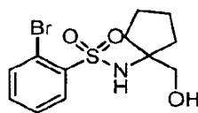
2-Bromo-N-(1-(hydroxymethyl)cyclopentyl)benzenesulfonamide.
