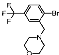
4-(2-Bromo-5-(trifluoromethyl)benzyl)morpholine
