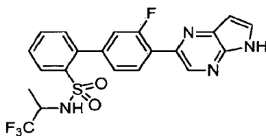
racemic 3'-Fluoro-4'-(5H-pyrrolo[2,3-b]pyrazin-2-yl)-N-(2,2,2-trifluoro-1-methylethyl)biphenyl-2-sulfonamide
