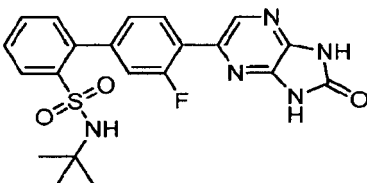
N -tert-Butyl-3'-fluoro-4'-(2-oxo-2,3-dihydro-1 H -imidazo[4,5- b ]pyrazin-5-yl)biphenyl-2-sulfonamide
