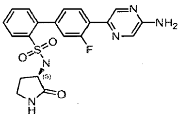
(S)-4'-(5-Aminopyrazin-2-yl)-3'-fluoro-N-(2-oxopyrrolidin-3-yl)-[1,1'-biphenyl]-2-sulfonamide
