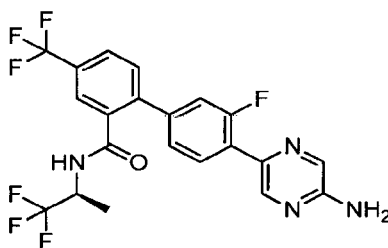
2-[4-(5-Aminopyrazin-2-yl)-3-fluoro-phenyl]-5-(trifluoromethyl)-N-[(1S)-2,2,2-trifluoro-1-methyl-ethyl]benzamide
