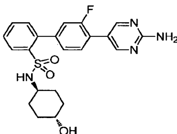
4'-(2-Aminopyrimidin-5-yl)-3'-fluoro-N-(trans-4-hydroxycyclohexyl)biphenyl-2-sulfonamide
