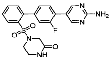
4'-((2-Aminopyrimidin-5-yl)-3'-fluorobiphenyl-2-yl)sulfonyl)piperazin-2-one trifluoroacetic acid salt
