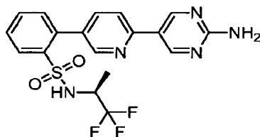
2-[6-(2-Aminopyrimidin-5-yl)pyridin-3-yl]- N -[(1 S )-2,2,2-trifluoro-1-methylethyl]benzenesulfonamide trifluoroacetic acid salt.
