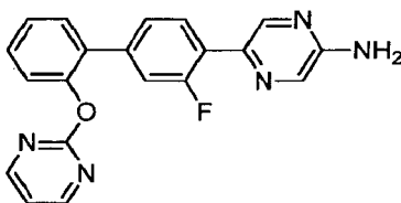
5-[3-Fluoro-2'-(pyrimidin-2-yloxy)biphenyl-4-yl]pyrazin-2-amine
