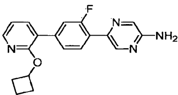
5-[4-[2-(Cyclobutyloxy)pyridin-3-yl]-2-fluorophenyl]pyrazin-2-amine
