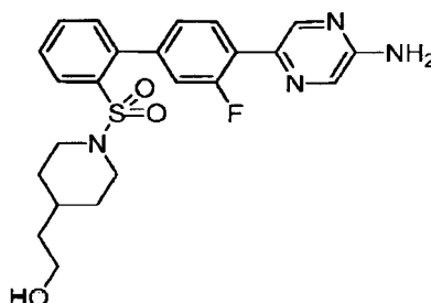
2-(1-([4'-(5-Aminopyrazin-2-yl)-3'-fluorobiphenyl-2-yl]sulfonyl)piperidin-4-yl)ethanol
