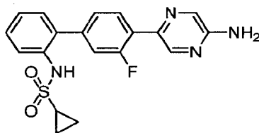
N -(4'-(5-aminopyrazin-2-yl)-3'-fluoro-[1,1'-biphenyl]-2-yl)cyclopropanesulfonamide
