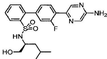
4'-(5-Aminopyrazin-2-yl)-3'-fluoro- N -[(1 S )-1-(hydroxymethyl)-3-methylbutyl]biphenyl-2-sulfonamide
