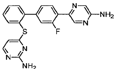
4-[[4'-(5-Aminopyrazin-2-yl)-3'-fluorobiphenyl-2-yl]sulfanyl]pyrimidin-2-amine hydrochloride
