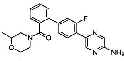
5-([2'-(2,6-Dimethylmorpholin-4-yl)carbonyl]-3-fluorobiphenyl-4-yl)pyrazin-2-amine (diastereoisomeric mixture).
