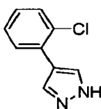
4-(2-Chlorophenyl)-1H-pyrazole
