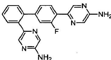
5,5'-(3'-Fluorobiphenyl-2,4'-diyl)dipyrazin-2-amine.
