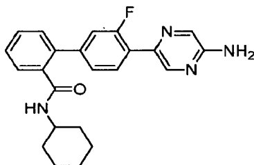
4'-{(5-Aminopyrazin-2-yl)-N-cyclohexyl-3'-fluorobiphenyl-2-carboxamide
