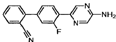
4'-(5-Aminopyrazin-2-yl)-3'-fluorobiphenyl-2-carbonitrile
