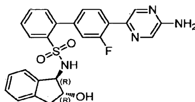
4'-(5-Aminopyrazin-2-yl)-3'-fluoro- N -((1 R ,2 R )-2-hydroxy-2,3-dihydro-1 H -inden-1-yl)-[1,1'-biphenyl]-2-sulfonamide
