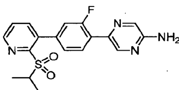
5-(2-Fluoro-4-{2-[(1-methylethyl)sulfonyl]pyridin-3-yl}phenyl)pyrazin-2-amine
