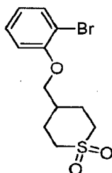
4-((2-Bromophenoxy)methyl)tetrahydro-2 H -thiopyran 1,1-dioxide
