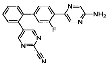
5-((4'-(5-Aminopyrazin-2-yl)-3'-fluorobiphenyl-2-yl)pyrimidine-2-carbonitrile.
