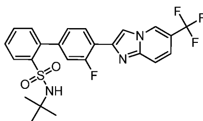
N -tert-Butyl-3'-fluoro-4'-[6-(trifluoromethyl)imidazo[1,2-a]pyridin-2-yl]biphenyl-2-sulfonamide
