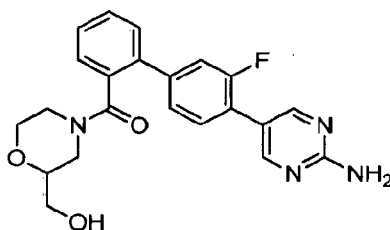
racemic [2-{4-(2-Aminopyrimidin-5-yl)-3-fluoro-phenyl}phenyl]-[2-(hydroxymethyl)morpholin-4-yl]methanone
