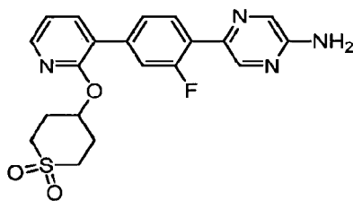
5-(4-{2-[(1,1-Dioxido-2H-thiopyran-4-yl)oxy]pyridin-3-yl}-2-fluorophenyl)pyrazin-2-amine.
