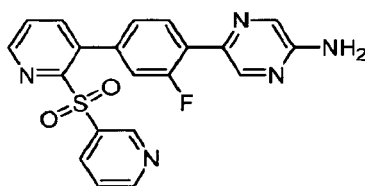
5- \{2\text{-Fluoro-4-[2-(pyridin-3-ylsulfonyl)pyridin-3-yl]phenyl}\} pyrazin-2-amine.
