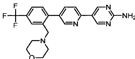
5-[5-[2-(Morpholin-4-ylmethyl)-4-(trifluoromethyl)phenyl]pyridin-2-yl]pyrimidin-2-amine.
