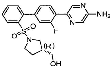
(R) -(1-((4'-(5-Aminopyrazin-2-yl)-3'-fluoro-[1,1'-biphenyl]-2-yl)sulfonyl)pyrrolidin-3-yl)methanol
