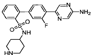
4'-(5-Aminopyrazin-2-yl)-3'-fluoro-N-piperidin-4-ylbiphenyl-2-sulfonamide
