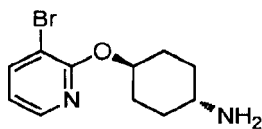
trans -4-((3-bromopyridin-2-yl)oxy)cyclohexanamine
