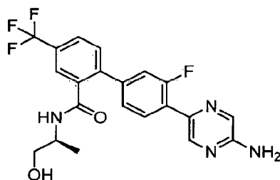
2-[4-(5-Aminopyrazin-2-yl)-3-fluoro-phenyl]-N-[(1 S )-2-hydroxy-1-methyl-ethyl]-5-(trifluoromethyl)benzamide
