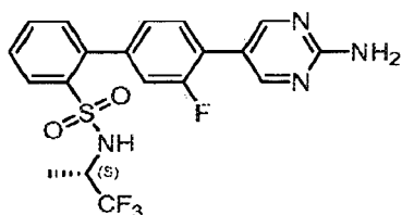
4'-(2-Aminopyrimidin-5-yl)-3'-fluoro-N-[(1S)-2,2,2-trifluoro-1-methylethyl]biphenyl-2-sulfonamide trifluoroacetic acid salt
