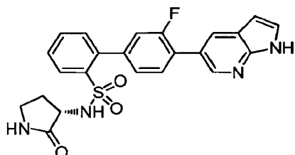
3'-Fluoro- N -[(3 S )-2-oxopyrrolidin-3-yl]-4'-(1 H -pyrrolo[2,3- b ]pyridin-5-yl)biphenyl-2-sulfonamide
