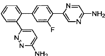
6-[4'-(5-Aminopyrazin-2-yl)-3'-fluorobiphenyl-2-yl]pyridazin-3-amine. #55495609#
