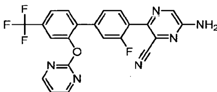
6-Amino-3-[3-fluoro-2'-(pyrimidin-2-yloxy)-4'-(trifluoromethyl)biphenyl-4-yl]pyrazine-2-carbonitrile
