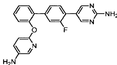
5-{2'-[(5-Aminopyridin-2-yl)oxy]-3-fluorobiphenyl-4-yl}pyrimidin-2-amine.
