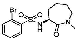
2-Bromo-N-[(3S)-1-methyl-2-oxazepan-3-yl]benzenesulfonamide
