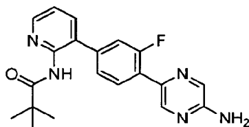
N -{3-[4-(5-Aminopyrazin-2-yl)-3-fluorophenyl]pyridin-2-yl}-2,2-dimethylpropanamide
