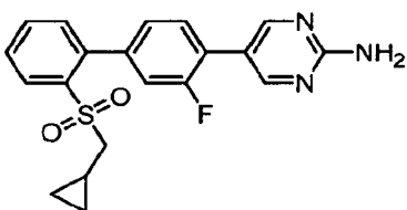
5-(2'-[(Cyclopropylmethyl)sulfonyl]-3-fluorobiphenyl-4-yl)pyrimidin-2-amine
