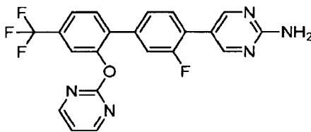
5-[3-Fluoro-2'-(pyrimidin-2-yloxy)-4'-(trifluoromethyl)biphenyl-4-yl]pyrimidin-2-amine
