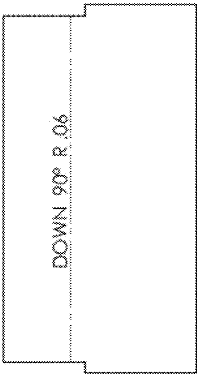
FLAT PATTERN
