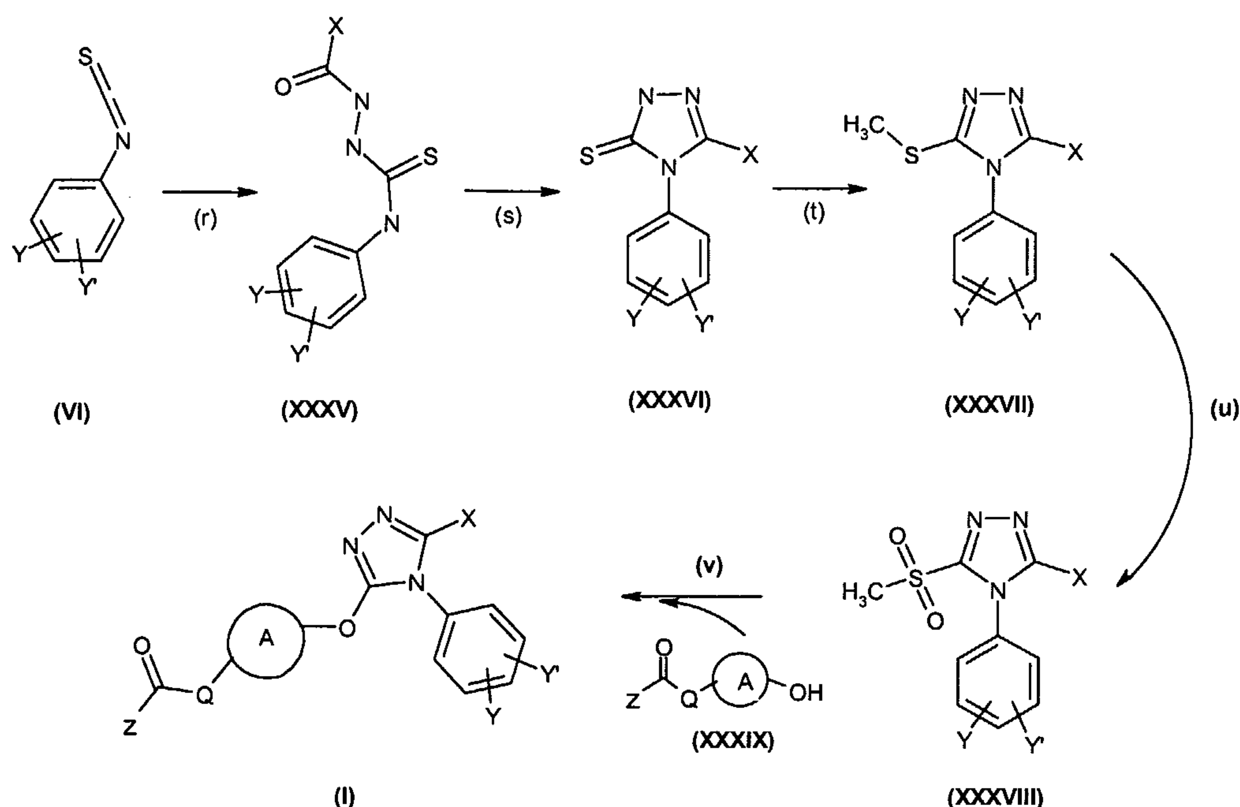
Scheme 12
