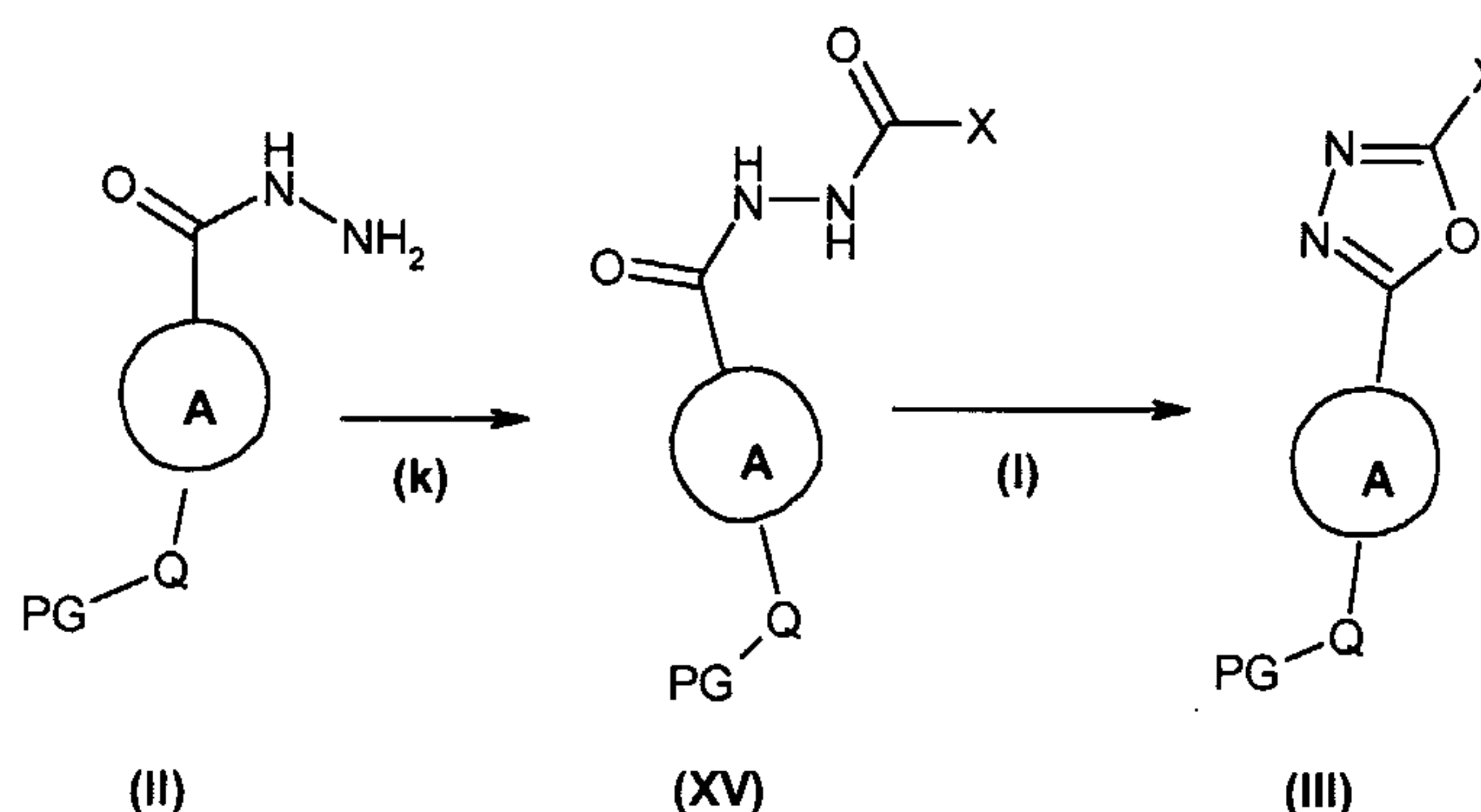
Scheme 5.
