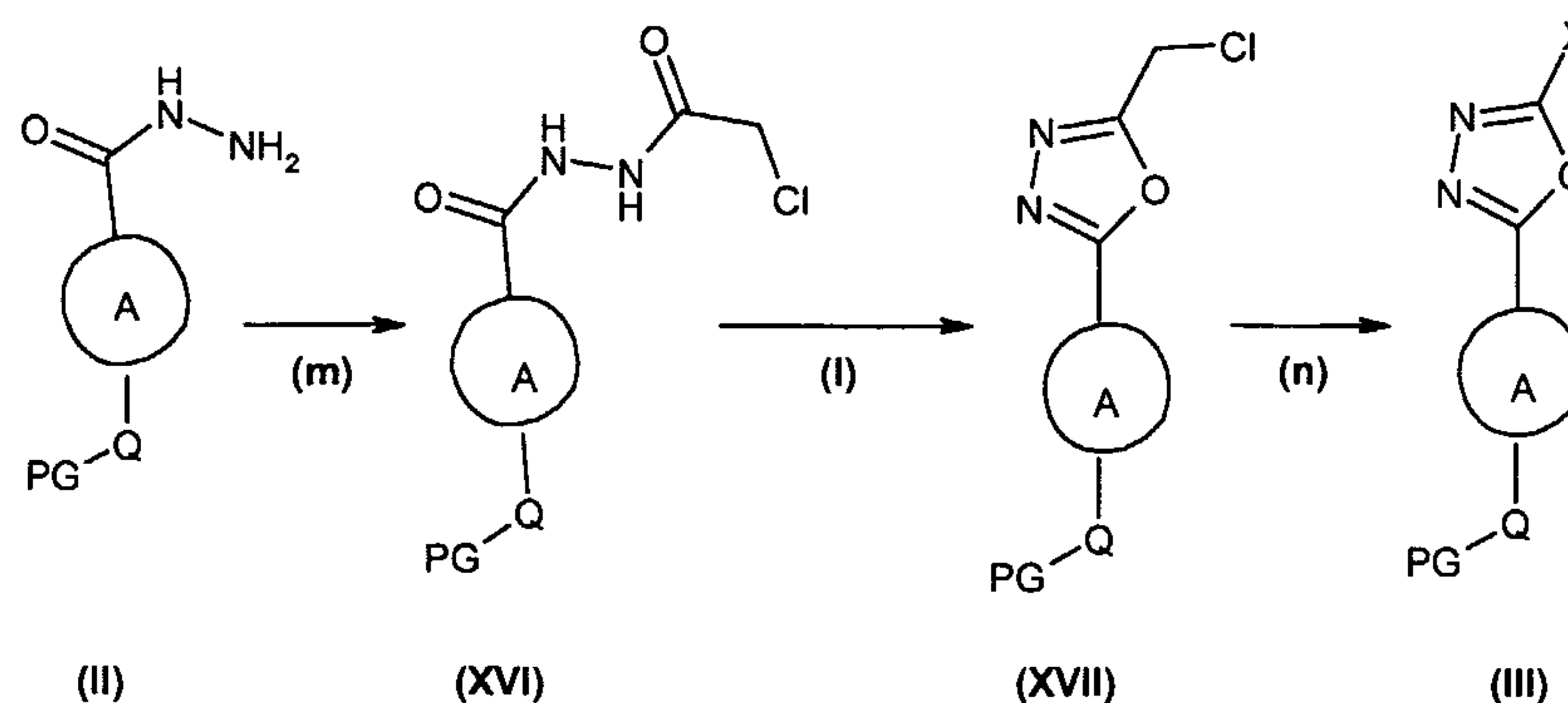
Scheme 6
