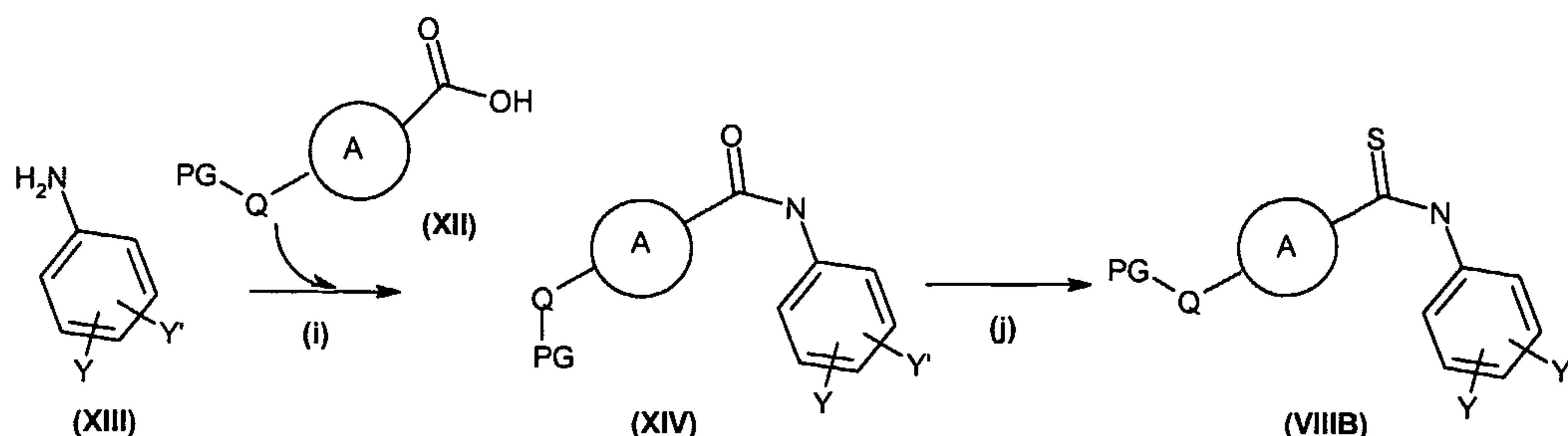
Scheme 4.
