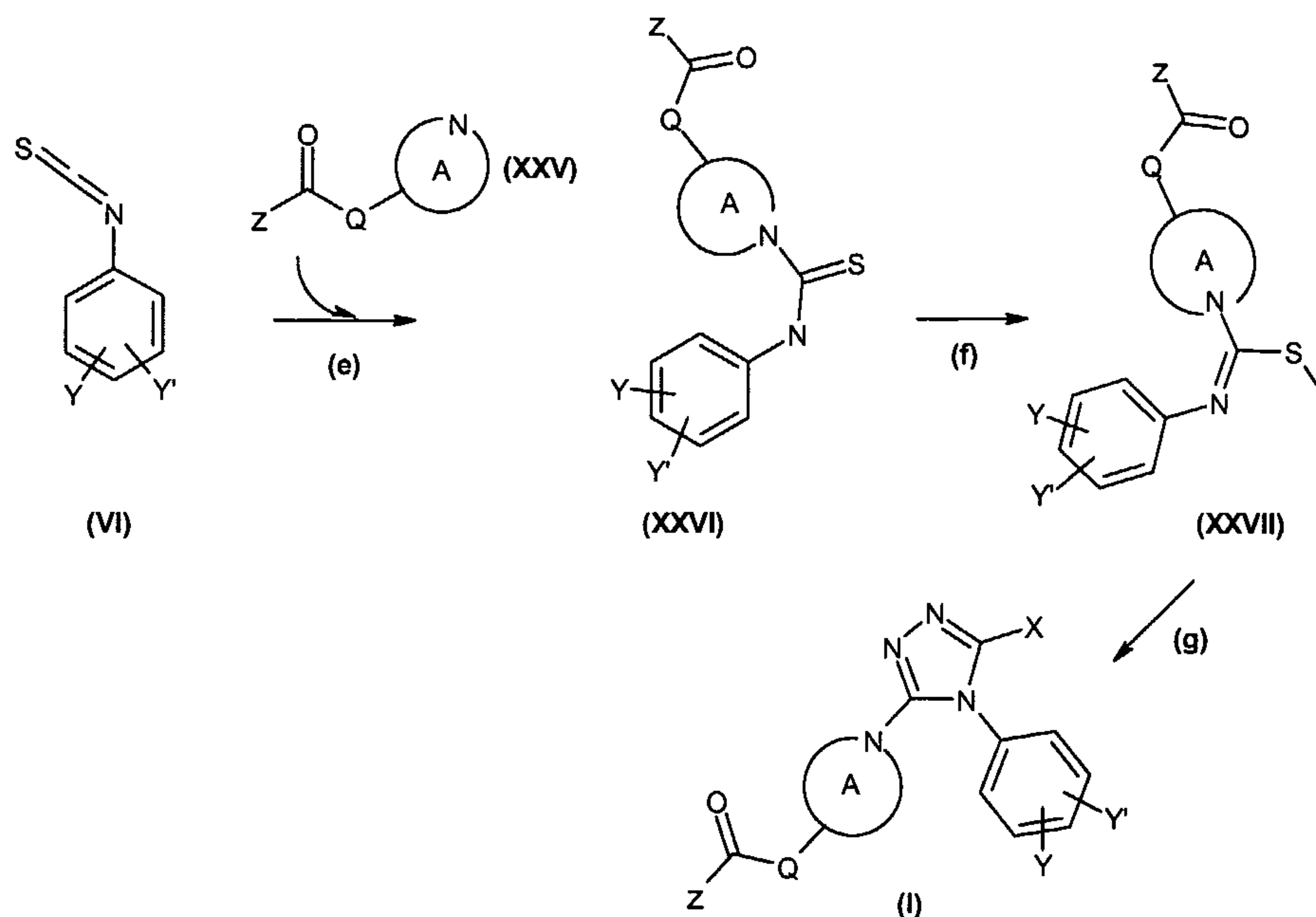
Scheme 9
