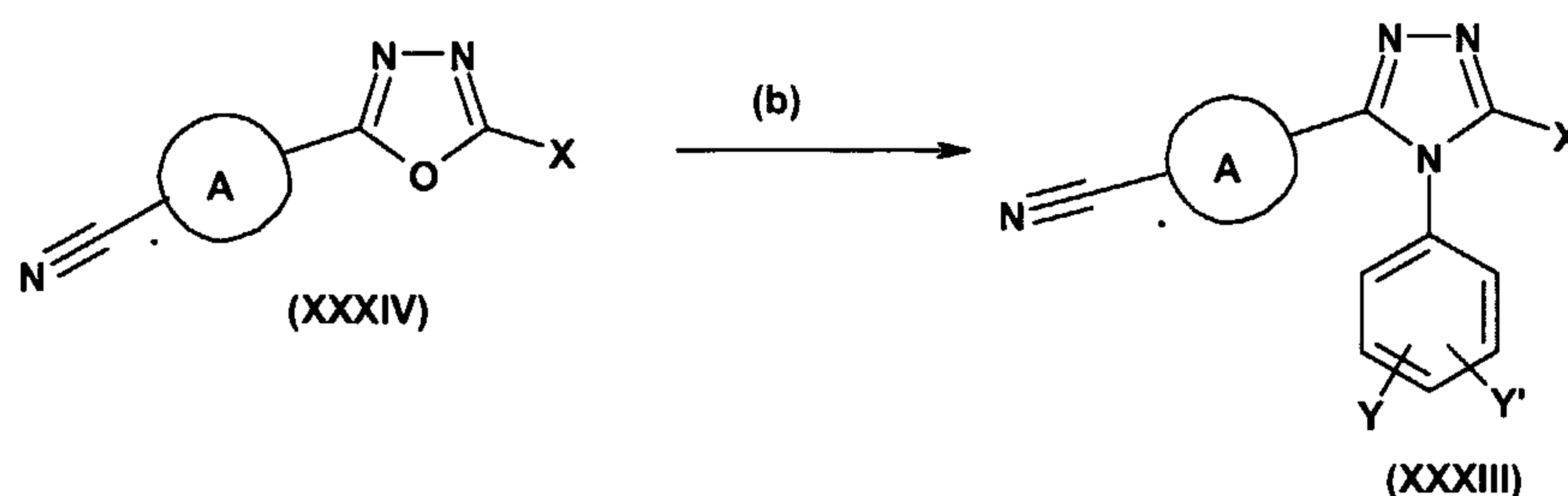
Scheme 11
