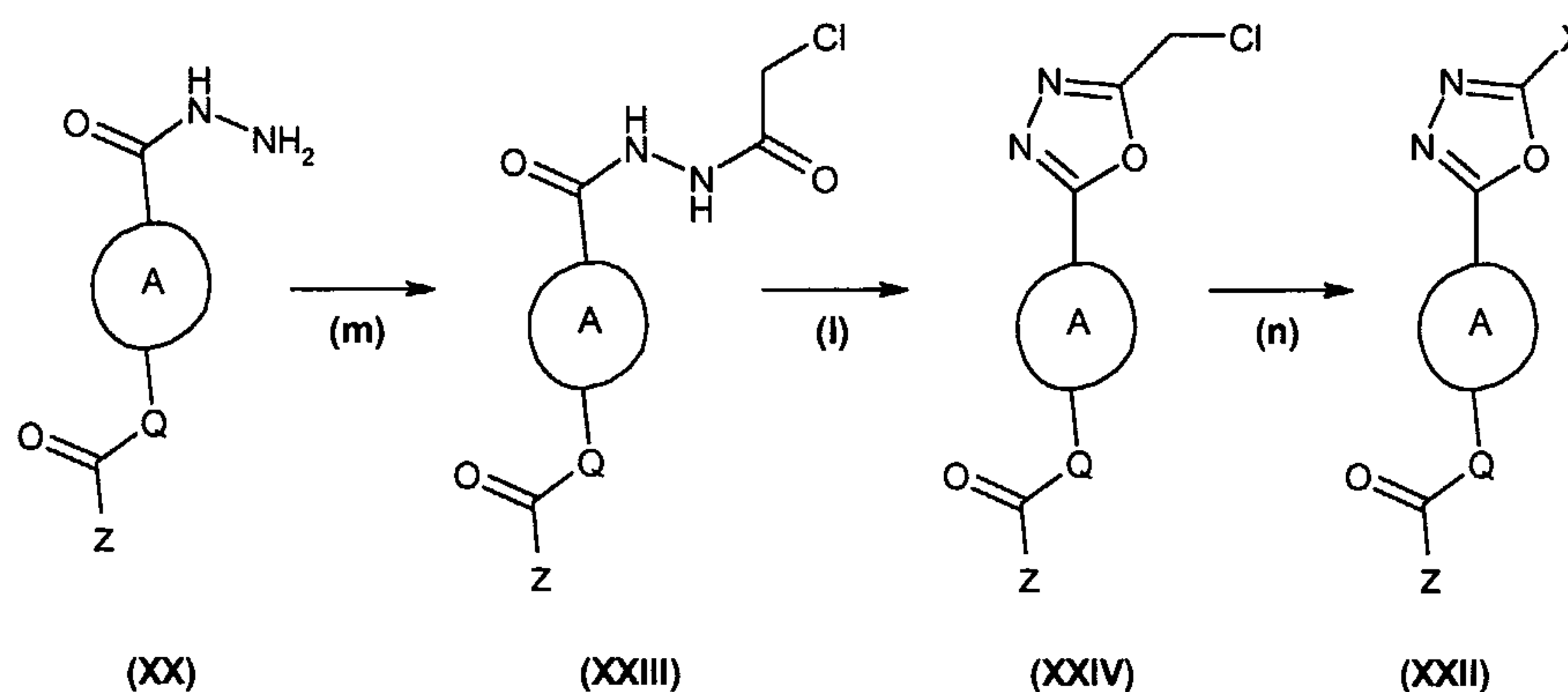
Scheme 8
