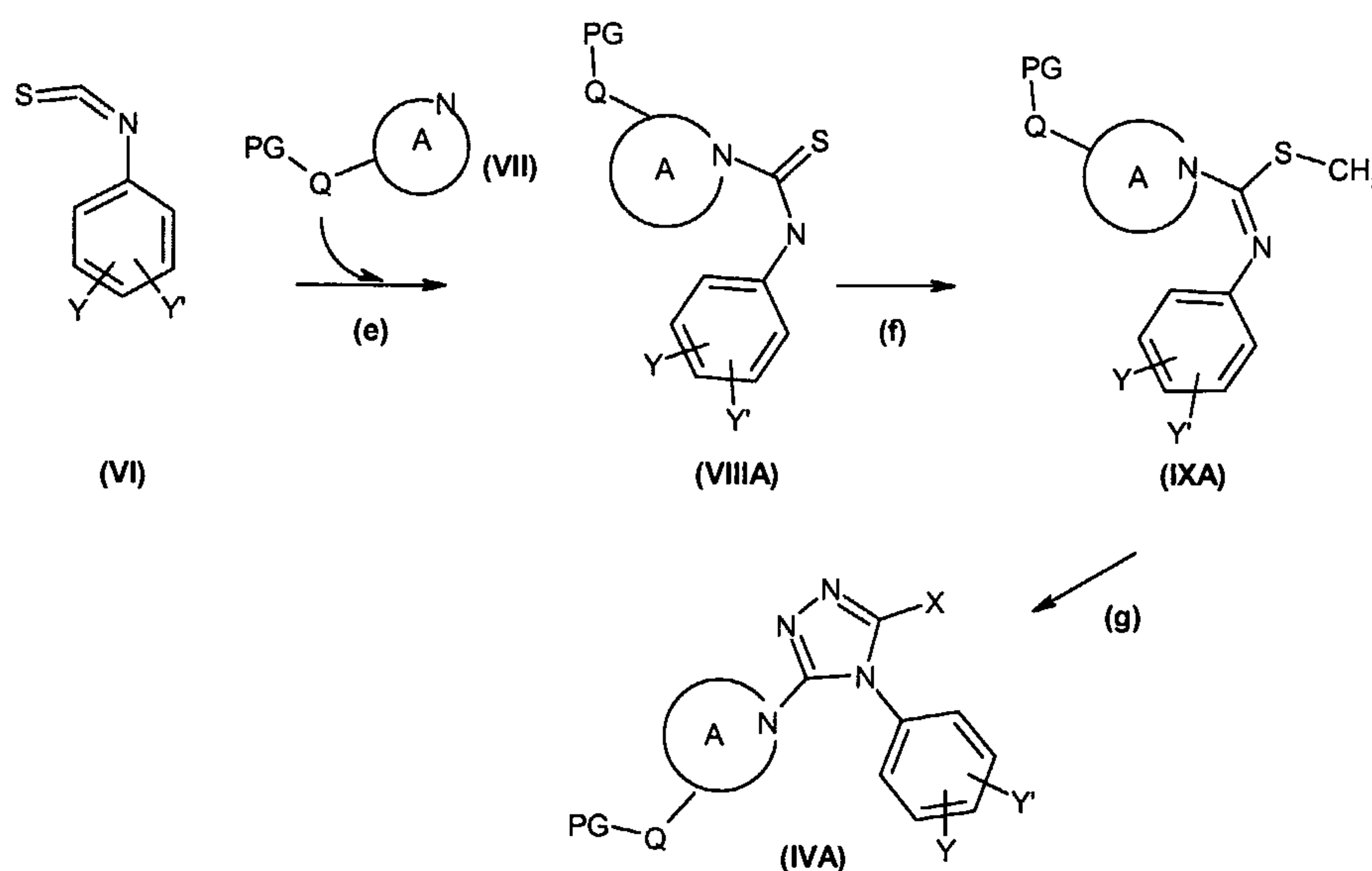
Scheme 2.
