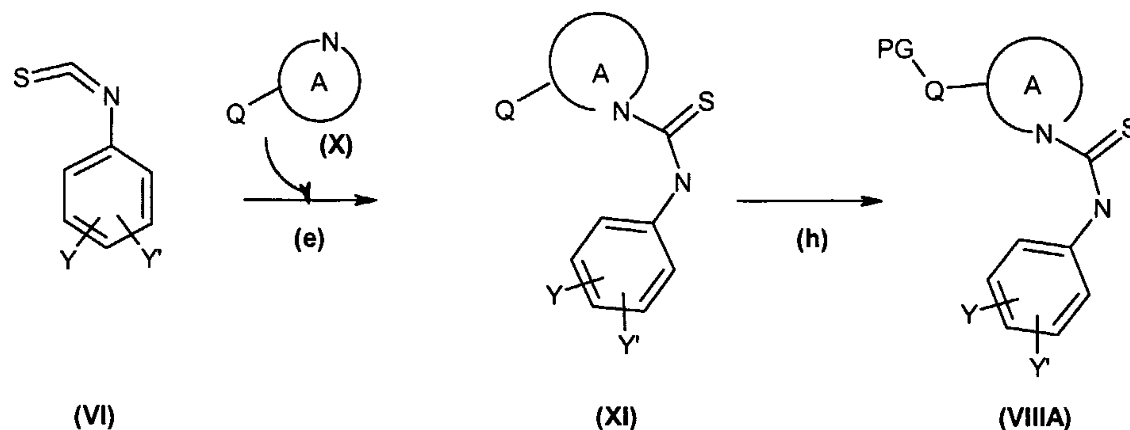
Scheme 3.
