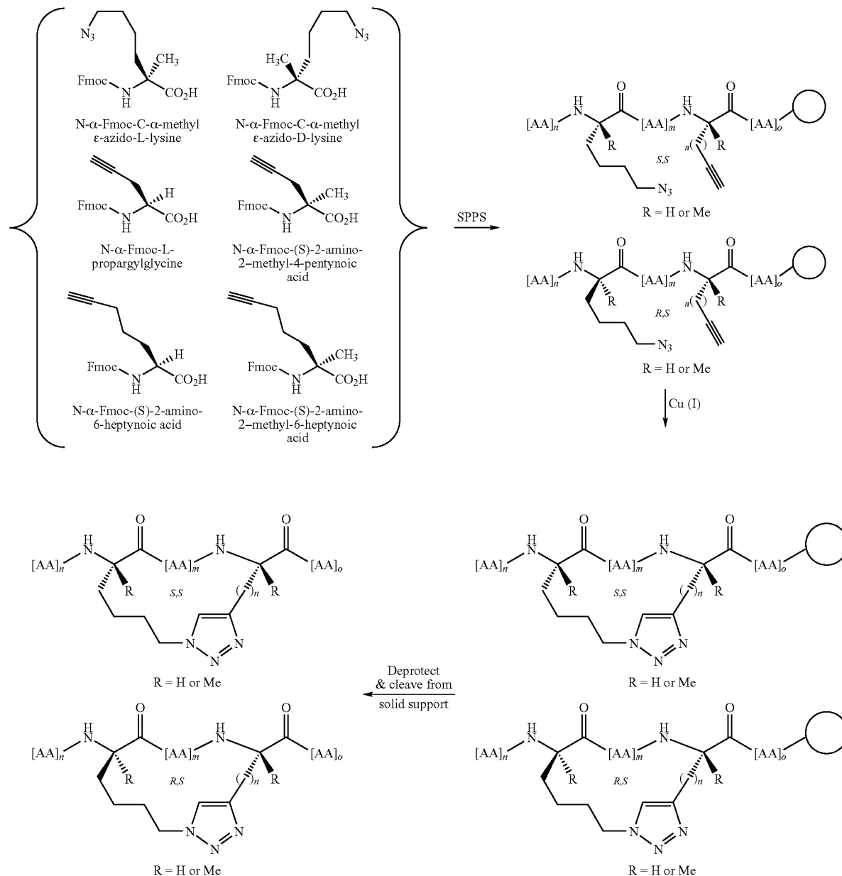
Synthetic Scheme 3:
