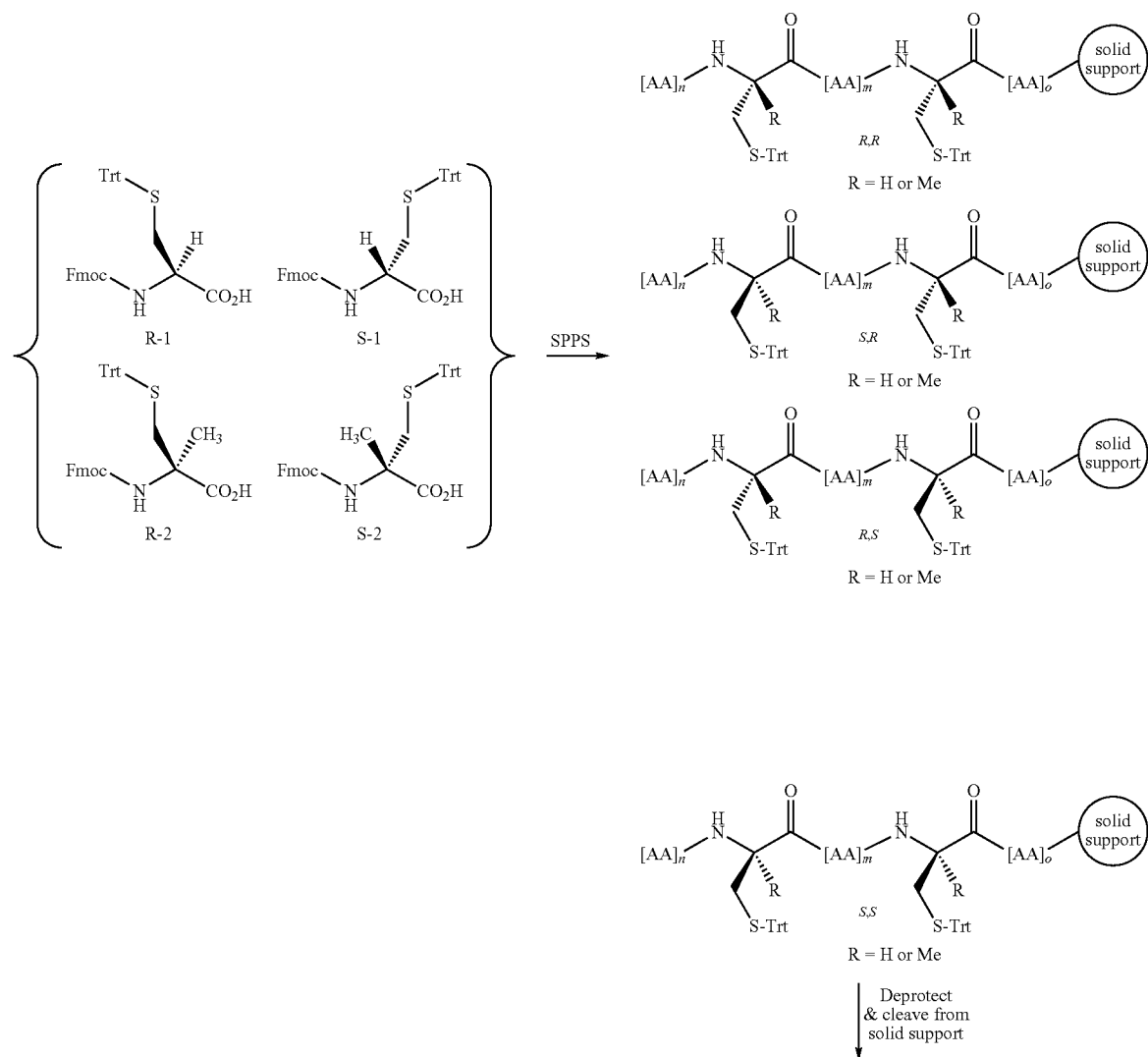
Synthetic Scheme 6:
