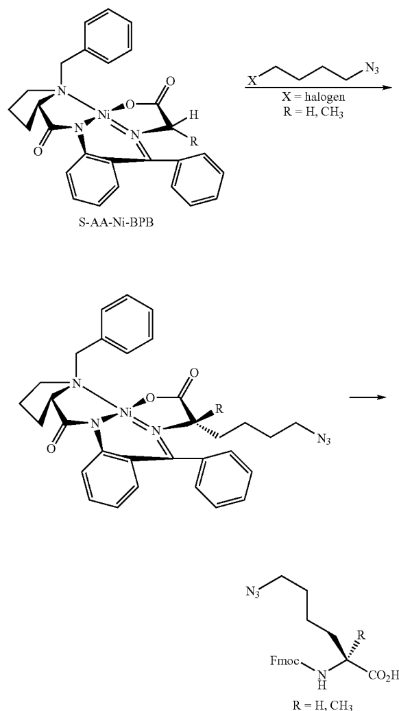
Synthetic Scheme 1:
