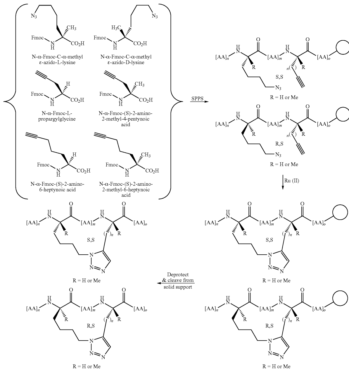
Synthetic Scheme 5:
