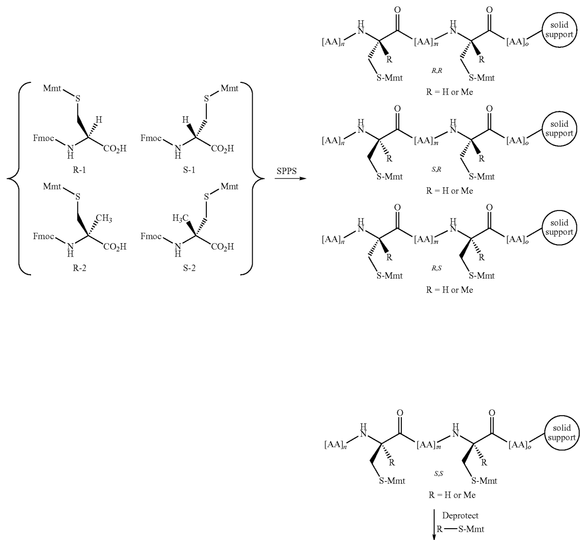
Synthetic Scheme 7:
