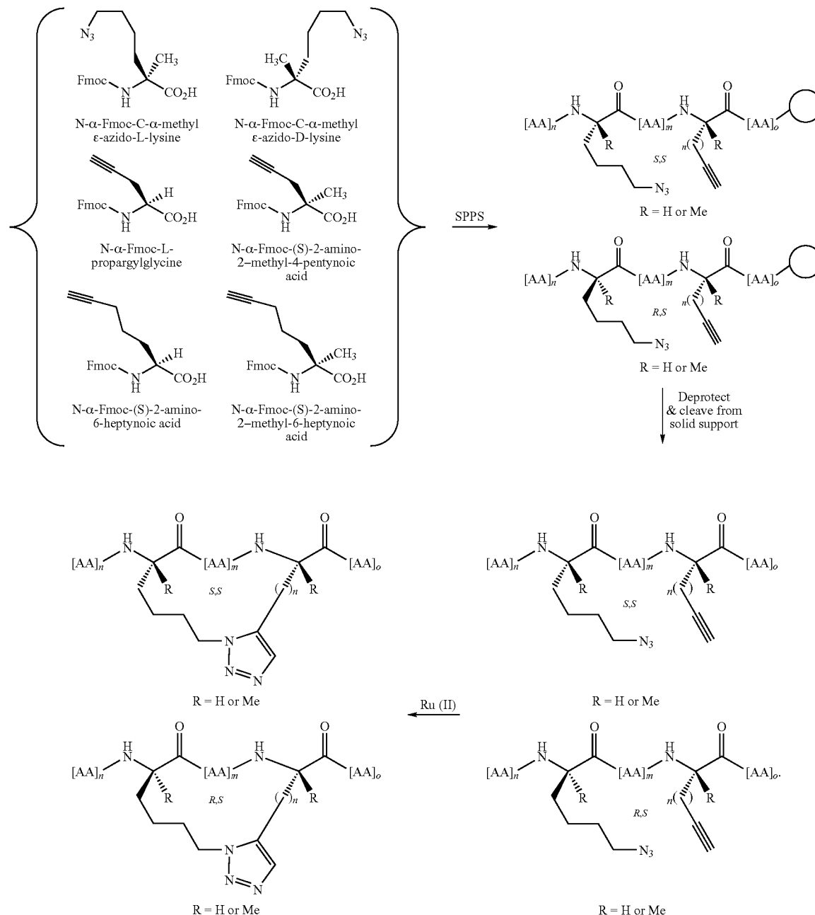
Synthetic Scheme 4:
