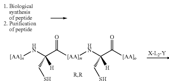
Synthetic Scheme 9:
