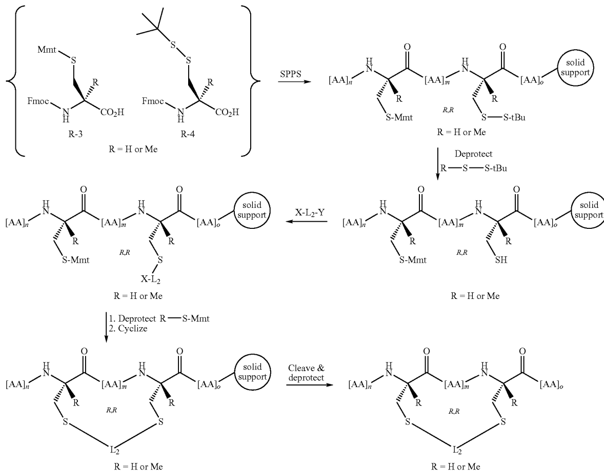
Synthetic Scheme 8:
