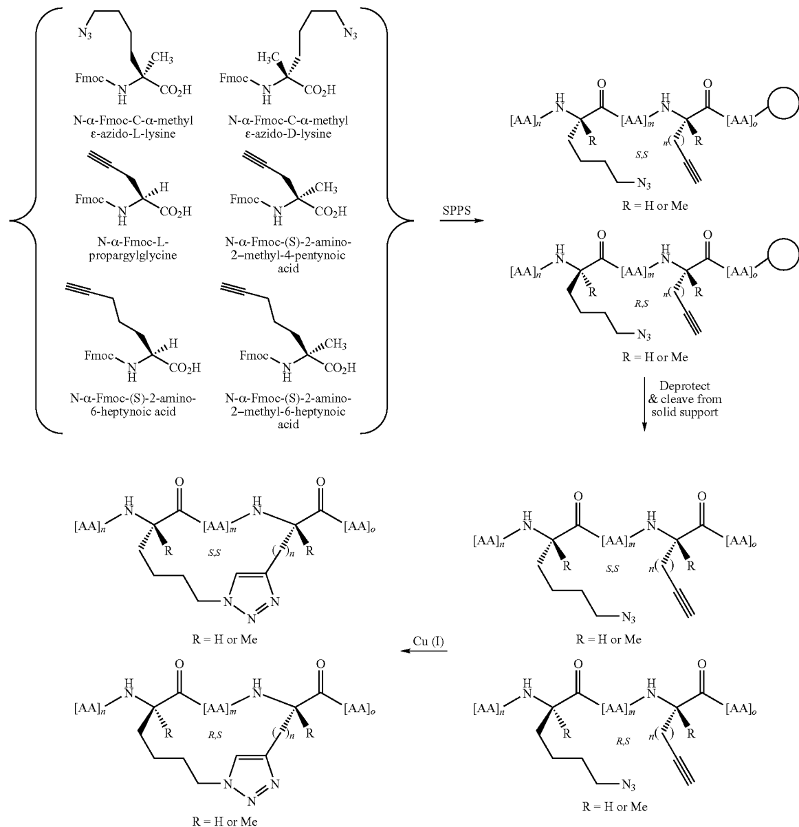
Synthetic Scheme 2:
