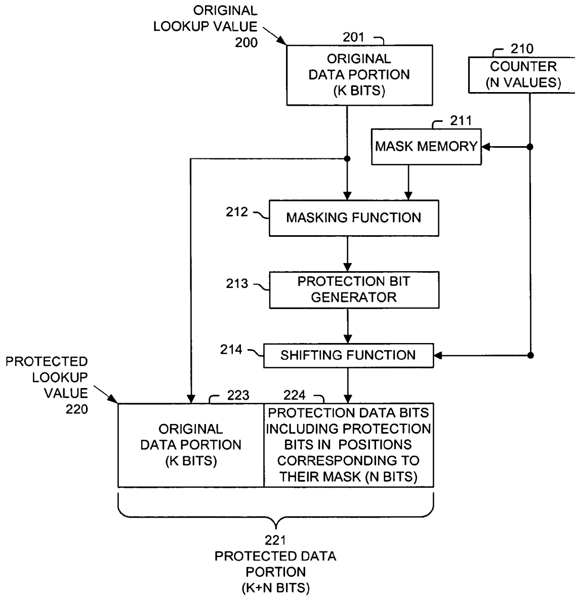
GENERATING A PROTECTED LOOKUP VALUE FIGURE 2A
