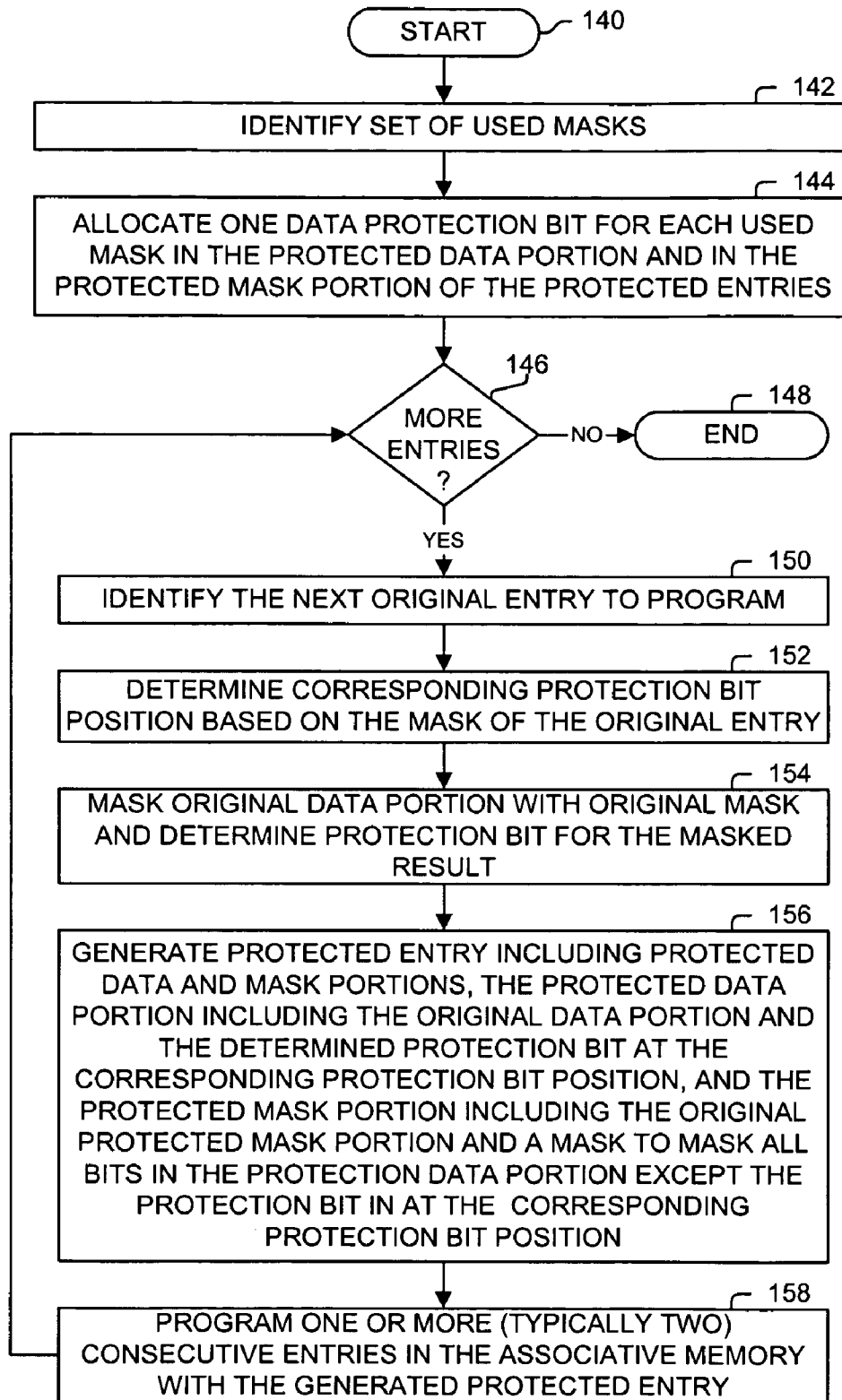
GENERATING PROTECTION ENTRIES FIGURE 1B
