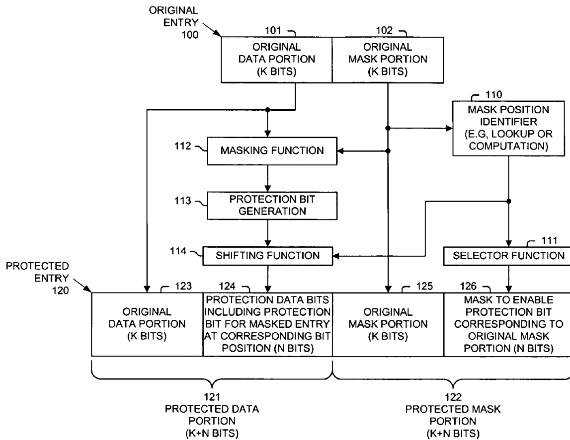
GENERATING PROTECTION ENTRIES FIGURE 1A
