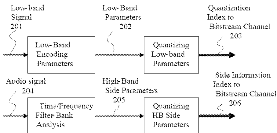
Encoder with SBR Side Information
