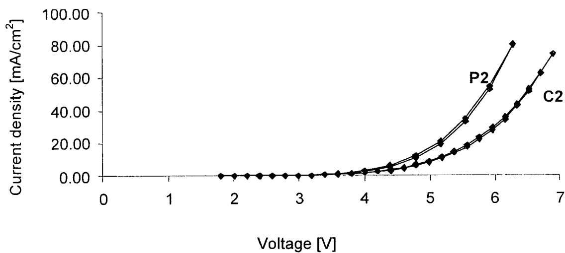
Current density/voltage curve for polymer P2 according to the invention and comparative polymer C2 .
