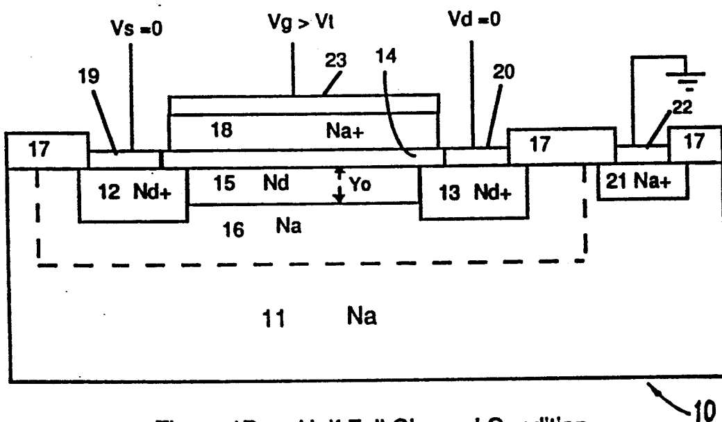
Figure 1B Half Full Channel Condition
