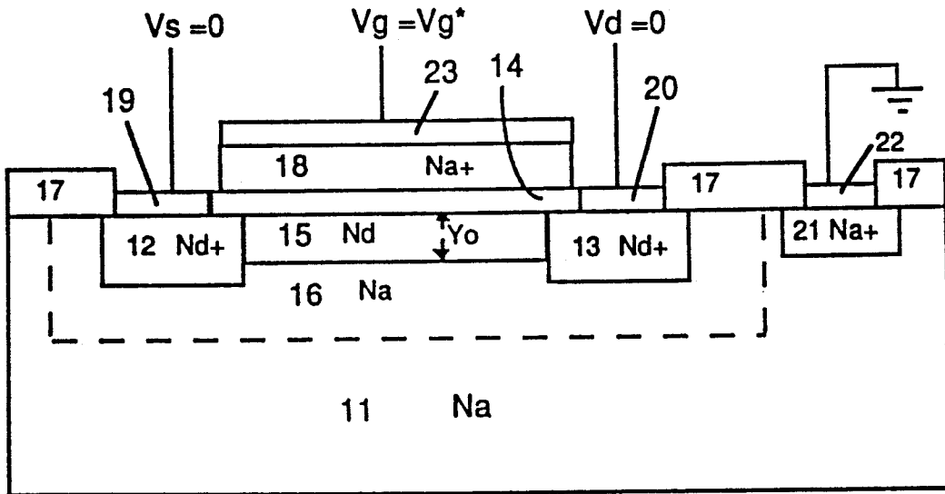
Figure 1C Full Channel Condition
