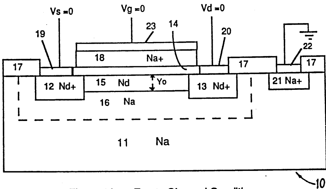
Figure 1A Empty Channel Condition
