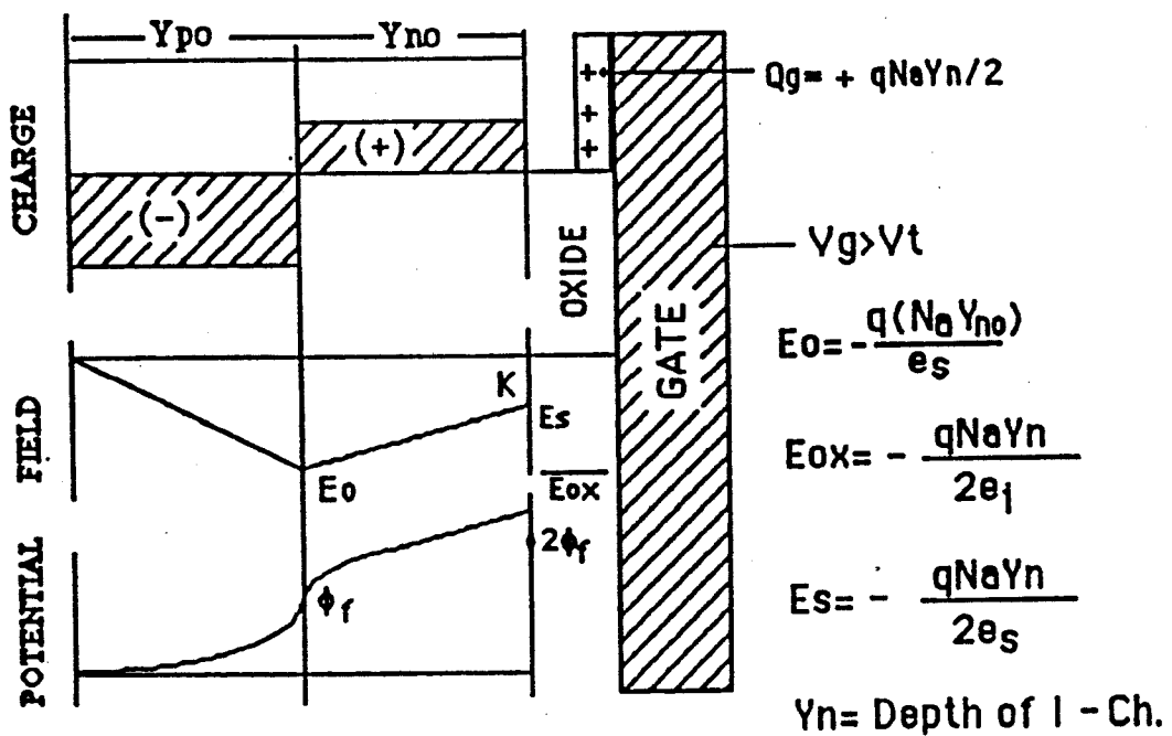
Figure 2-B HALF FULL CHANNEL
