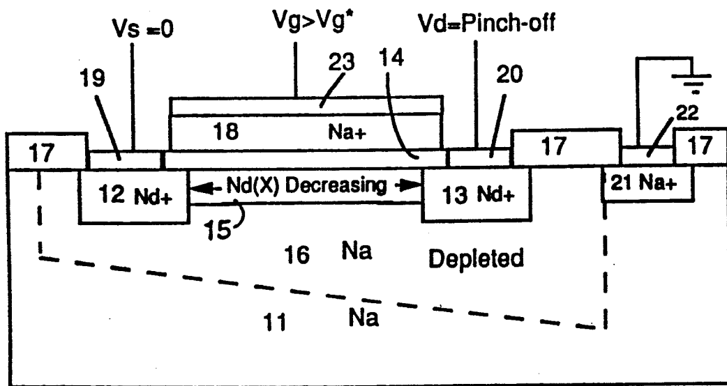
Figure 1D Fermi-FET at Pinch-off
