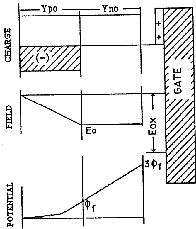
FIG.2-C Full Channel Condition
