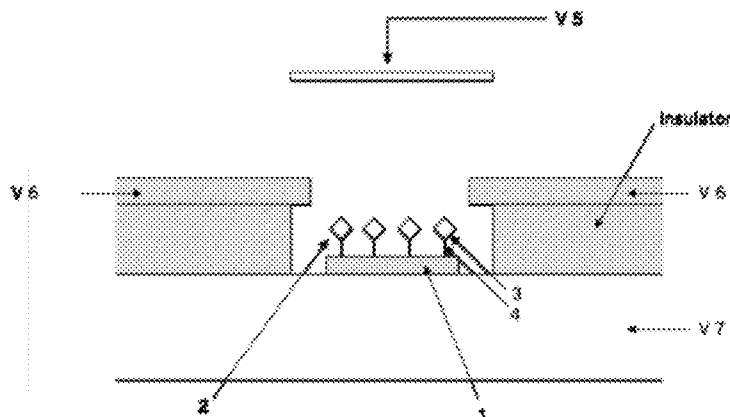
Three Terminal Field Emission Device
