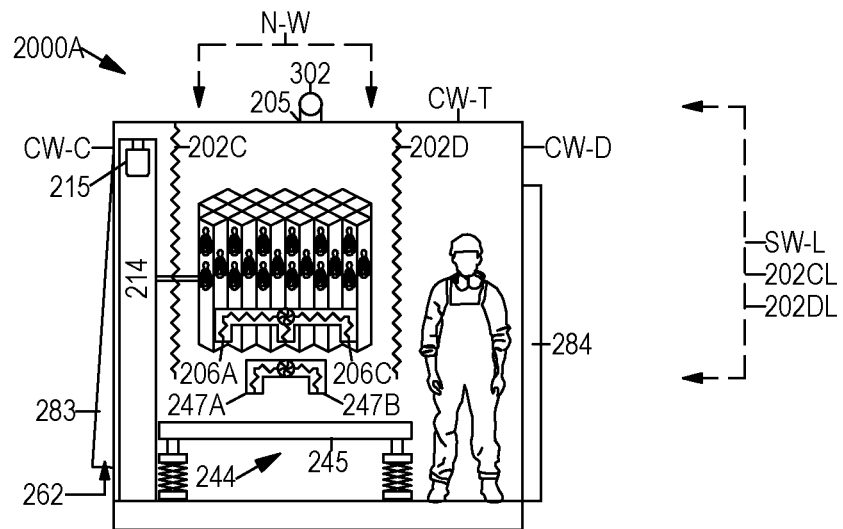
FIGURE 29 INSECT FEEDING MODULE, SIDE VIEW
