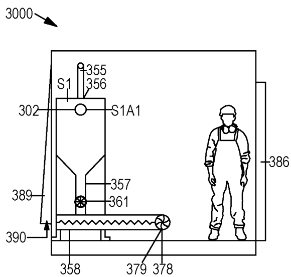
FIGURE 32 INSECT EVACUATION MODULE, SIDE VIEW
