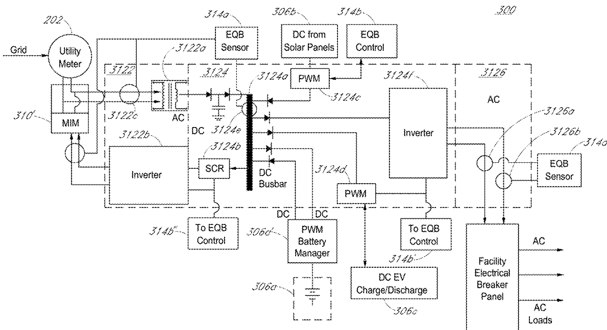
Expanded Non-Limiting View of Dynamic f_0 Power Electronics Module
