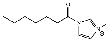
1-methyl-3-(1-oxoheptyl)-1H-imidazolium
