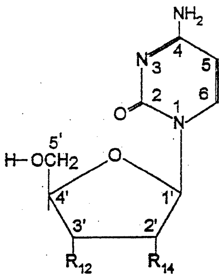
Cytidine
