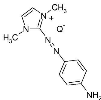
Basic Orange 31
