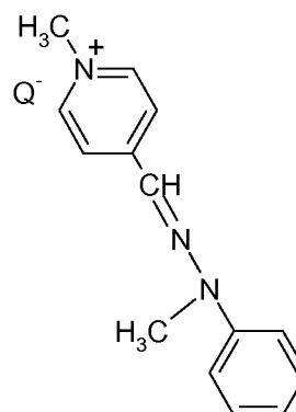
Basic Yellow 87
