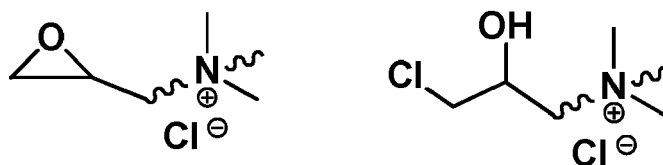
quaternized epoxy
