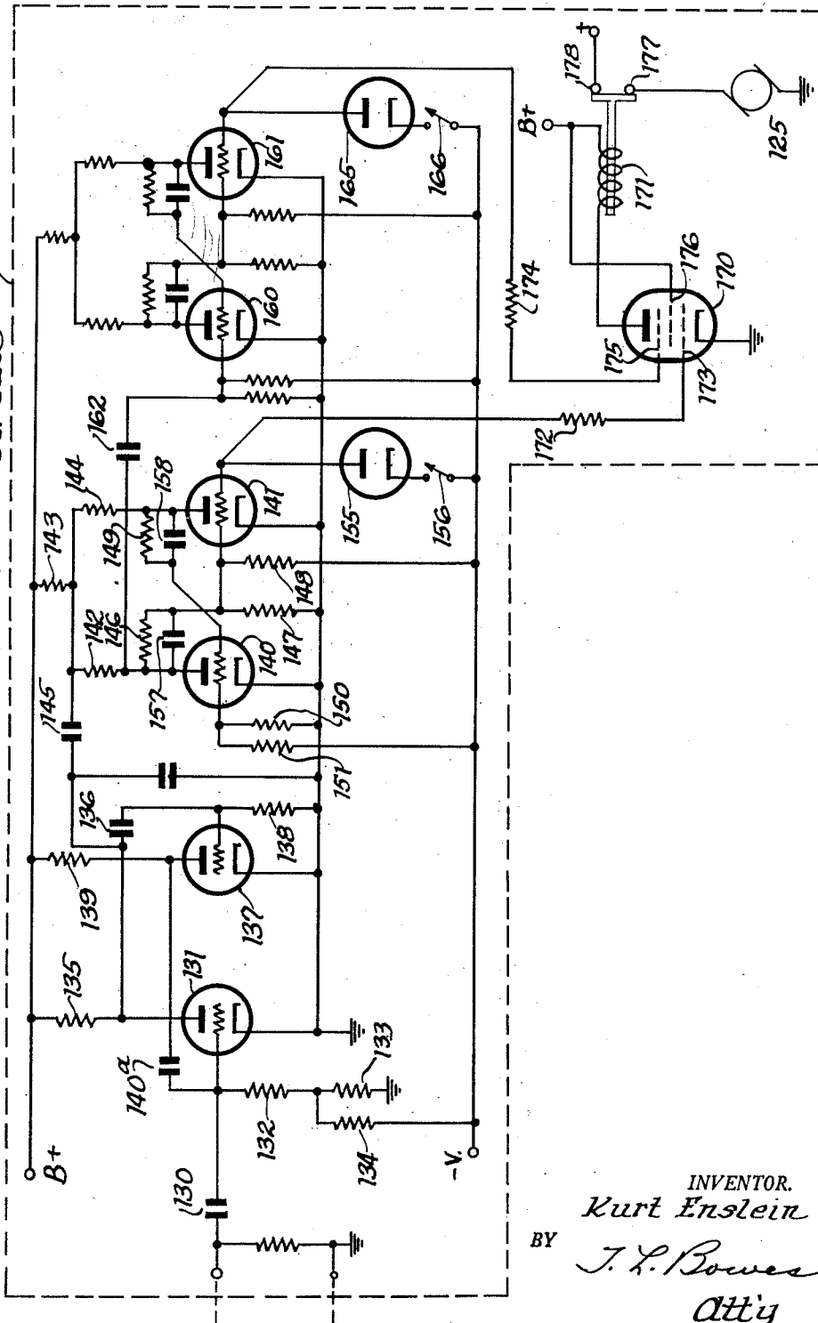
Fig. 10 Pulse Counter Circuit 38
