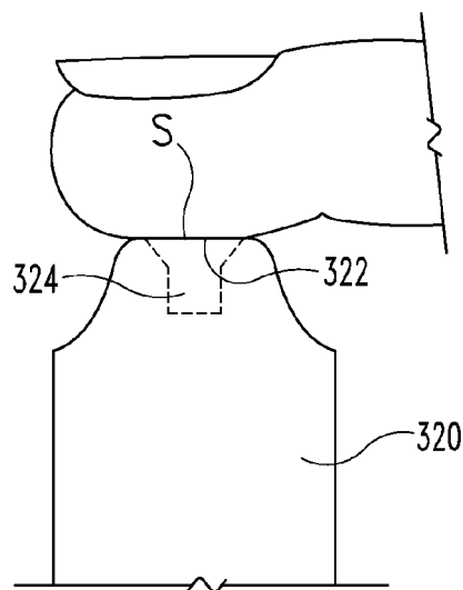
Fig. 6 (PRIOR ART)
