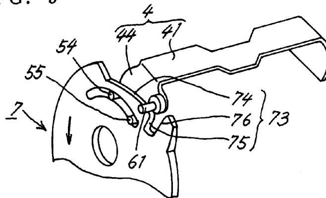
FIG. 9 Ink-sheet feed mode
