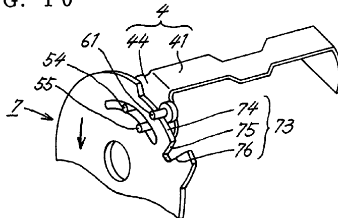
FIG. 10 Sheet ejecting mode
