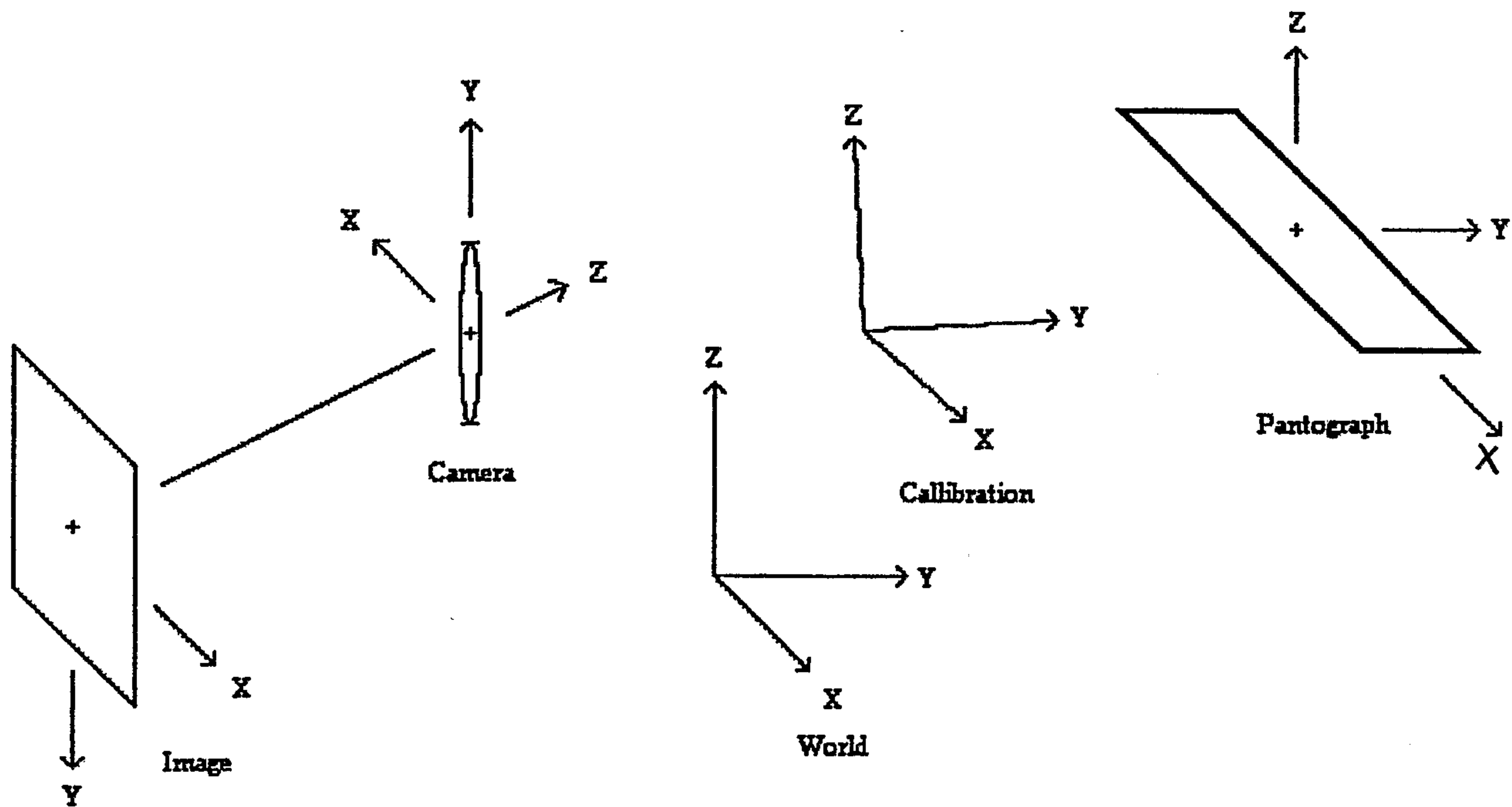
Figure 12: Reference Frames
