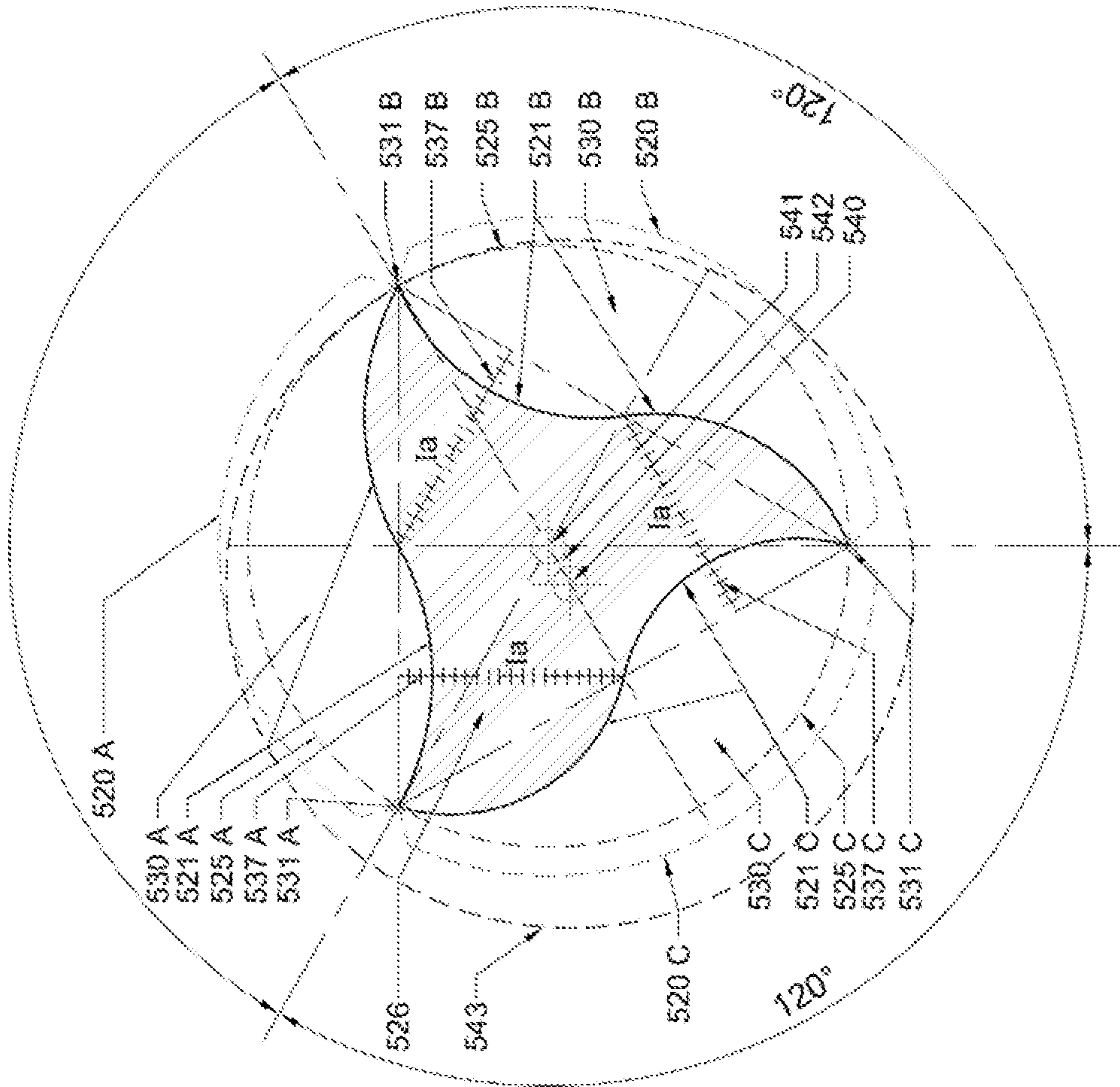
Section A-A 120°
