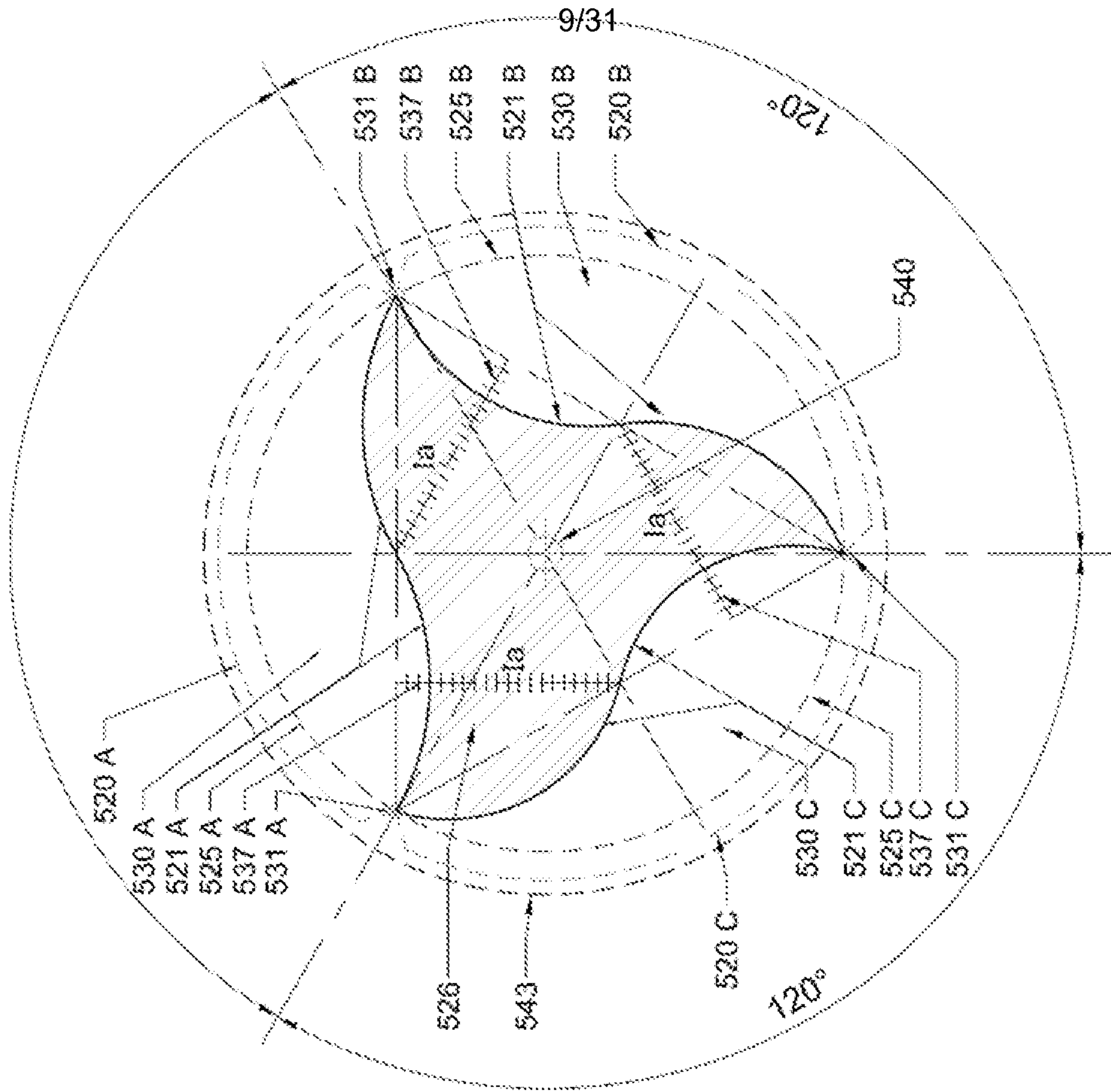
Section B-B 120°
