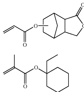
[Chemical formula 55]
