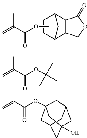
[Chemical formula 54]
