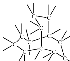
[Chemical formula 40]
