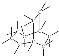
[Chemical formula 39]
