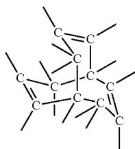
[Chemical formula 39]
