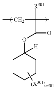
[Chemical formula 30]
