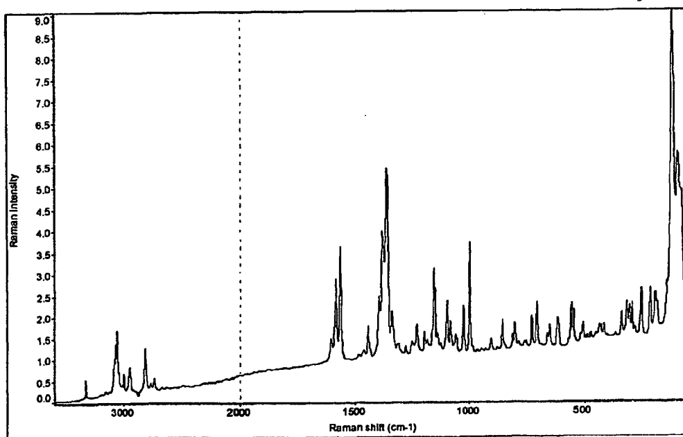
Figure 2 Raman spectrum of 3-phenylsulfonyl-8-piperazin-1-yl-quinoline (Form I)
