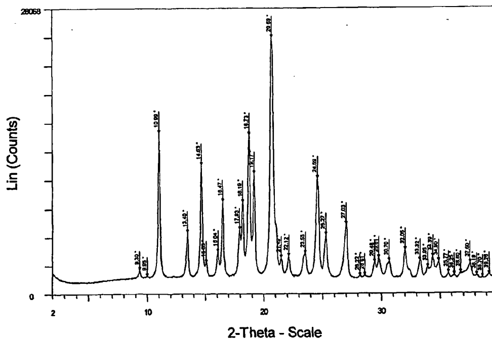
Figure 6 X-ray powder diffraction pattern for 3-phenylsulfonyl-8-piperazin-1-yl-quinoline (Form II)
