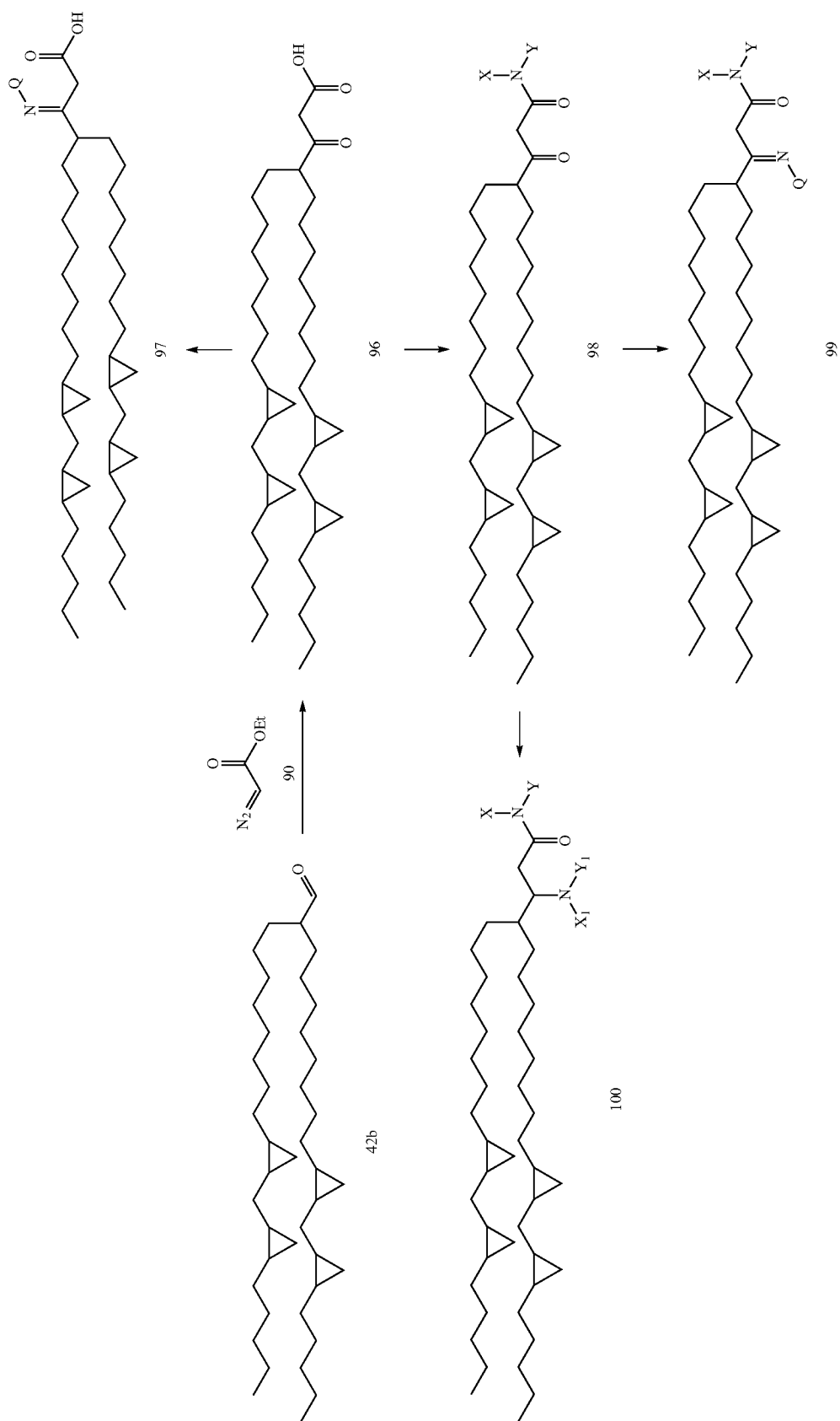
Scheme 7b ( \beta -Keto Acid Analogs)
