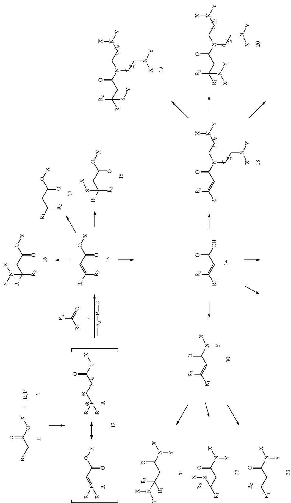
Scheme 2a (Wittig Reaction Followed By 1,4-Michael Addition)
