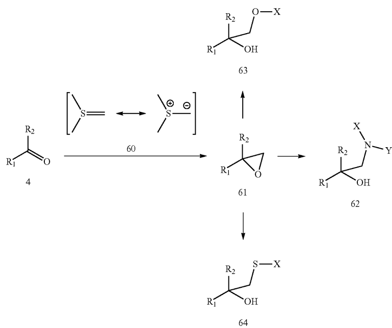
Scheme 4 (Sulfur Ylides)
