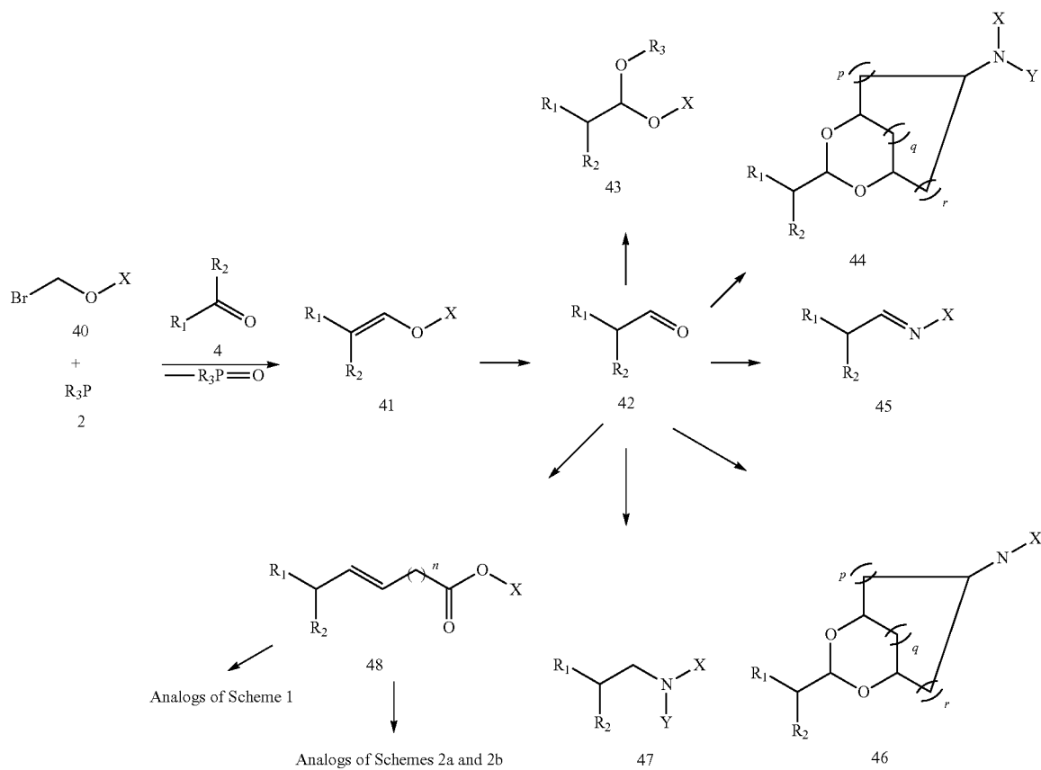
Scheme 3 (Wittig Reaction Followed By Michael Addition)
