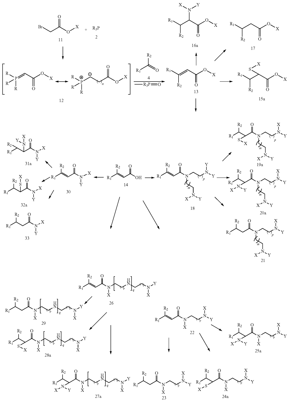
Scheme 2b (Wittig Reaction Followed By 1,2-Michael Addition)
