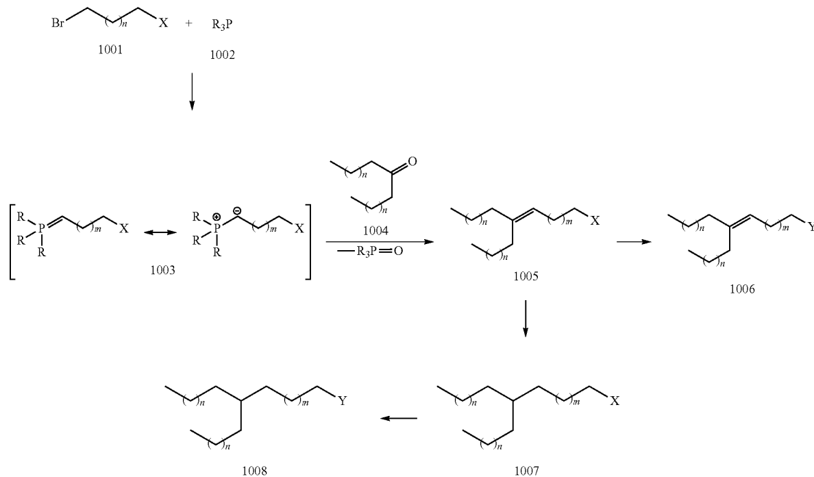
Scheme 8 (Wittig Reaction)
