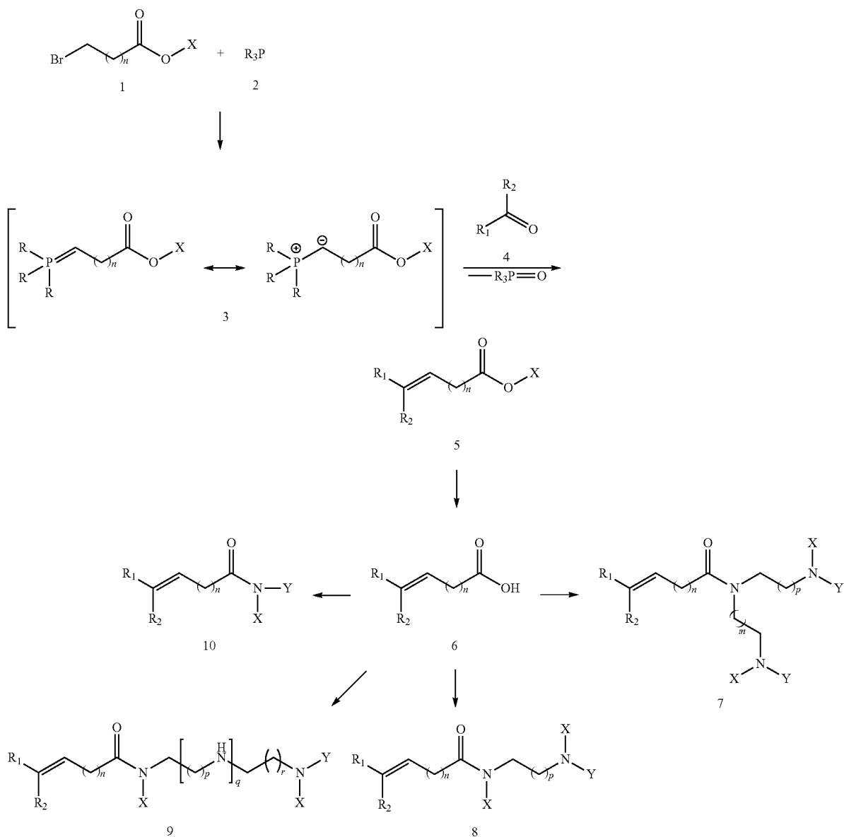
Scheme 1 (Wittig Reaction)
