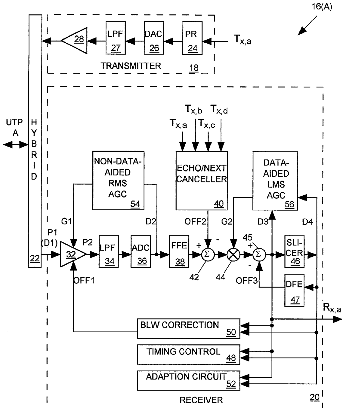
FIG. 2 (PRIOR ART)
