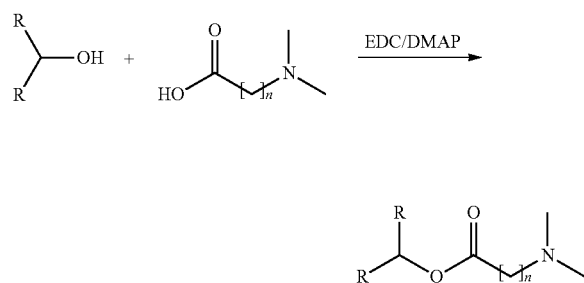
Scheme 1: M series (esters) synthesis
