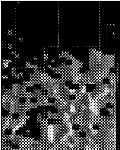
Y Direction Asymmetry in Terrain Height 10 03
