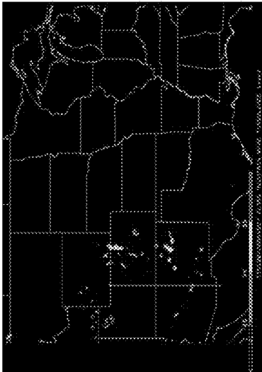
MWAVE grid output 8 01
